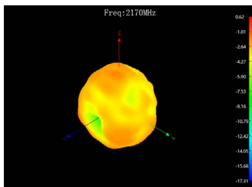
Div 3D pattern
