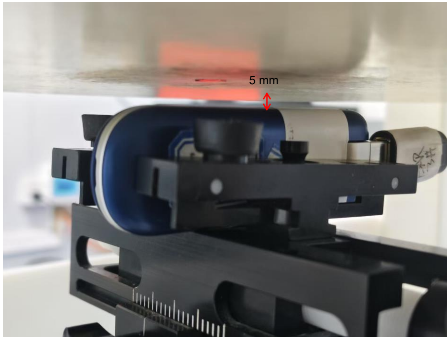
Horizontal-Front (5mm)
