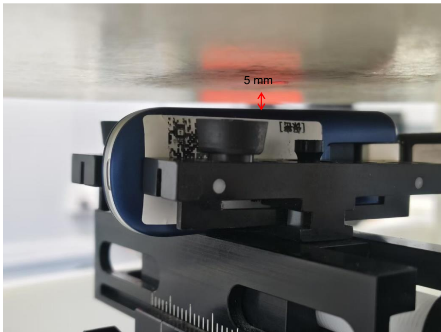
Horizontal-Back (5mm)
