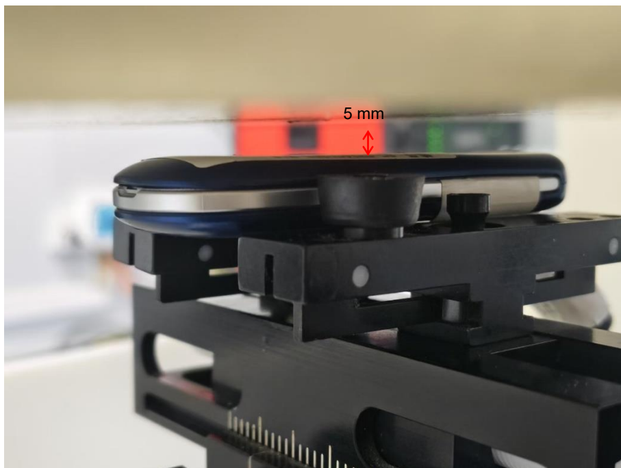
Horizontal-Down (5mm)
