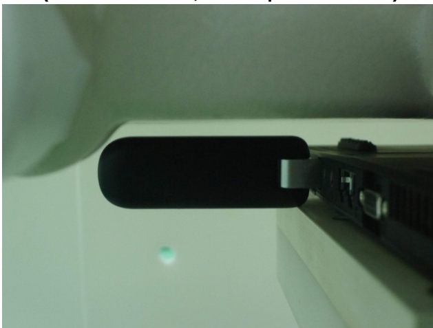
Direct Laptop Plug-in USB Configuration 4 (Vertical Back, Test Separation 5 mm)
