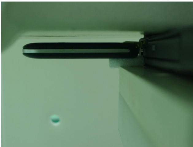
Direct Laptop Plug-in for USB Configuration 2 (Horizontal Down, Test Separation 5 mm)
