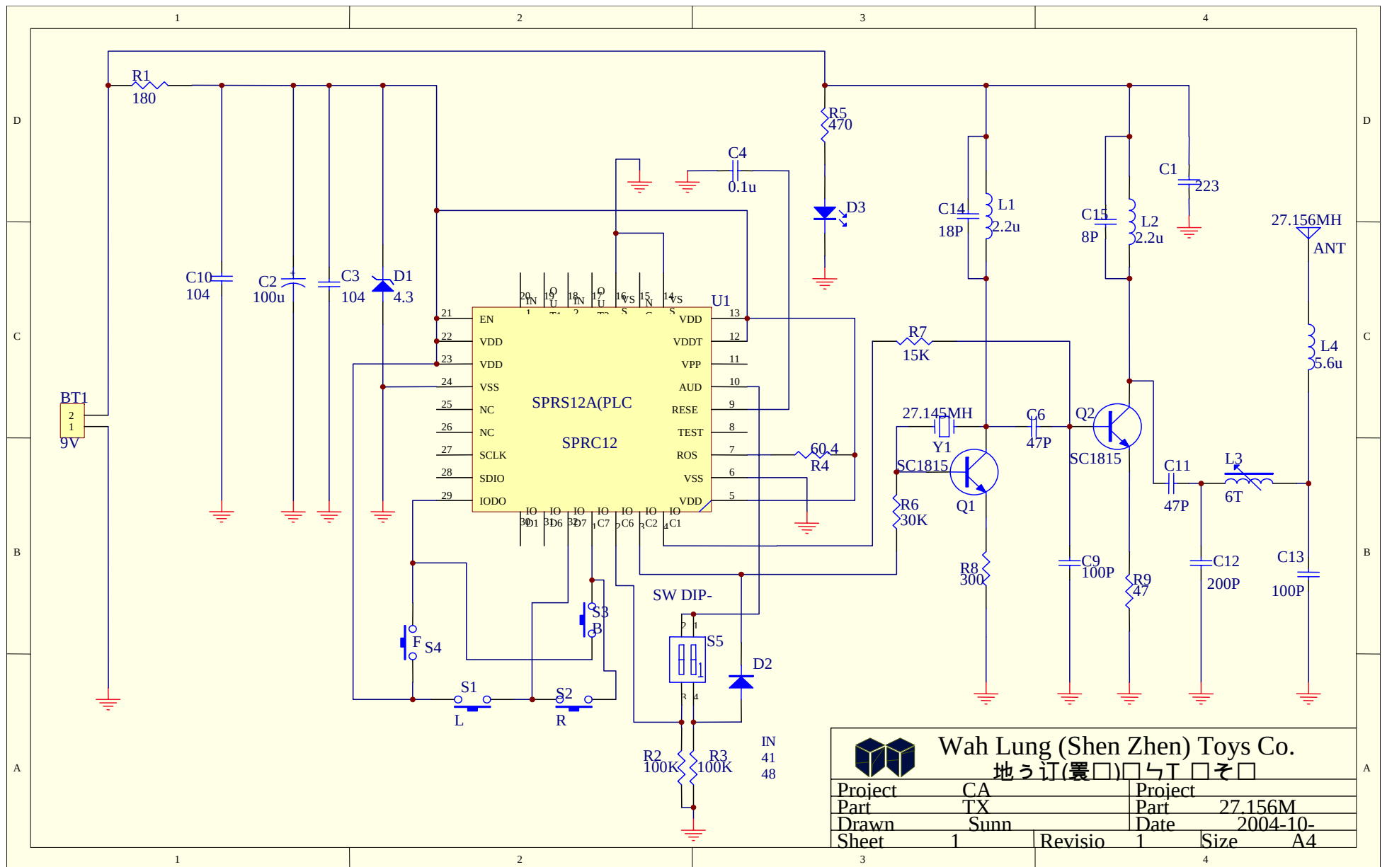
27.145MHZ TX Schematic
