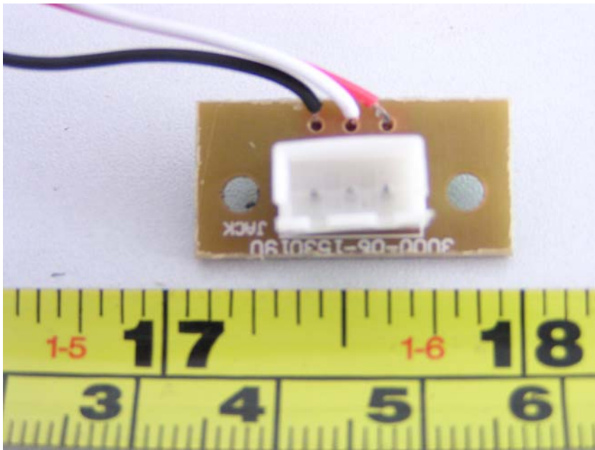
EUT – PCB1 Front View
