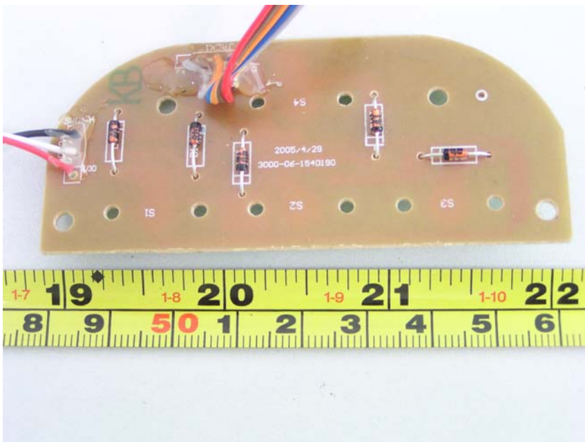
EUT – PCB3 Front View
