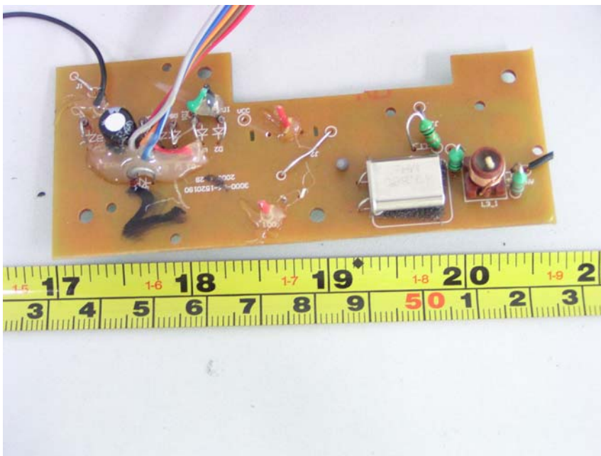
EUT – PCB2 Front View
