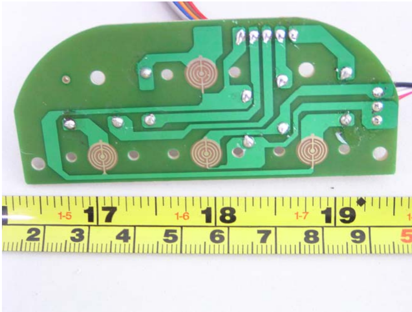
EUT – PCB3 Rear View
