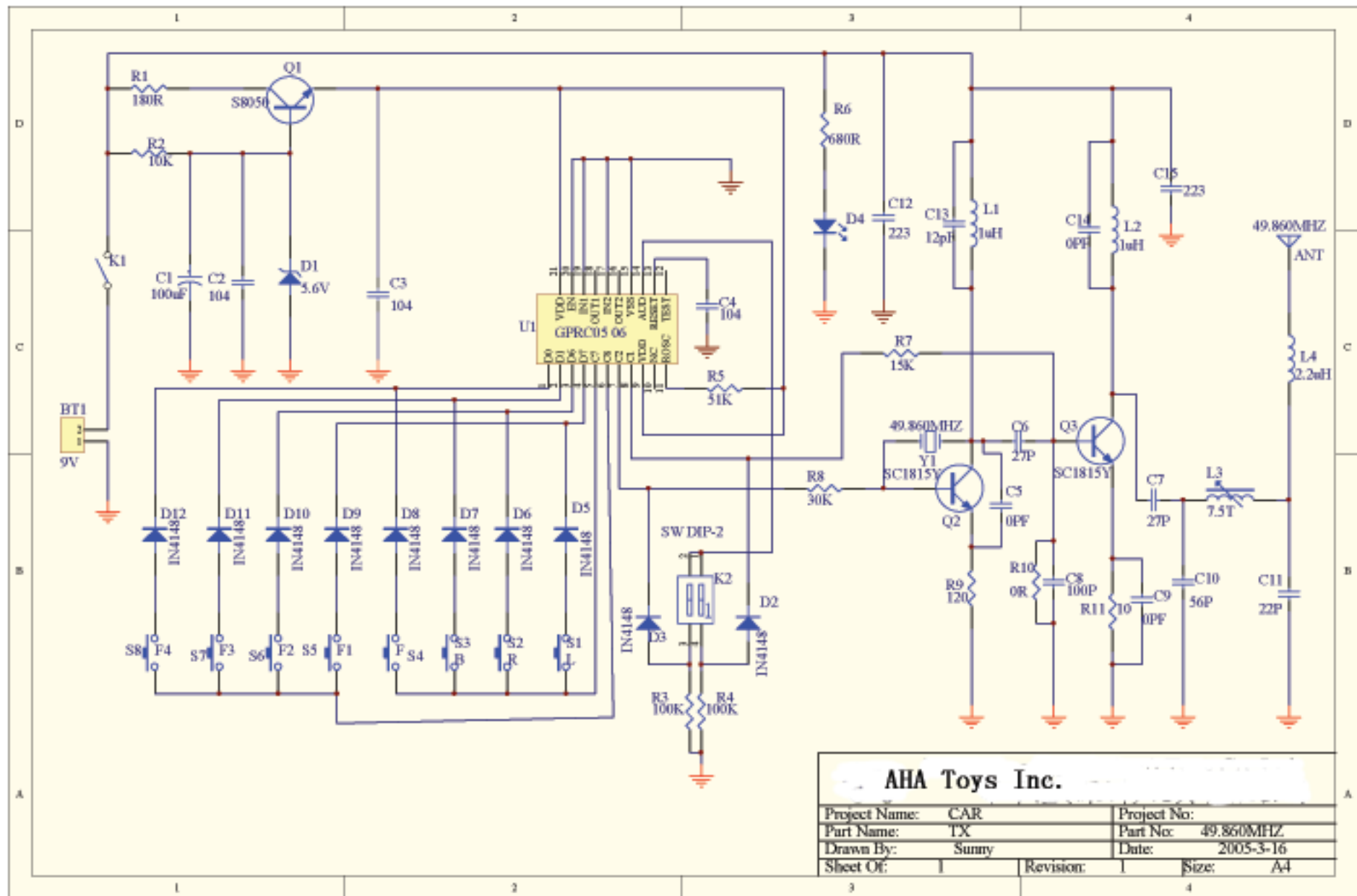
49.860MHZ TX CIRCUIT SCHEMATIC
