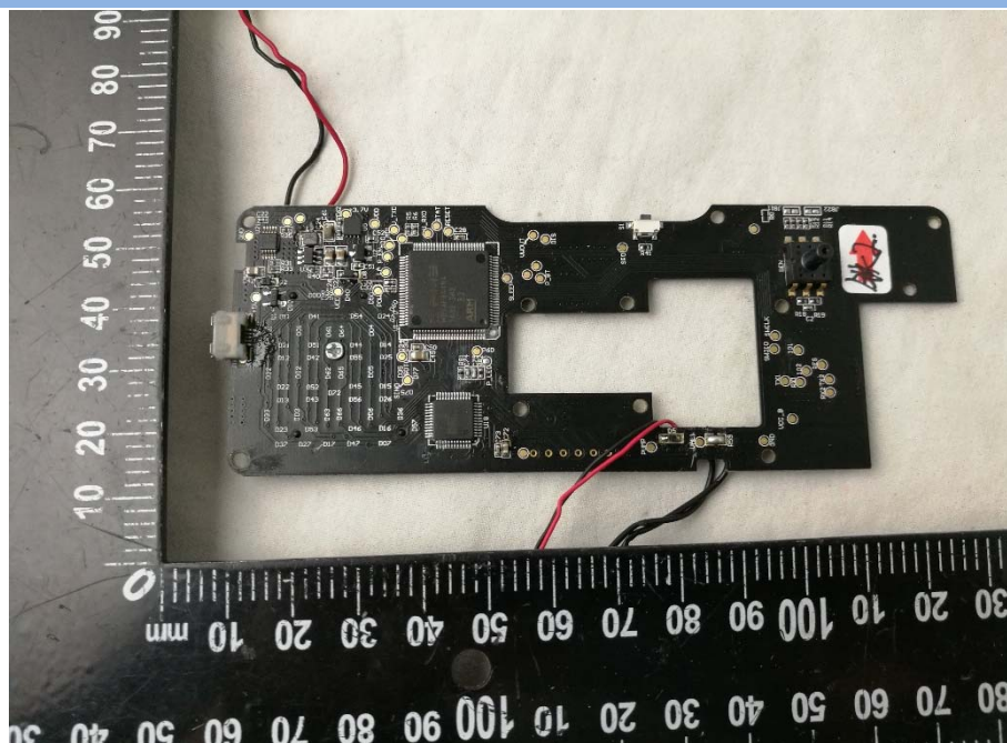
MAIN BOARD 1 BACK VIEW 1
