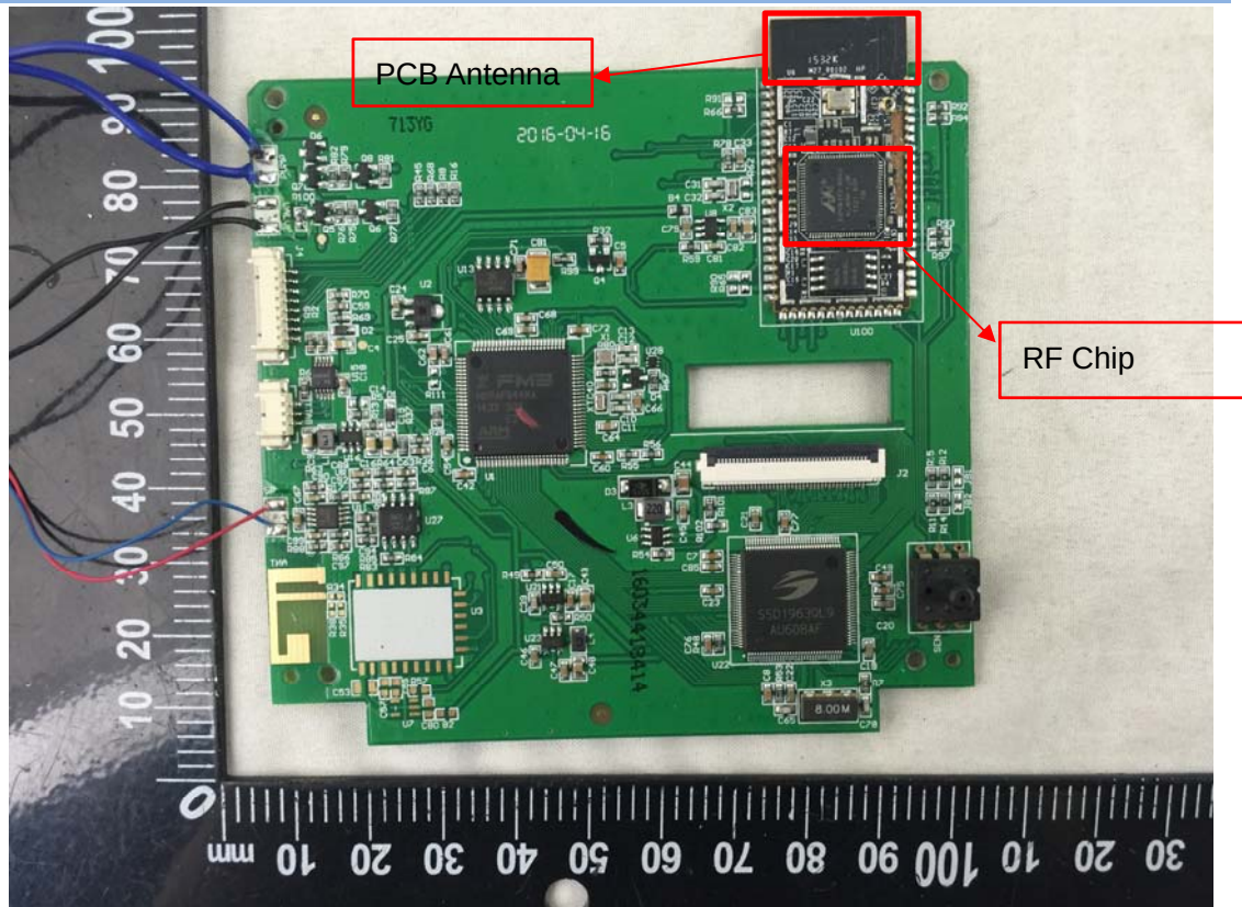
MAIN BOARD 1 FRONT VIEW
