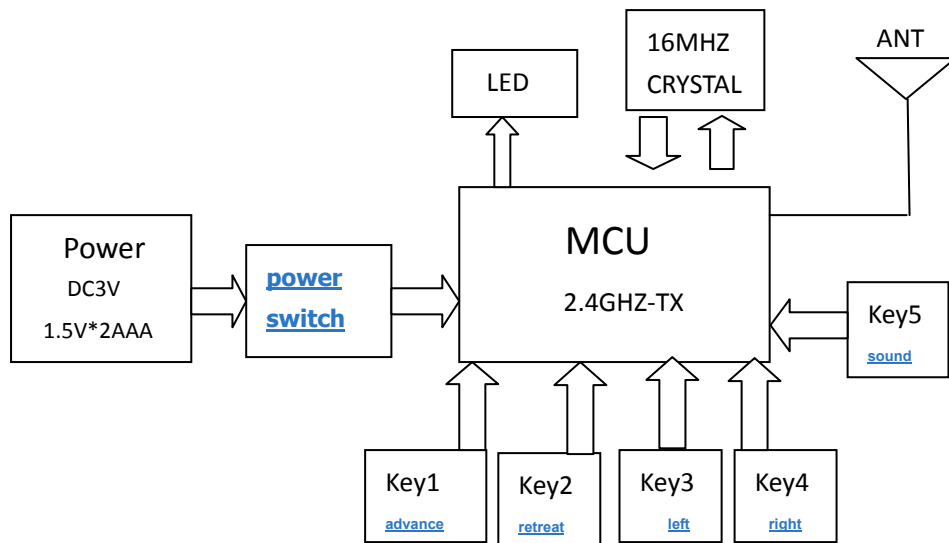
WH1330-WH1333TX ( block scheme )
