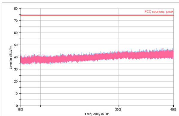
Figure 5. 18-40GHz Peak
