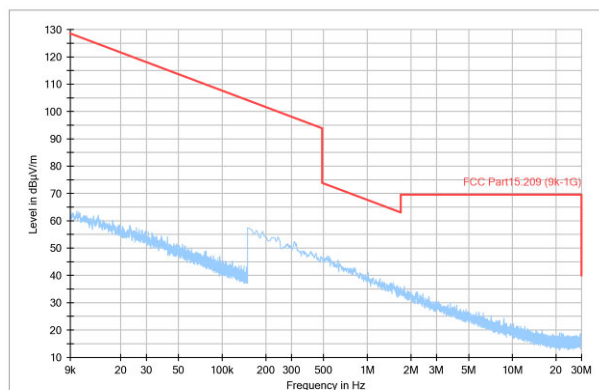
Figure 1. 9k-30MHz
