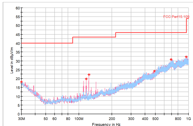
Figure 2. 30M-1GHz
