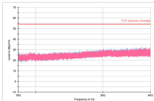
Figure 6. 18-40GHz Average
