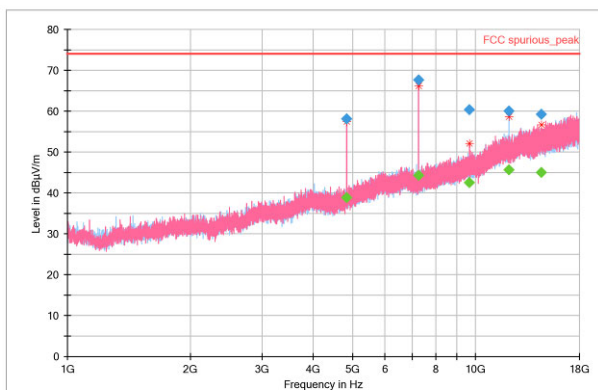
Figure 3. 1-18GHz Peak
