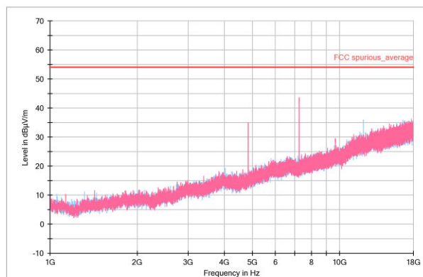
Figure 4. 1-18GHz Average
