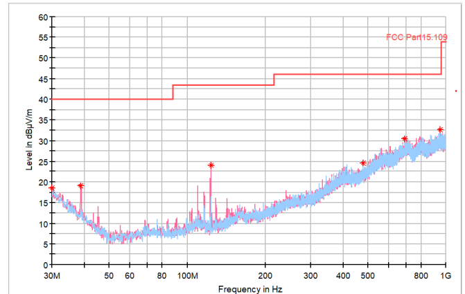
Figure 2. 30M-1GHz
