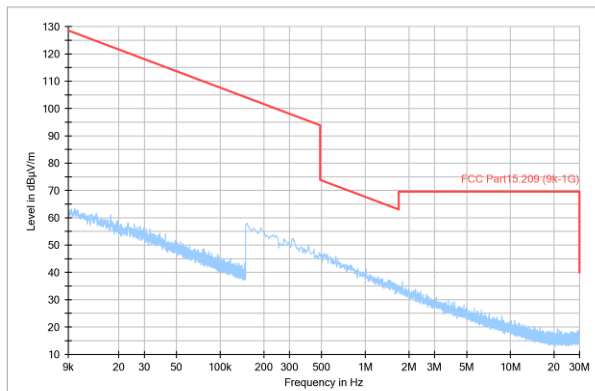
Figure 1. 9k-30MHz
