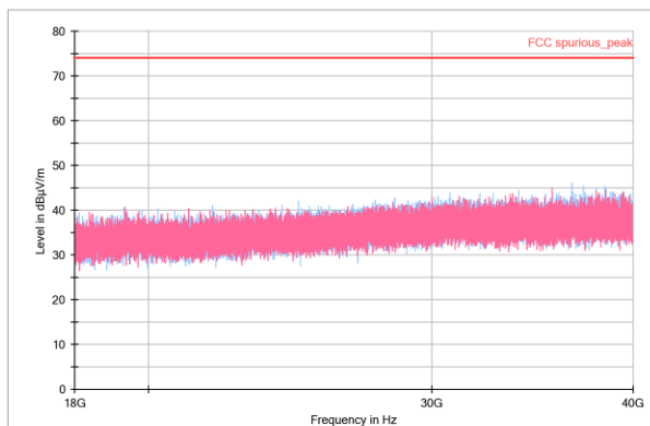
Figure 5. 18-40GHz Peak
