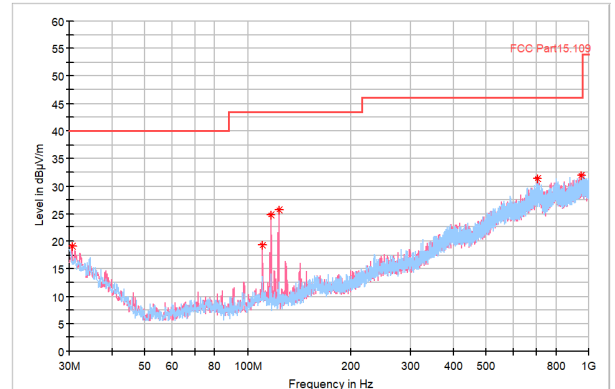
Figure 2. 30M-1GHz
