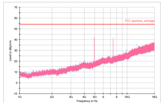
Figure 4. 1-18GHz Average
