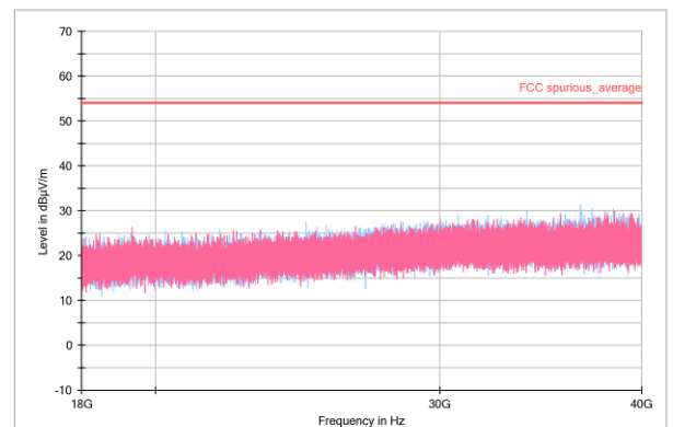
Figure 6. 18-40GHz Average
