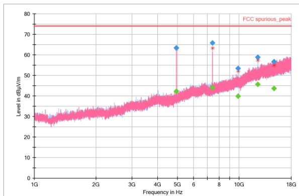
Figure 3. 1-18GHz Peak
