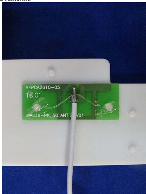
(34) EUT Photo-5GHz Antenna
