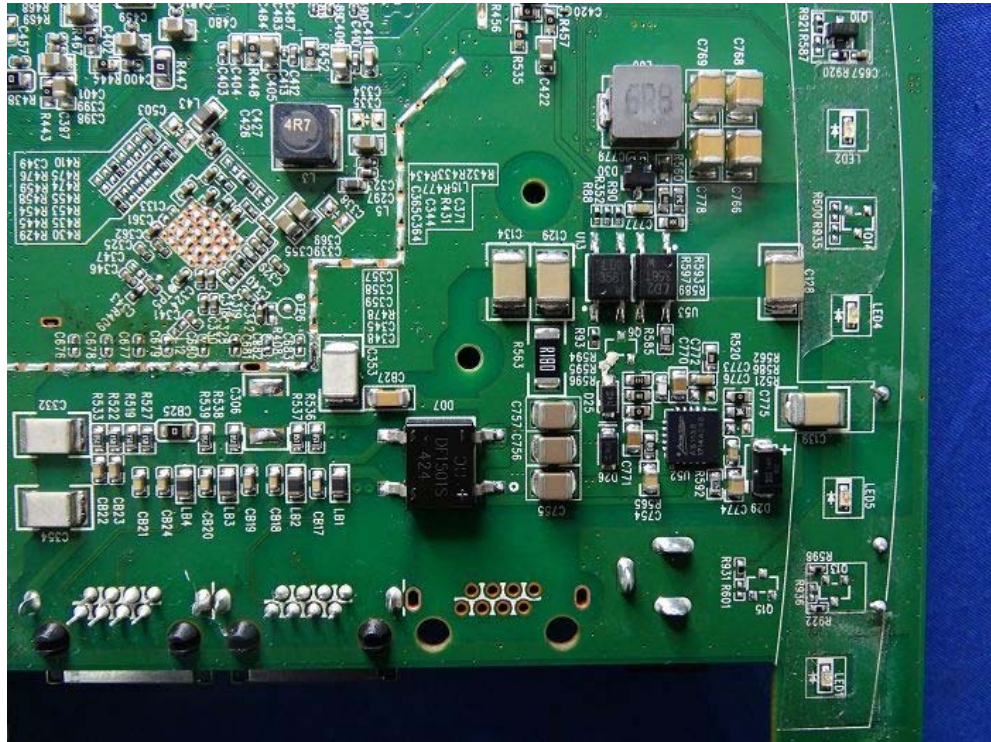
(25) EUT Photo
