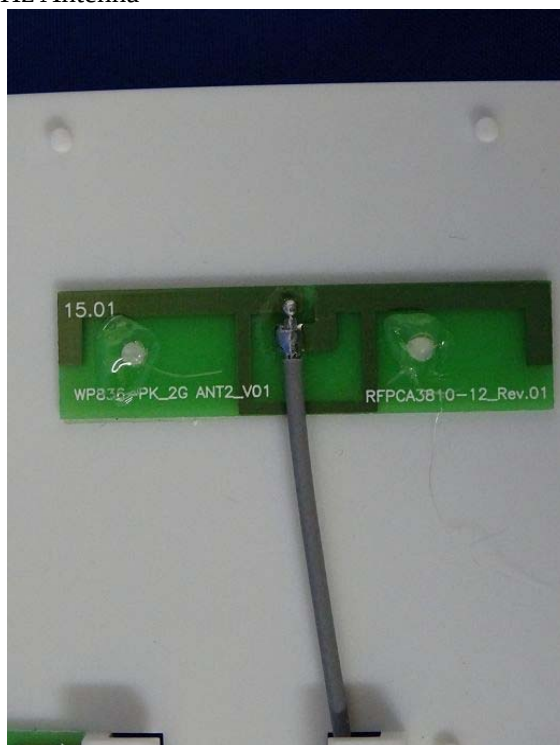
(32) EUT Photo-2.4GHz Antenna
