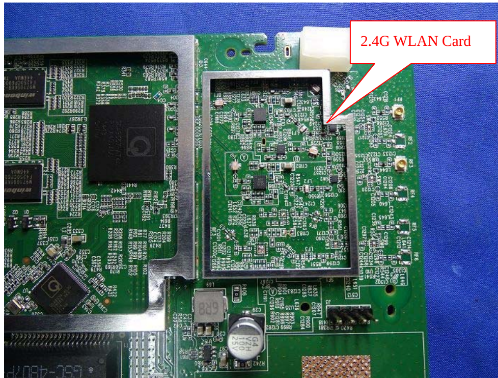
(27) EUT Photo
