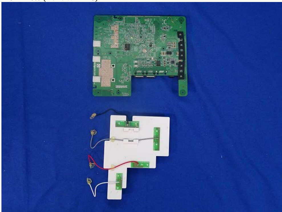
(52) EUT Photo (M/N: WK-1-C)
