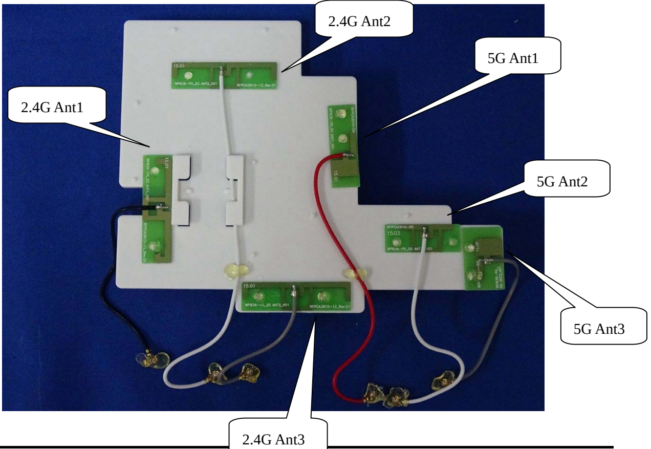
(25) EUT Photo
