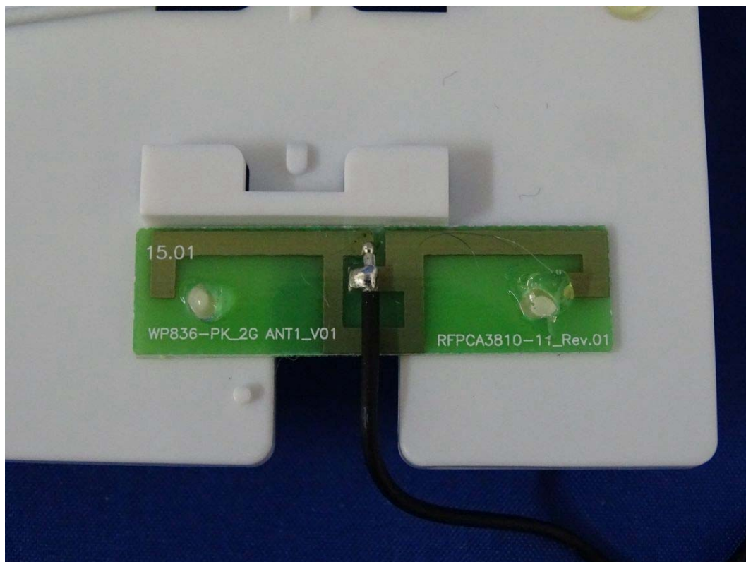
(28) EUT Photo-2.4G Ant-1
