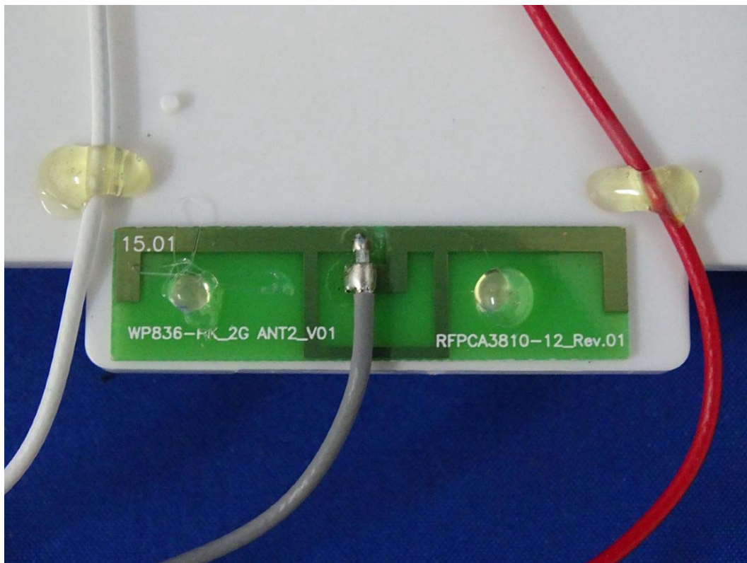
(26) EUT Photo-2.4G Ant-3
