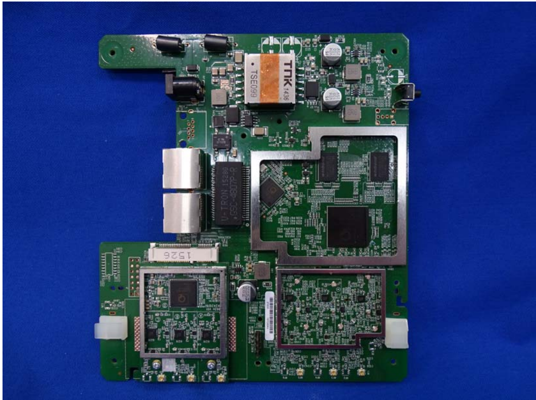
(52) EUT Photo (M/N: WK-2-C)
