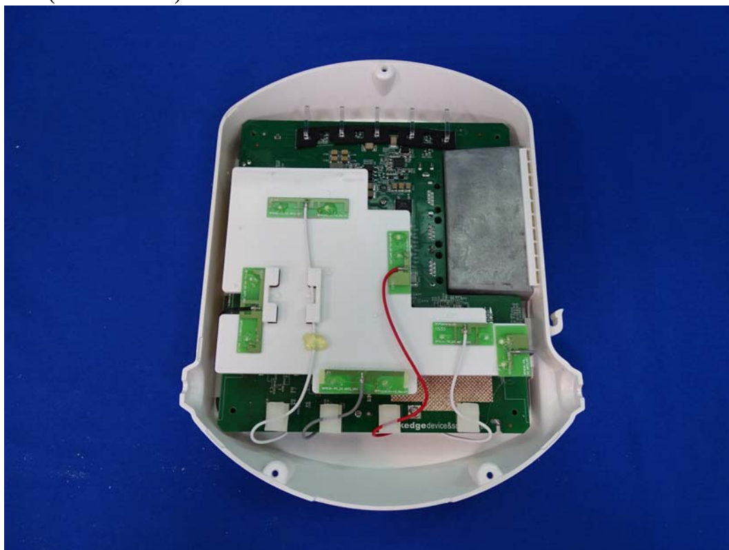
(45) EUT Photo (M/N: WK-2-C)
