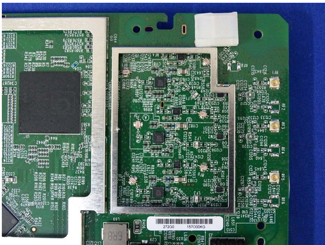
(19) EUT Photo (M/N: WK-2)
