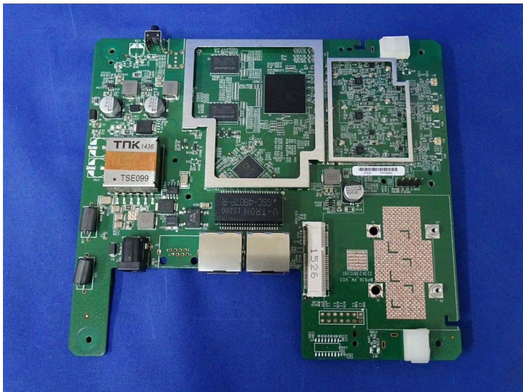
(21) EUT Photo (M/N: WK-2)
