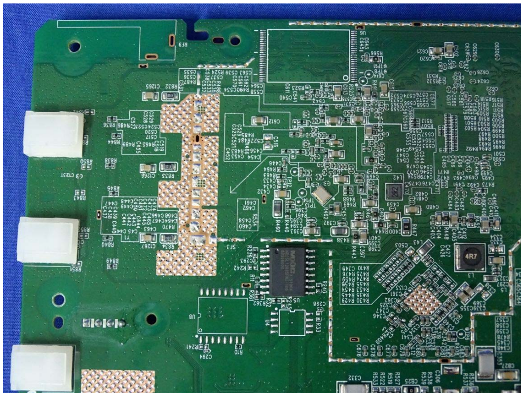
(9) EUT Photo (M/N: WK-2)
