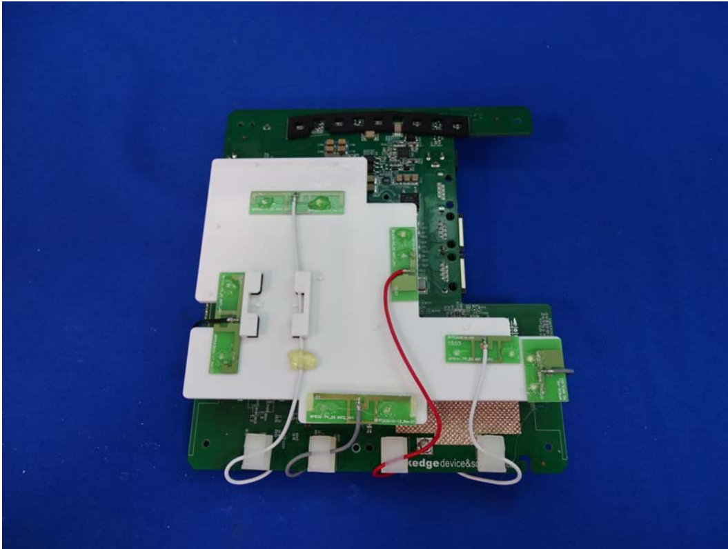
(47) EUT Photo (M/N: WK-2-C)
