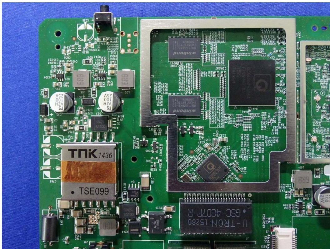
(17) EUT Photo (M/N: WK-2) 2.4G Module
