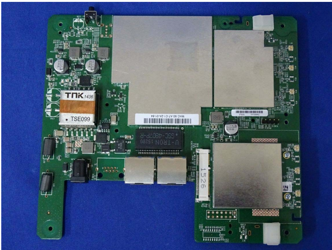
(14) EUT Photo (M/N: WK-2)
