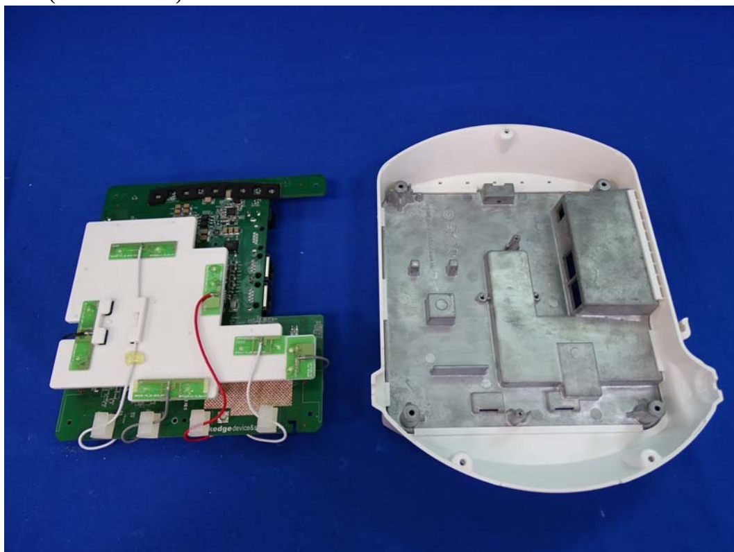
(46) EUT Photo (M/N: WK-2-C)
