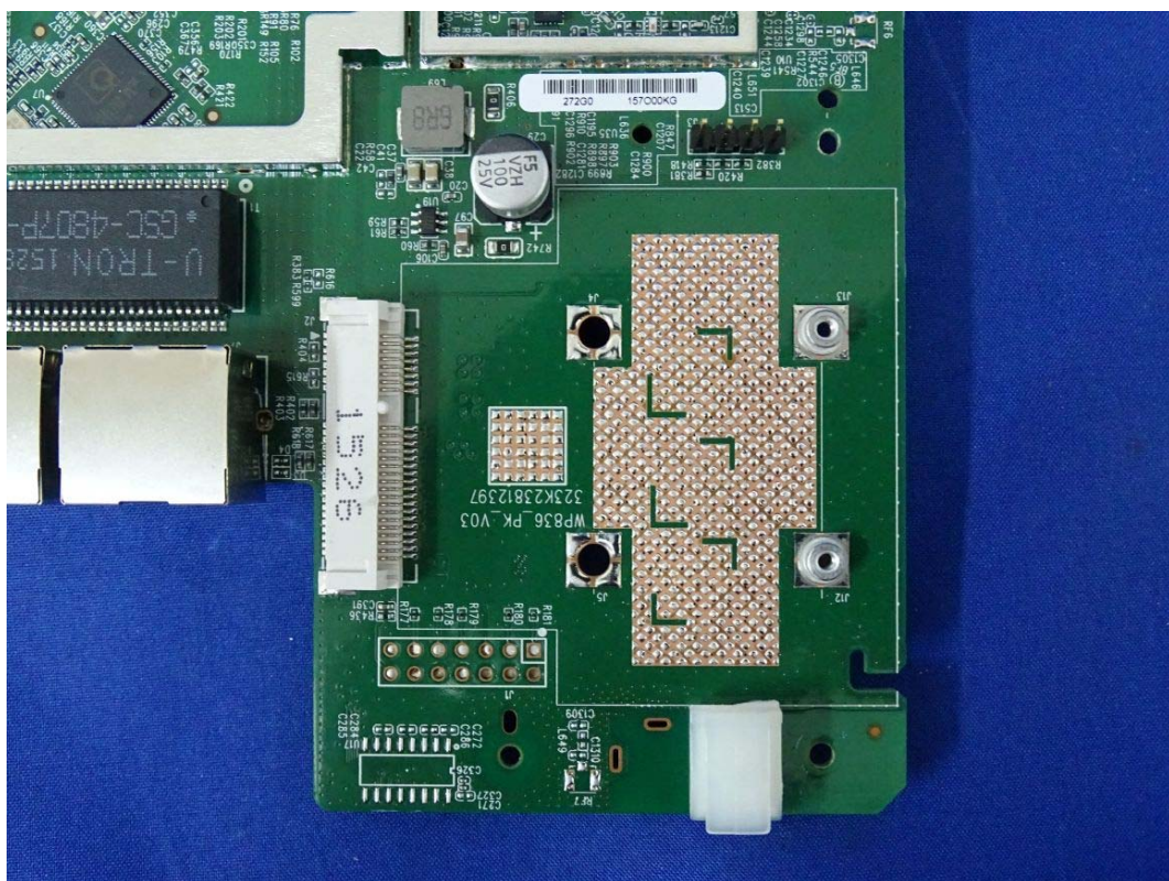
(22) EUT Photo (M/N: WK-2)
