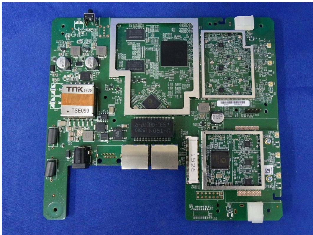
(16) EUT Photo (M/N: WK-2)
