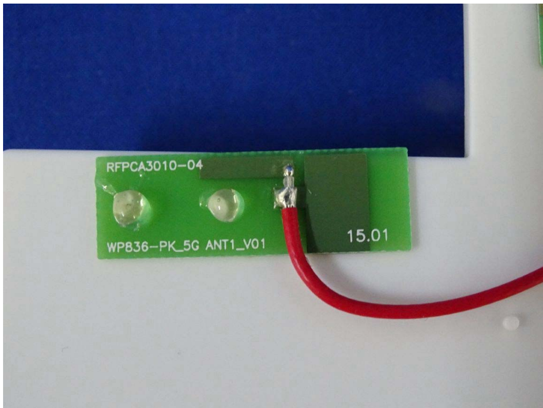
(31) EUT Photo (M/N: WK-2) 5G Ant-1
