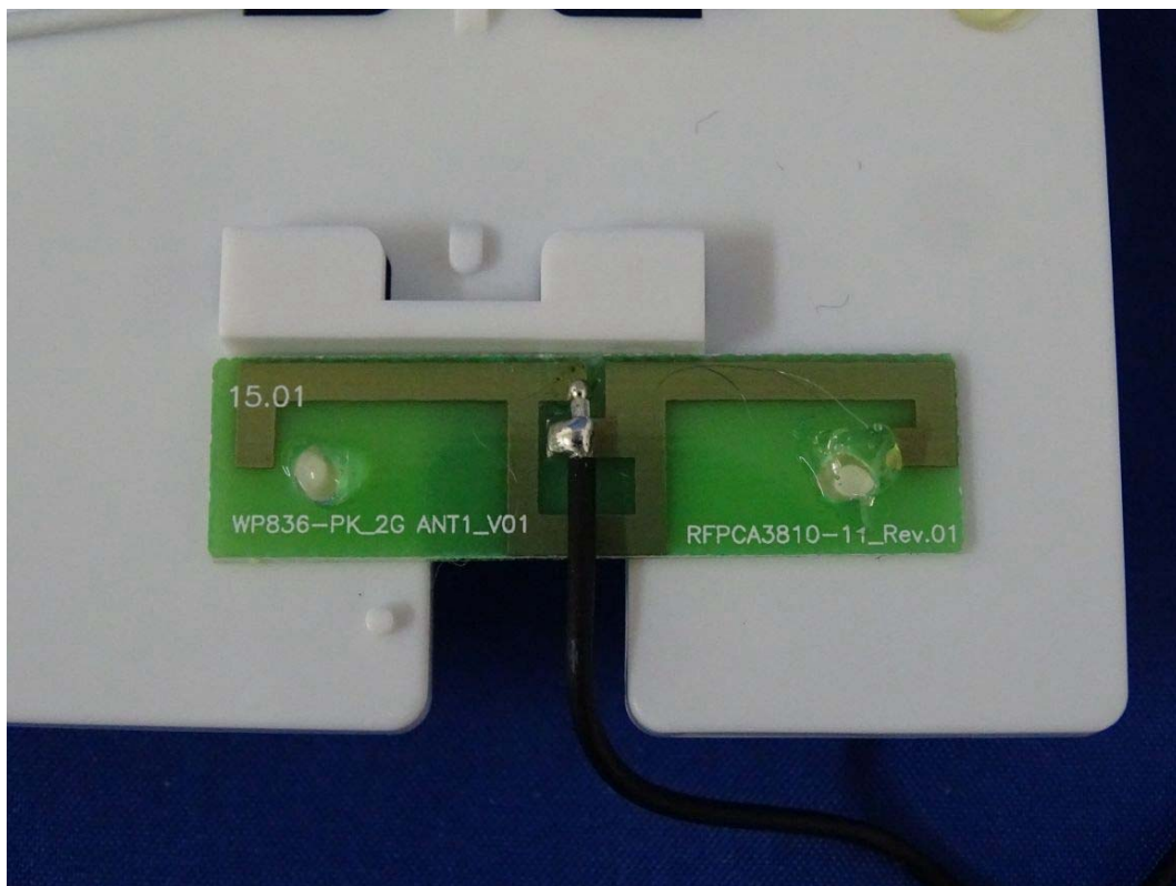
(28) EUT Photo (M/N: WK-2) 2.4G Ant-1
