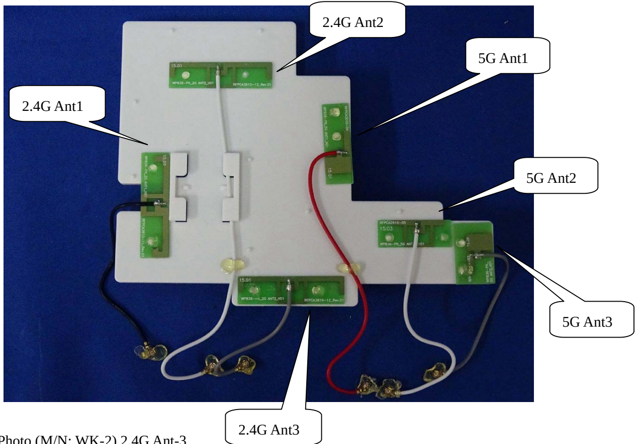
(26) EUT Photo (M/N: WK-2) 2.4G Ant-3
