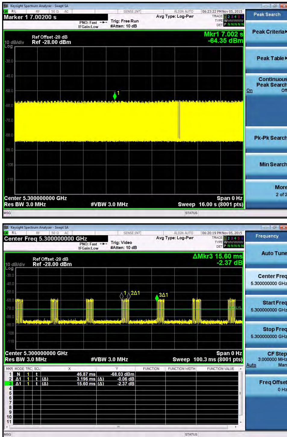
Plot of WLAN Traffic at 5300MHz-20BW
