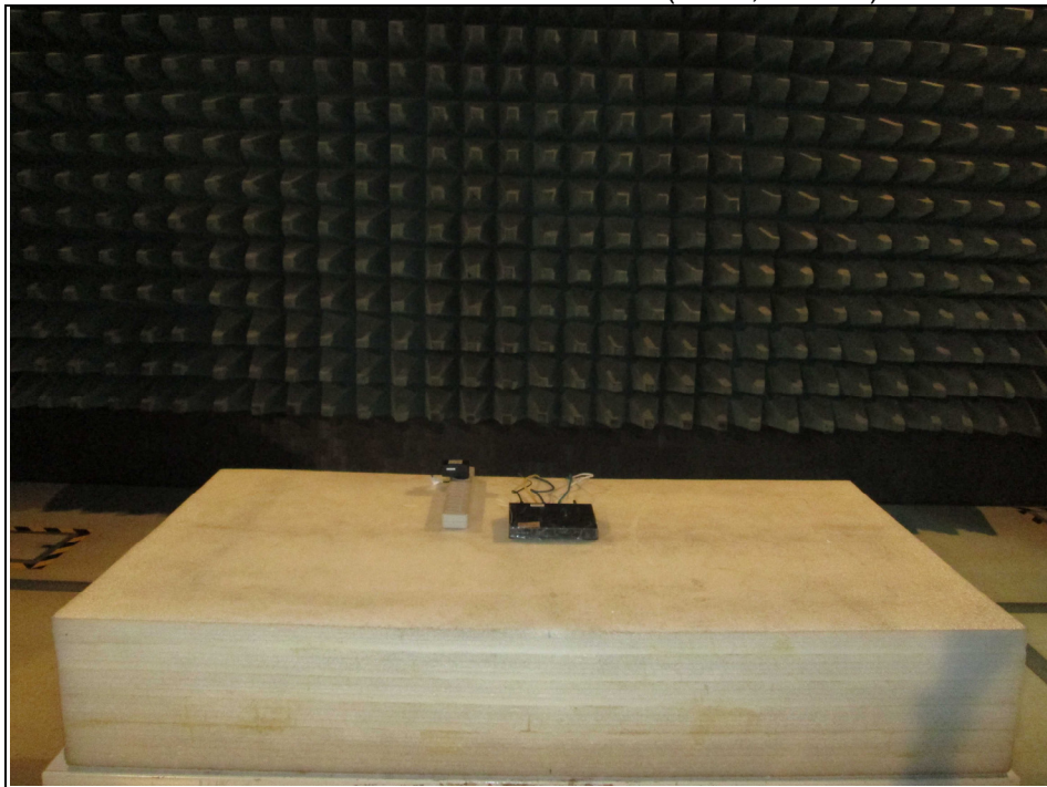
Radiated Emission Test below 1GHz (5GHz, Mode B)
