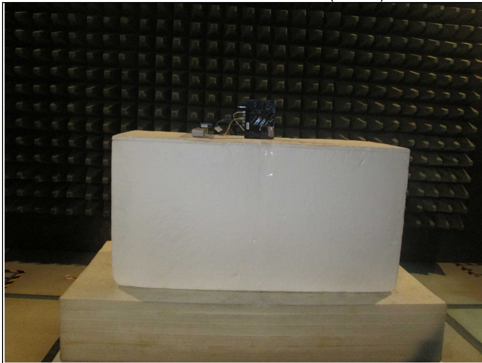
Radiated Emission Test above 1GHz (2.4GHz)
