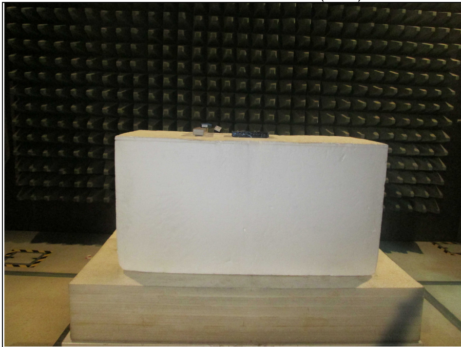
Radiated Emission Test above 1GHz (5GHz)
