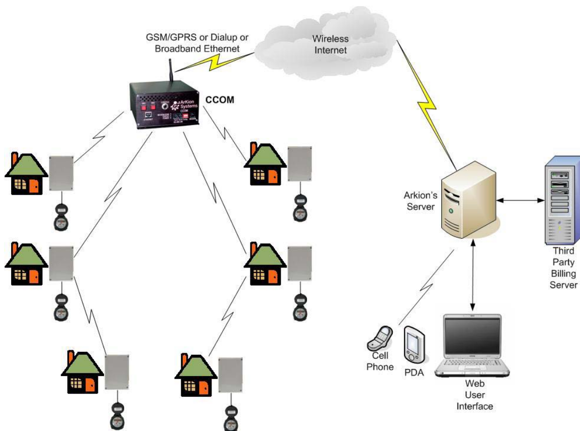
Figure 2.1 Water Meters Connected to ArKion Systems Network
