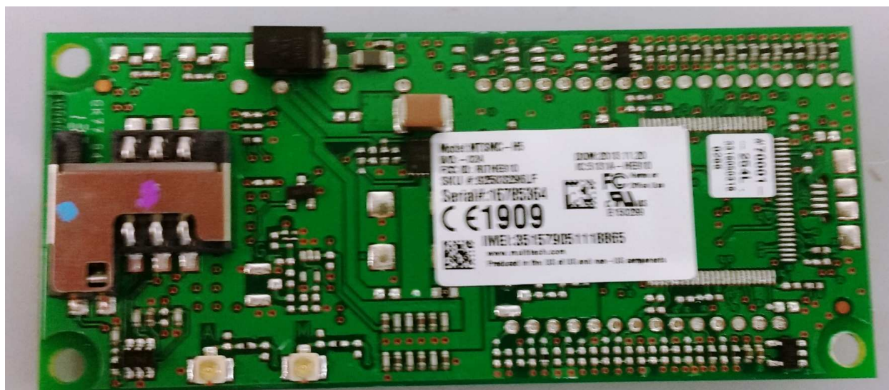
Figure 16: Internal Photo – Modem Top
