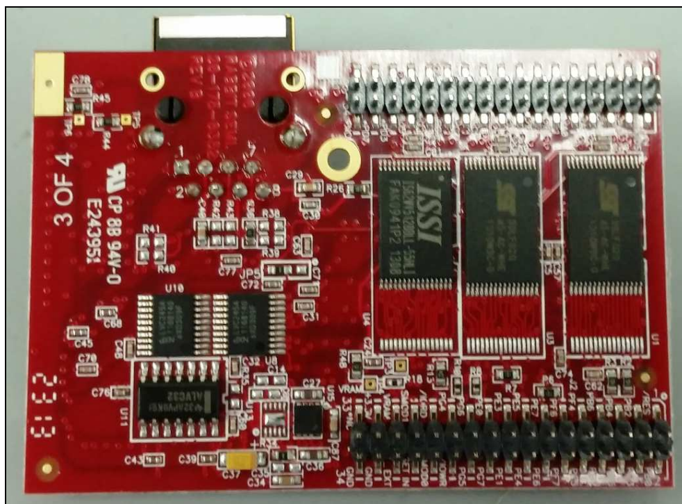
Figure 19: Internal Photo – Rabbit Bottom
