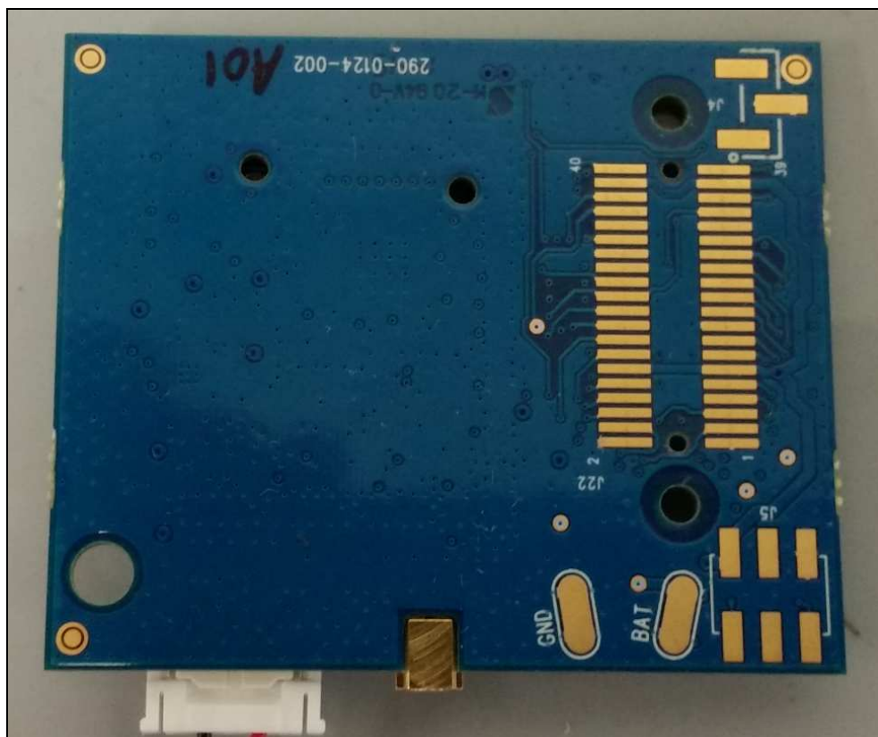
Figure 13: Internal Photo – LFM Bottom
