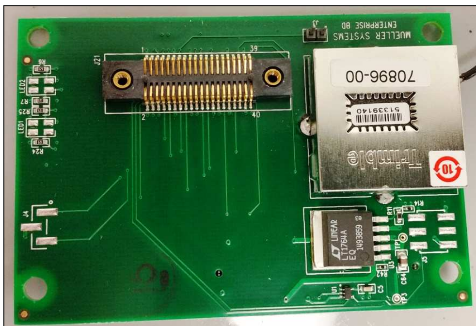
Figure 9: Internal Photo – GPS Top
