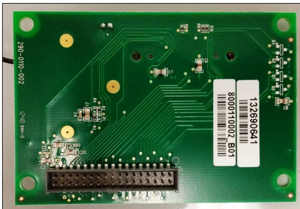
Figure 10: Internal Photo – GPS Bottom
