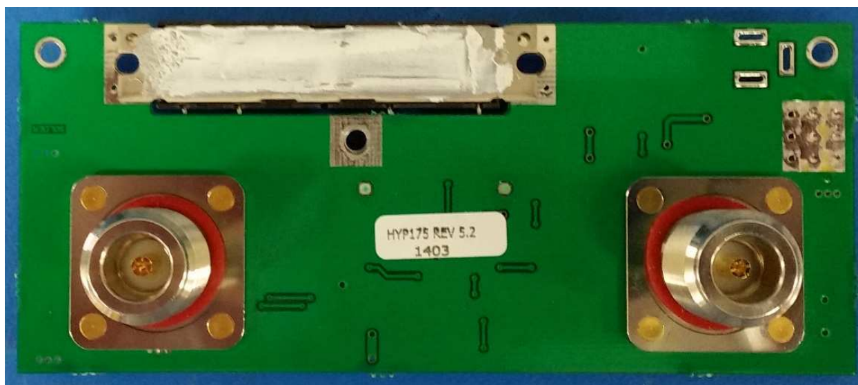
Figure 8: Internal Photo – Amp Bottom
