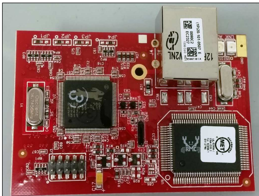
Figure 18: Internal Photo – Rabbit Top
