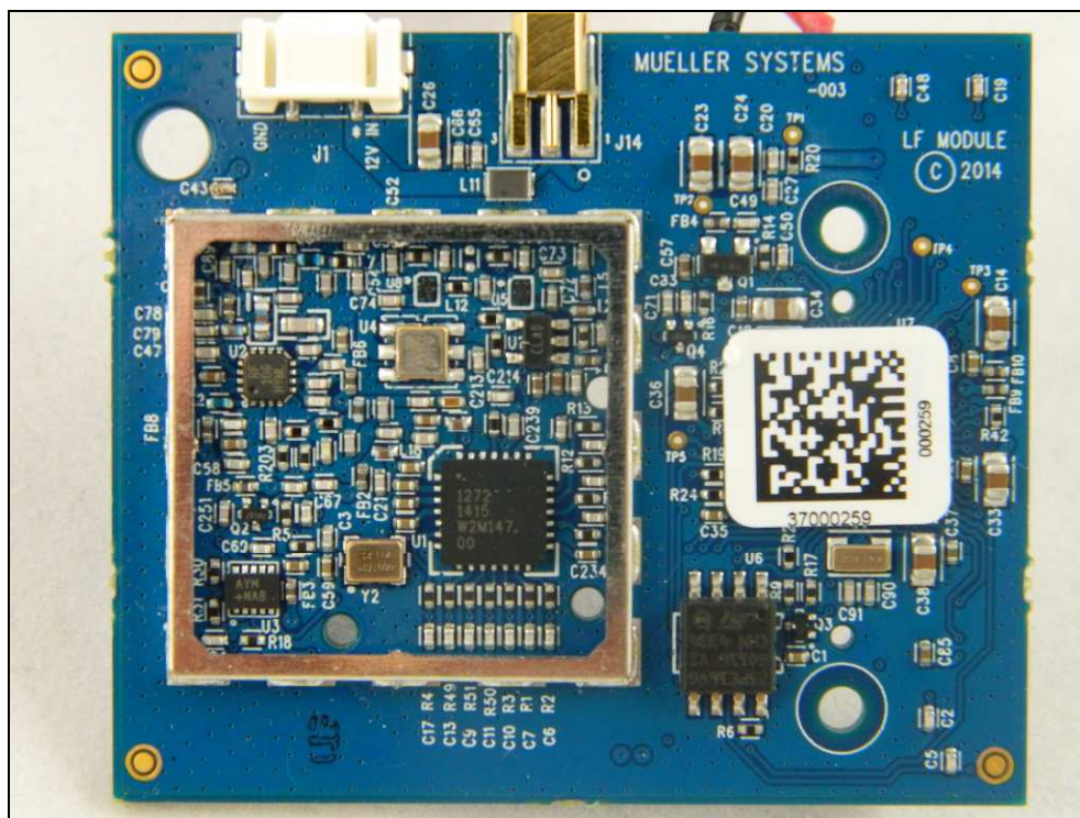
Figure 12: Internal Photo – LFM Top, Shield Removed
