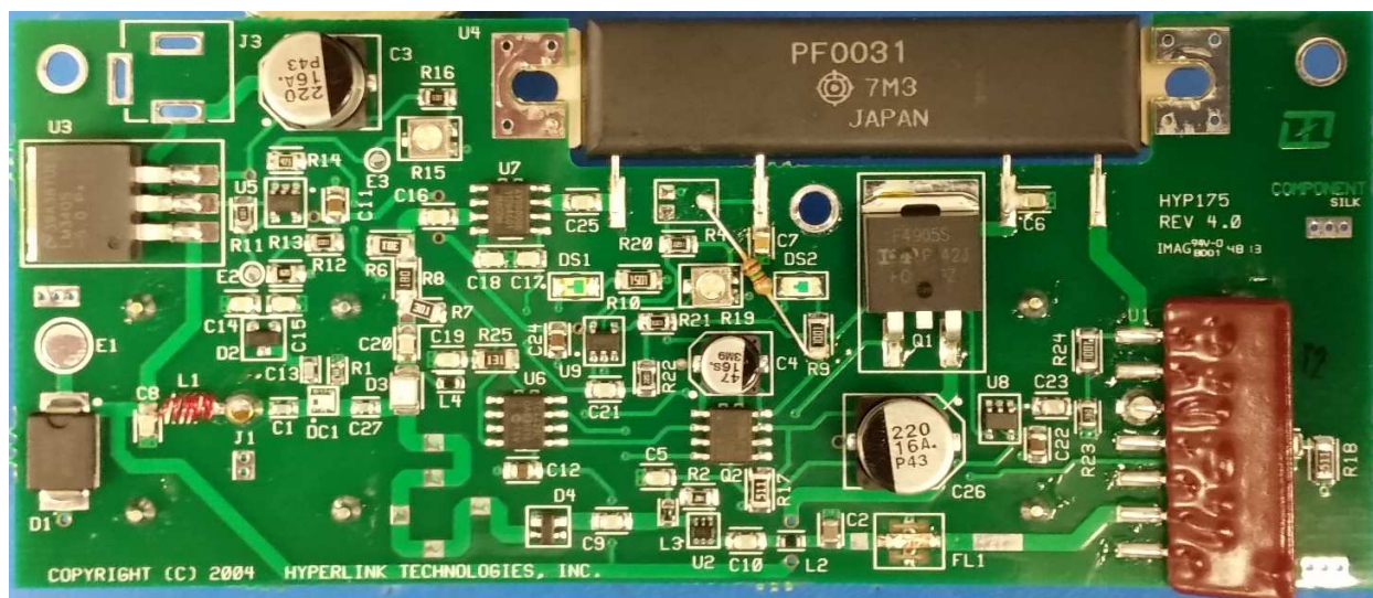
Figure 7: Internal Photo – Amp Top
