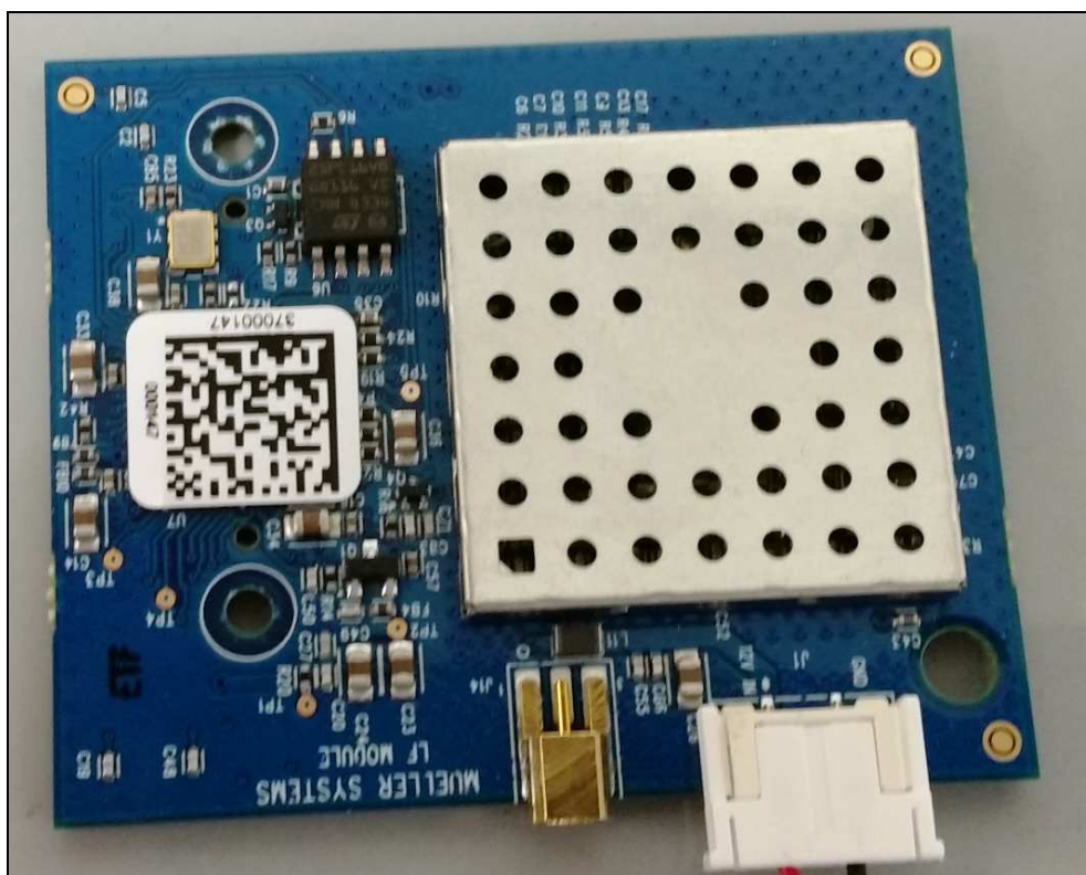
Figure 11: Internal Photo – LFM Top
