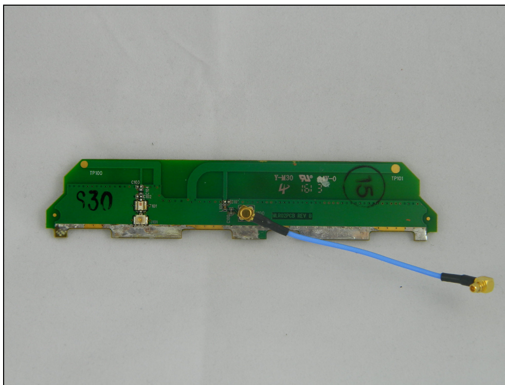
Figure 4: External Photo – Printed Inverted F Antenna
