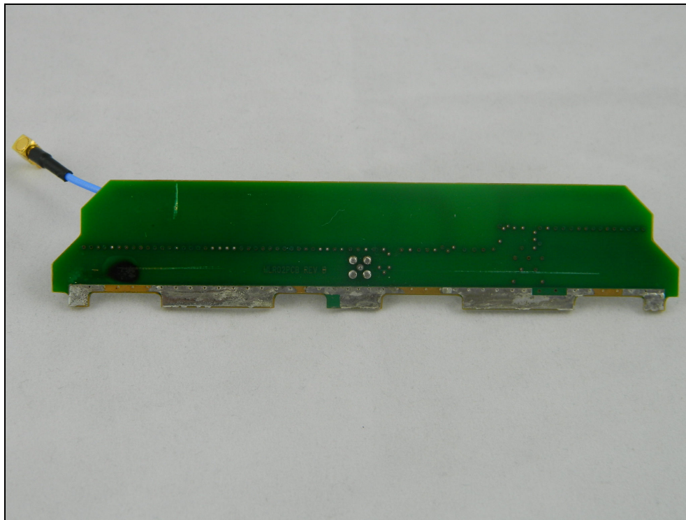
Figure 3: External Photo – Printed Inverted F Antenna
