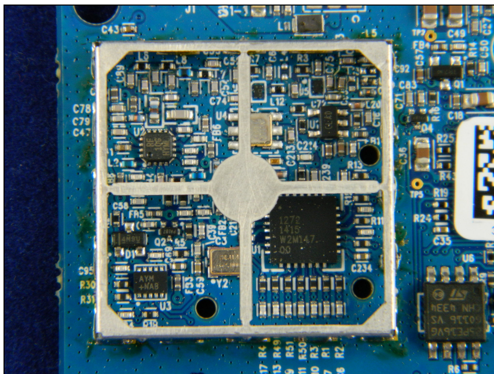
Figure 2: Internal Photo Shield Removed
