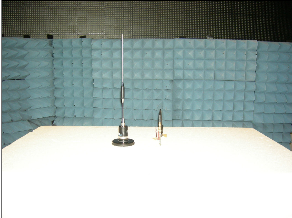
Figure 4: Radiated Emissions – DSS
