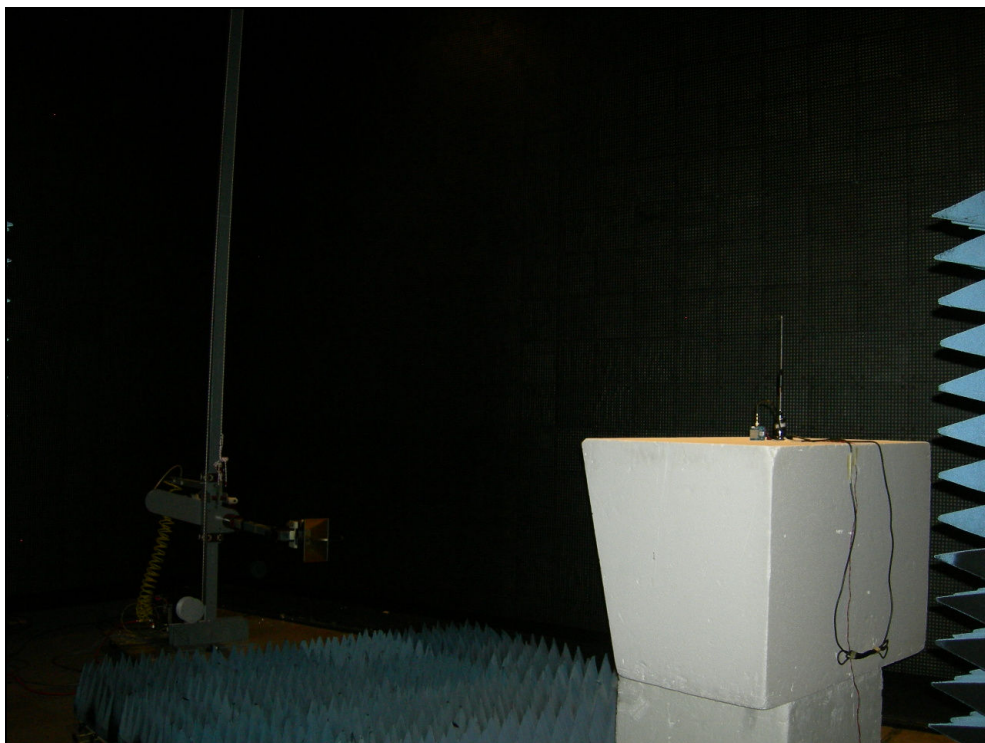
Figure 6: Radiated Emissions – DSS
