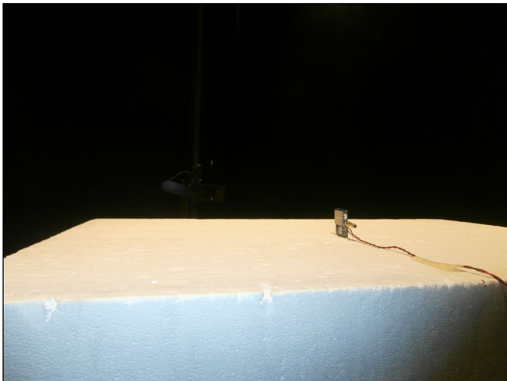
Figure 2: Radiated Emissions – DTS
