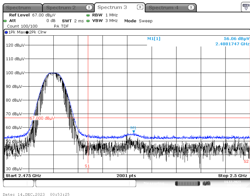
Radiated Restricted Band Edges plot – Peak Result (Ch.39, Z-H)
