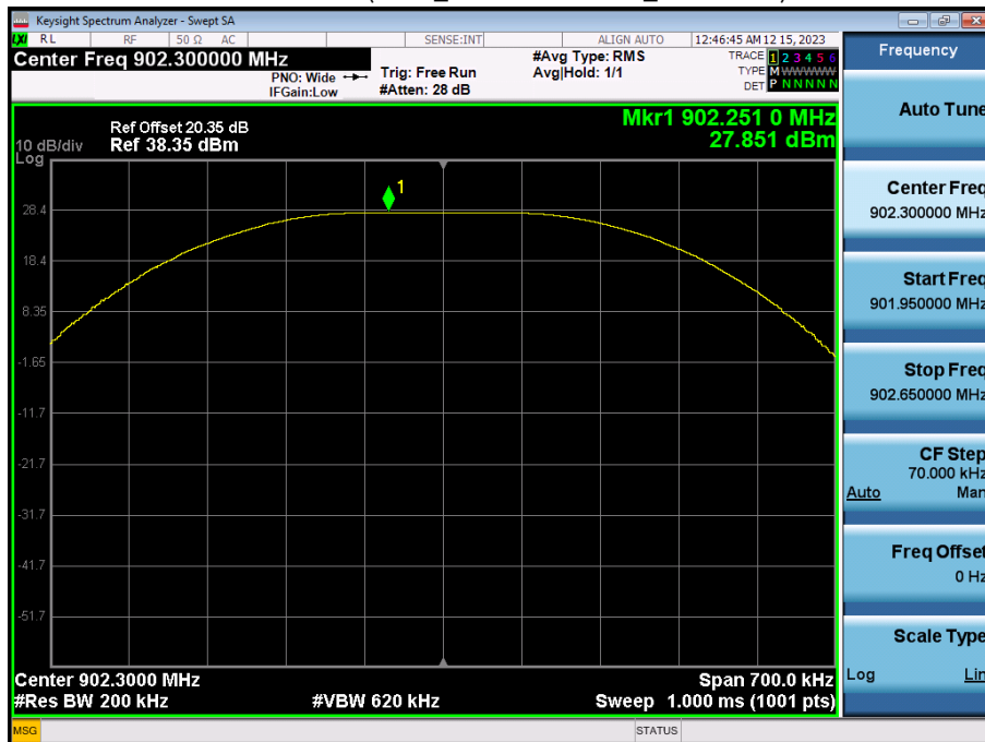
Peak Power (SF10_Packet Lenth 24_Channel 0)
