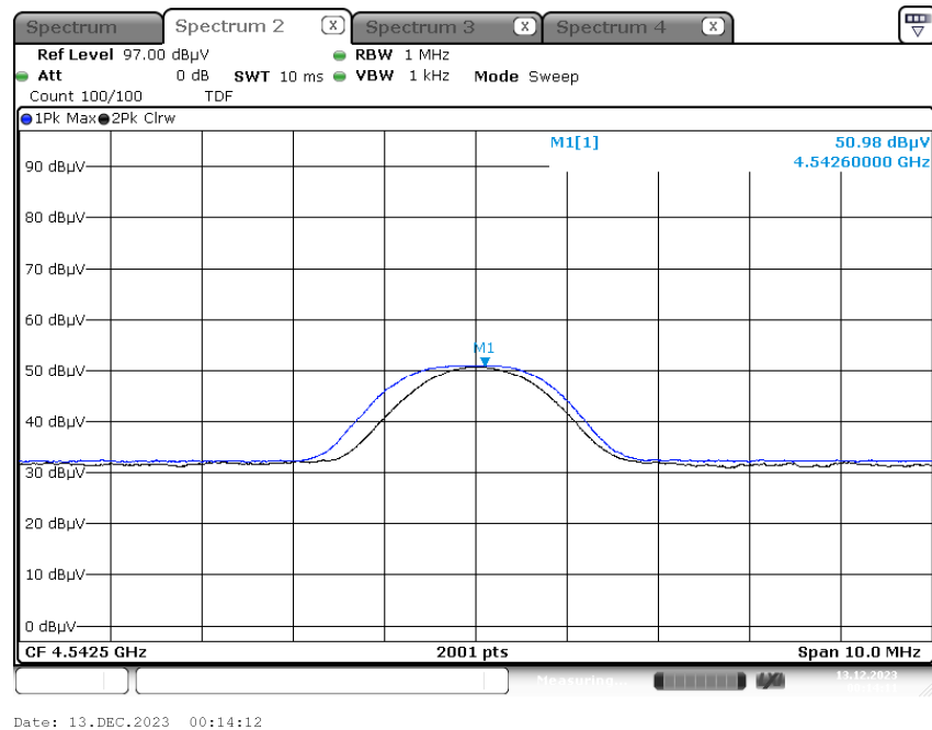
Radiated Spurious Emissions plot – Average Result (SF10 4 th Harmonic)
