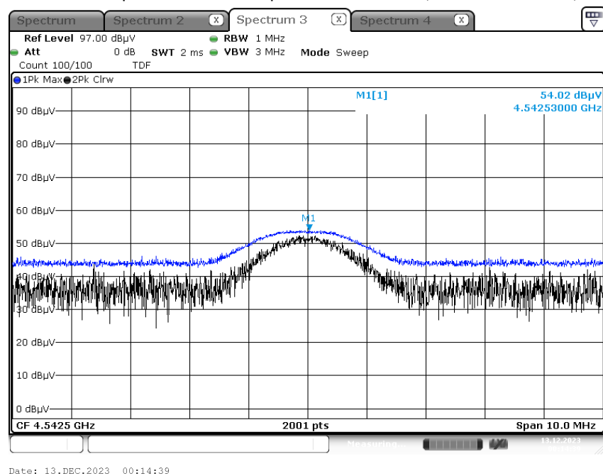
Radiated Spurious Emissions plot – Peak Result (SF10 4 th Harmonic)
