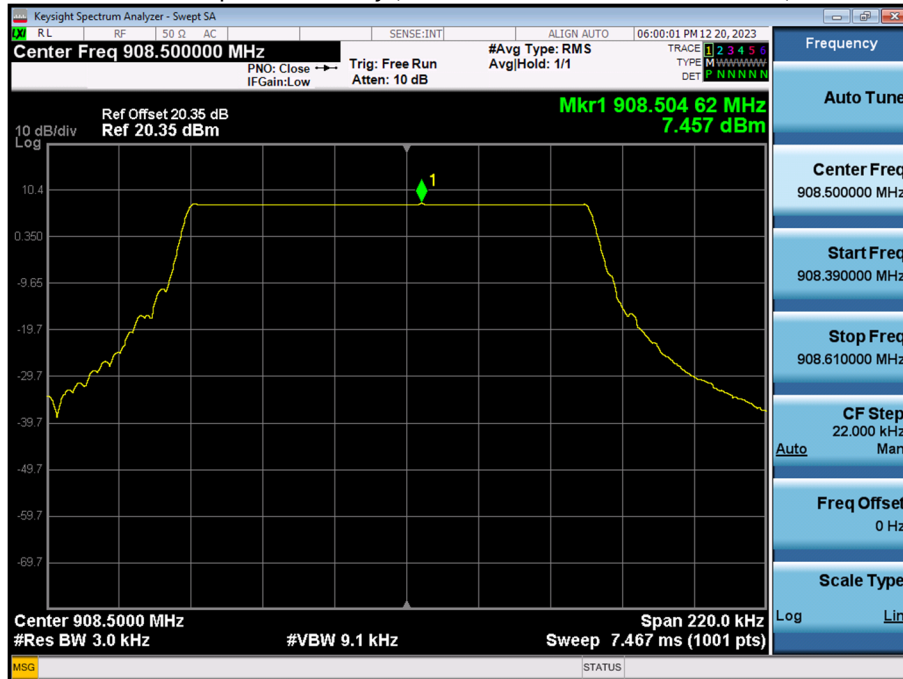
Power Spectral Density (SF10_Packet Lenth 24_Channel 31)
