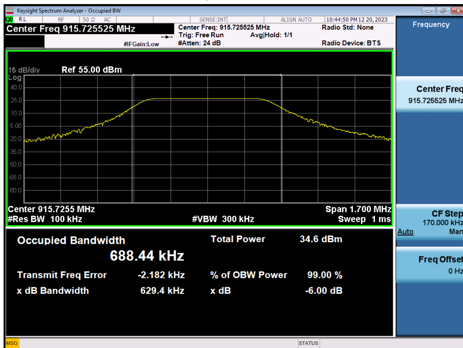
6 dB Bandwidth plot (SF7 - Private Channel)
