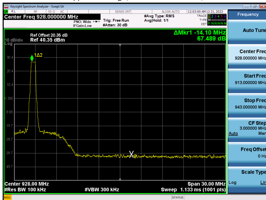
Upper Band Edge(SF 12- Private Channel)
