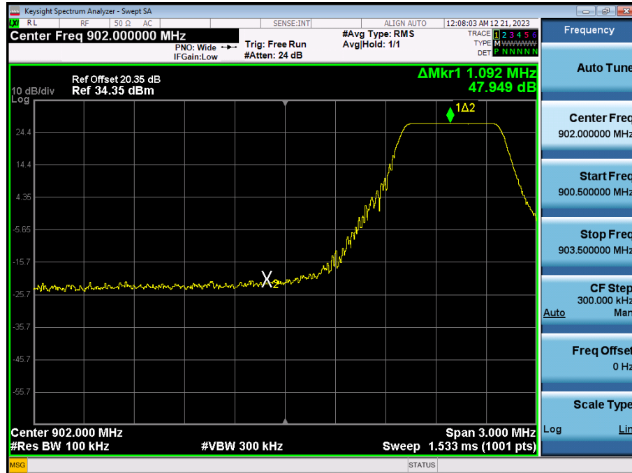
Lower Band Edge(SF 12- Channel 64)
