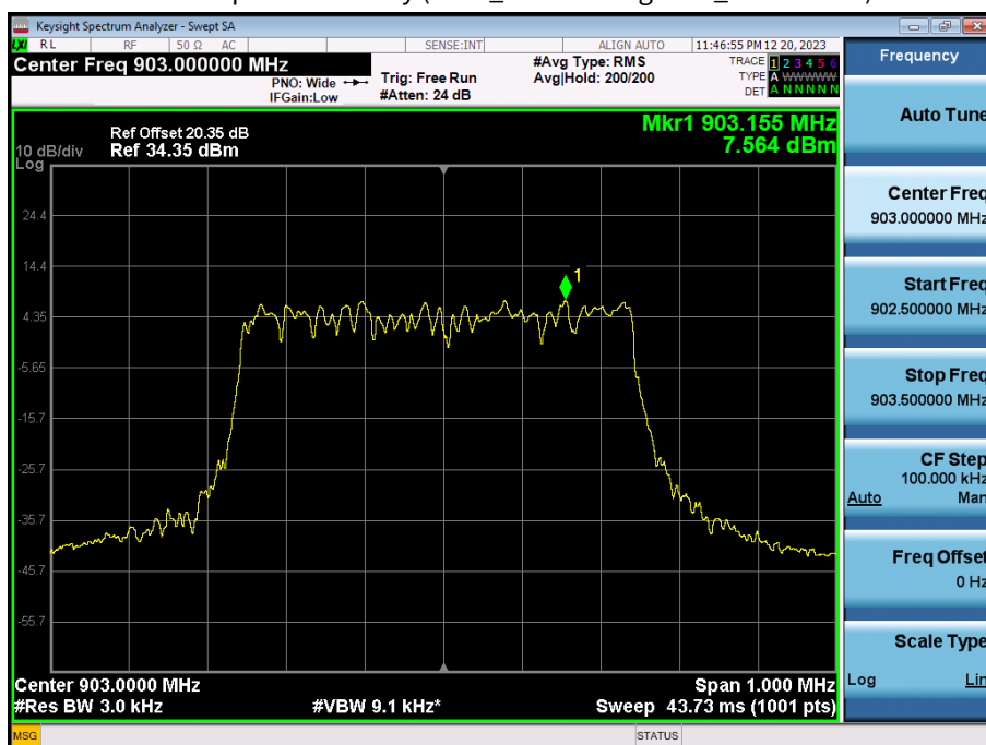
Power Spectral Density (SF12_Packet Length 36_Channel 64)
