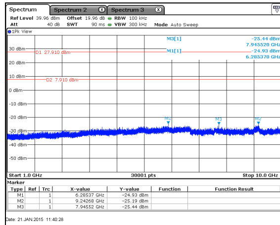
Figure 7.5.2.2-2: 1 GHz – 10 GHz – LCH 2604.2bps
