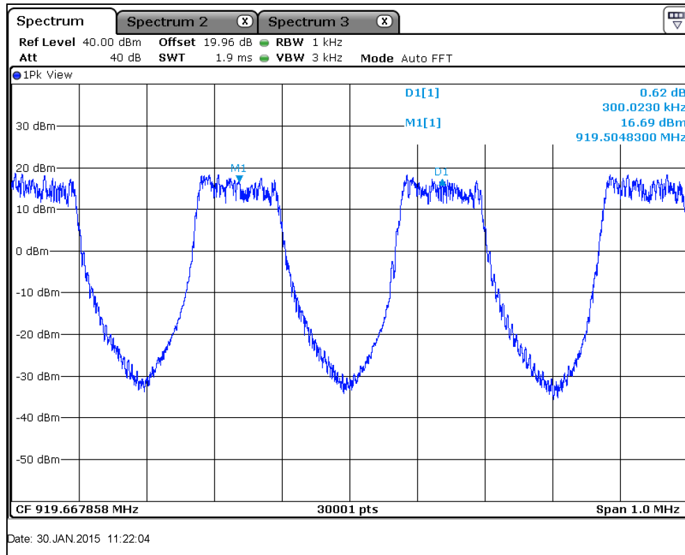
Figure 7.4.1.2-2: Carrier Frequency Separation 4557.3bps
