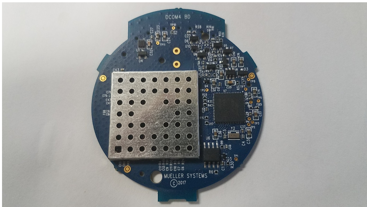
Figure 1: Top View
