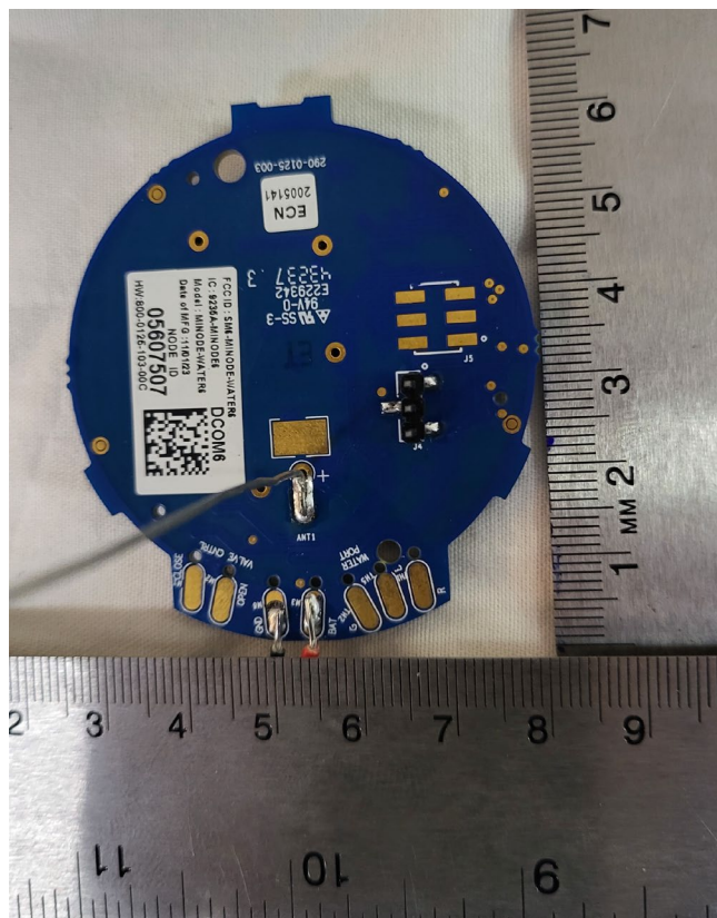
Figure 2. PCB – Back
