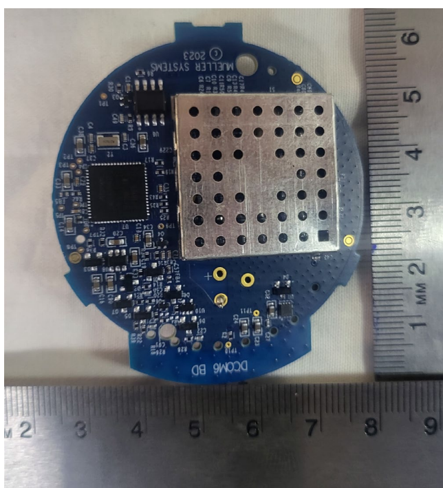
Figure 1. PCB – Front
