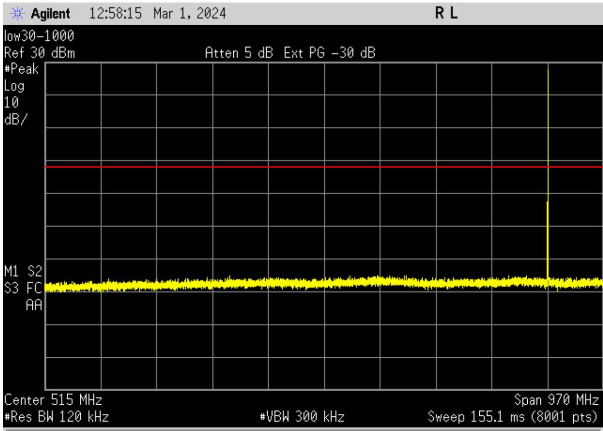
Figure 2. Conducted Spurious Emissions-Low Channel, 30MHz – 1 GHz
