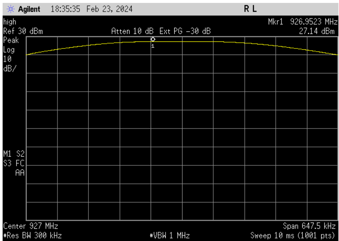
Figure 20. Peak Antenna Conducted Output Power, High Channel
