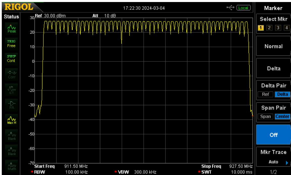
Figure 17. Hopping Channels 102 through 151
