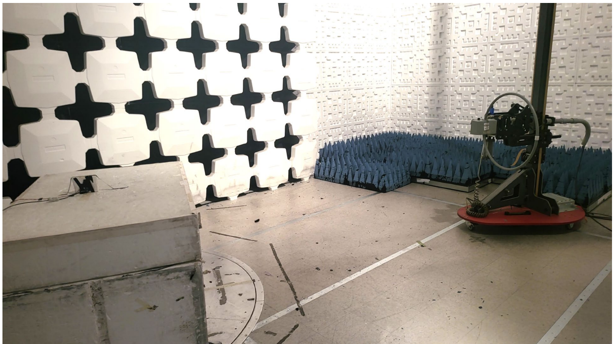
Figure 2. Radiated Emissions Test Setup (9 kHz - 30 MHz)
