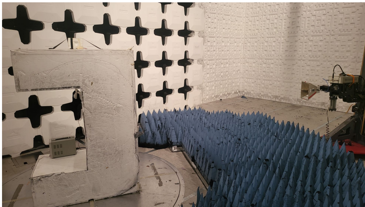
Figure 4. Radiated Emissions Test Setup (above 1 GHz)
