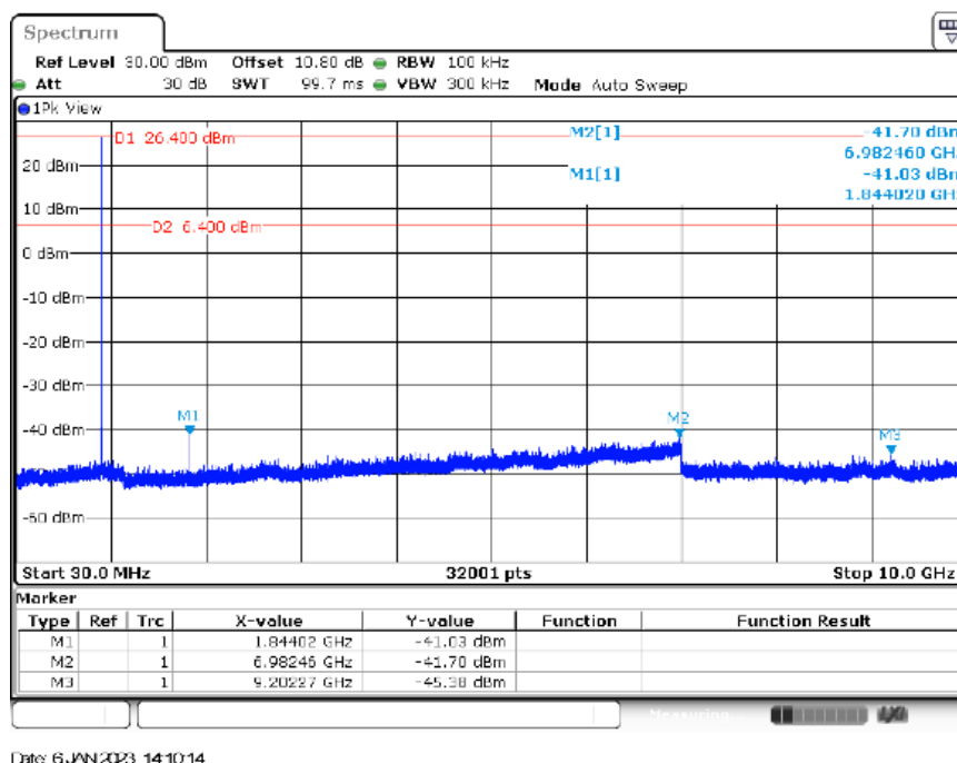
Figure 2.4.6-2: 30MHz-10 GHz- MCH
