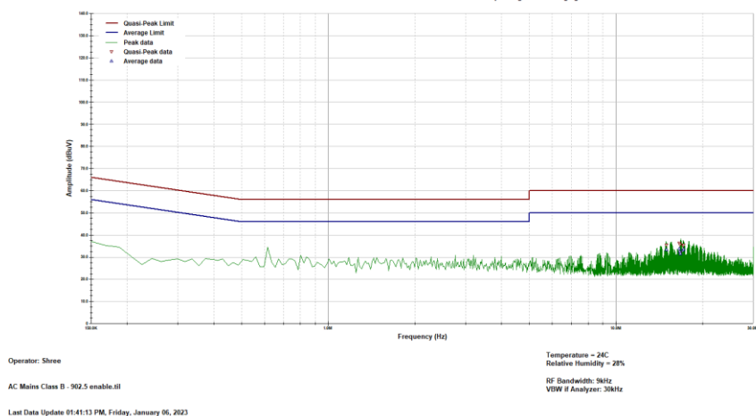
Figure 2.2.6-2 – Graphical Results – AC Mains N Plot
