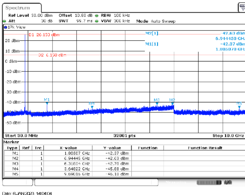
Figure 2.4.6-1: 30MHz-10 GHz- LCH
