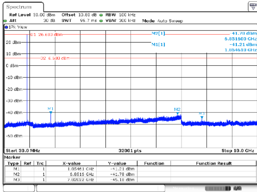
Figure 2.4.6-3: 30MHz-10 GHz- HCH
