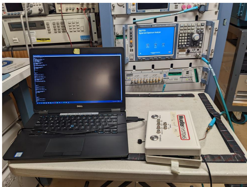
Figure 4: Test Setup – Antenna Port Measurement
