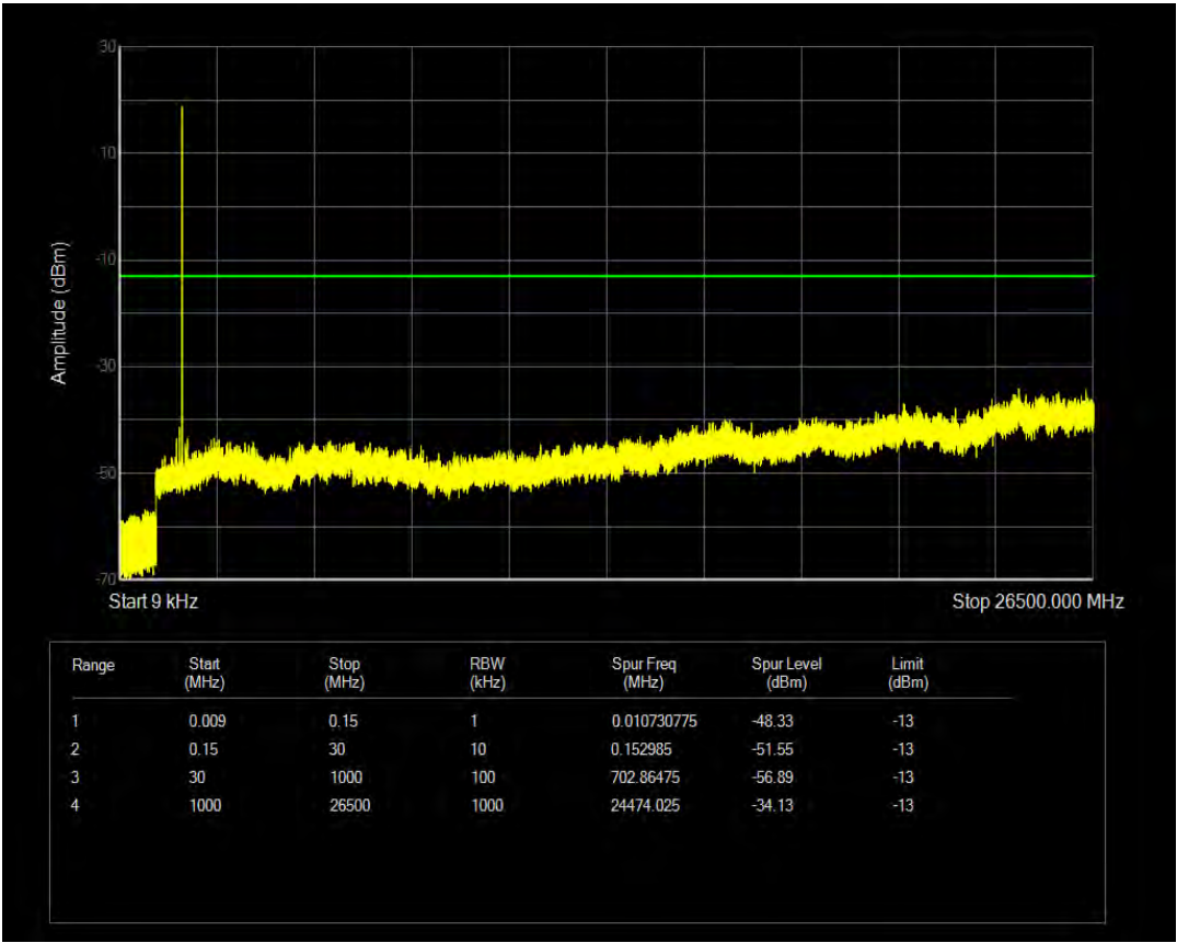
Band4 16QAM BW=15MHz Channel=20025 RB Size=6 Position=#0 NB Index=0
