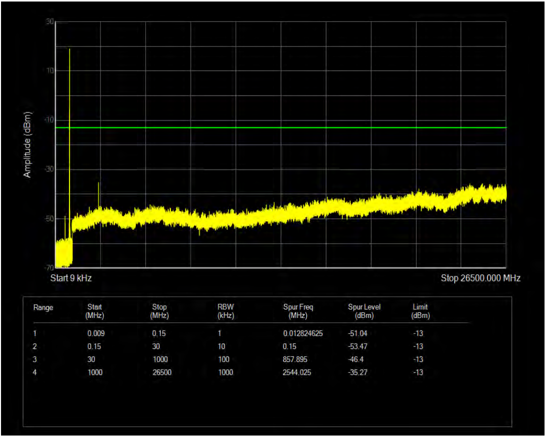
Band5 16QAM BW=1.4MHz Channel=20643 RB Size=6 Position=#0 NB Index=0
