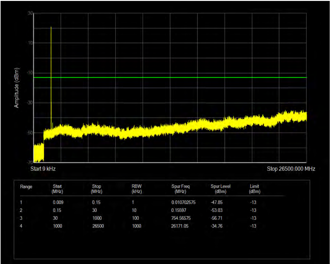
Band4 16QAM BW=20MHz Channel=20050 RB Size=6 Position=#0 NB Index=0
