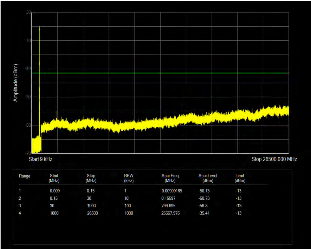
Band5 16QAM BW=5MHz Channel=20625 RB Size=6 Position=#0 NB Index=0
