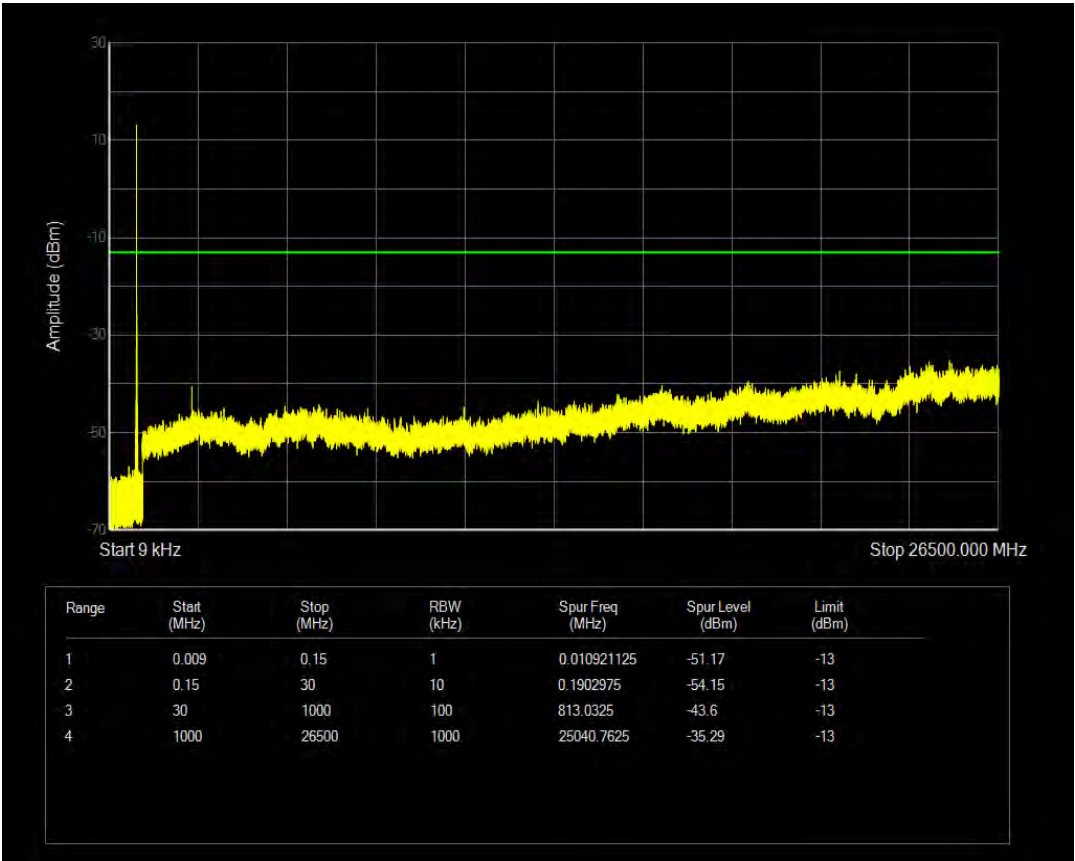
Band26(824-849) QPSK BW=1.4MHz Channel=27033 RB Size=1 Position=#0 NB Index=0
