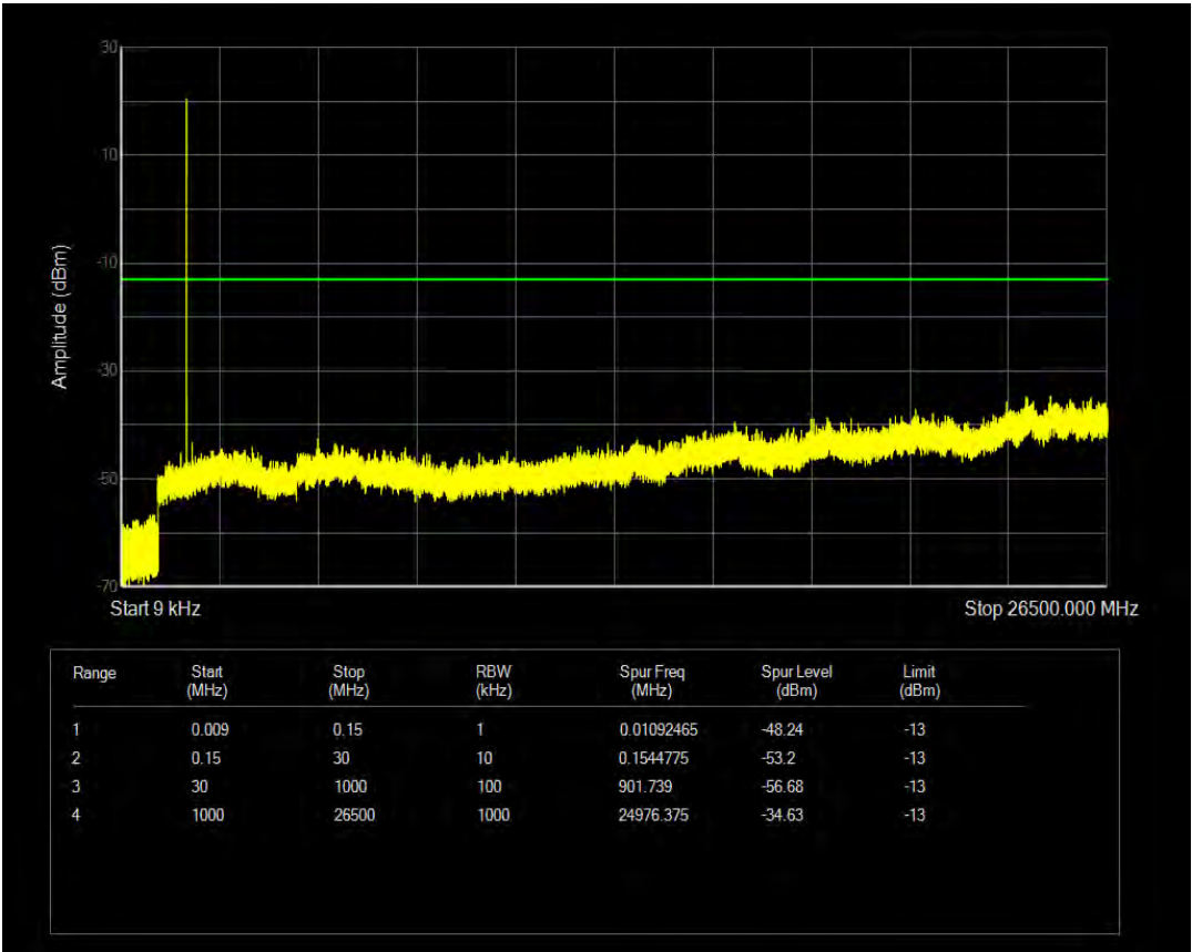
Band66 16QAM BW=15MHz Channel=132597 RB Size=6 Position=#0 NB Index=0
