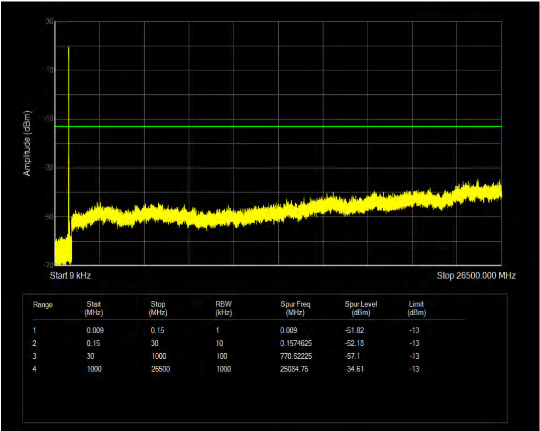
Band5 16QAM BW=10MHz Channel=20600 RB Size=6 Position=#0 NB Index=0
