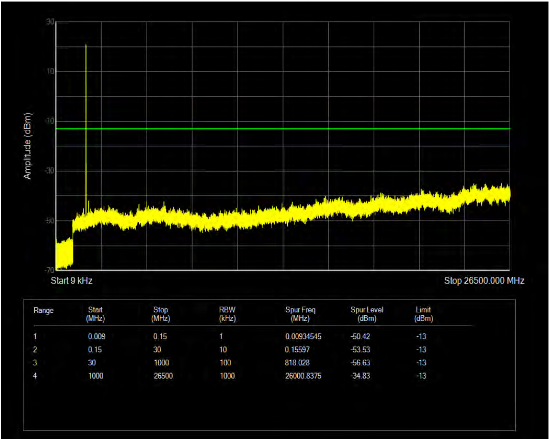
Band66 16QAM BW=10MHz Channel=132622 RB Size=6 Position=#0 NB Index=0
