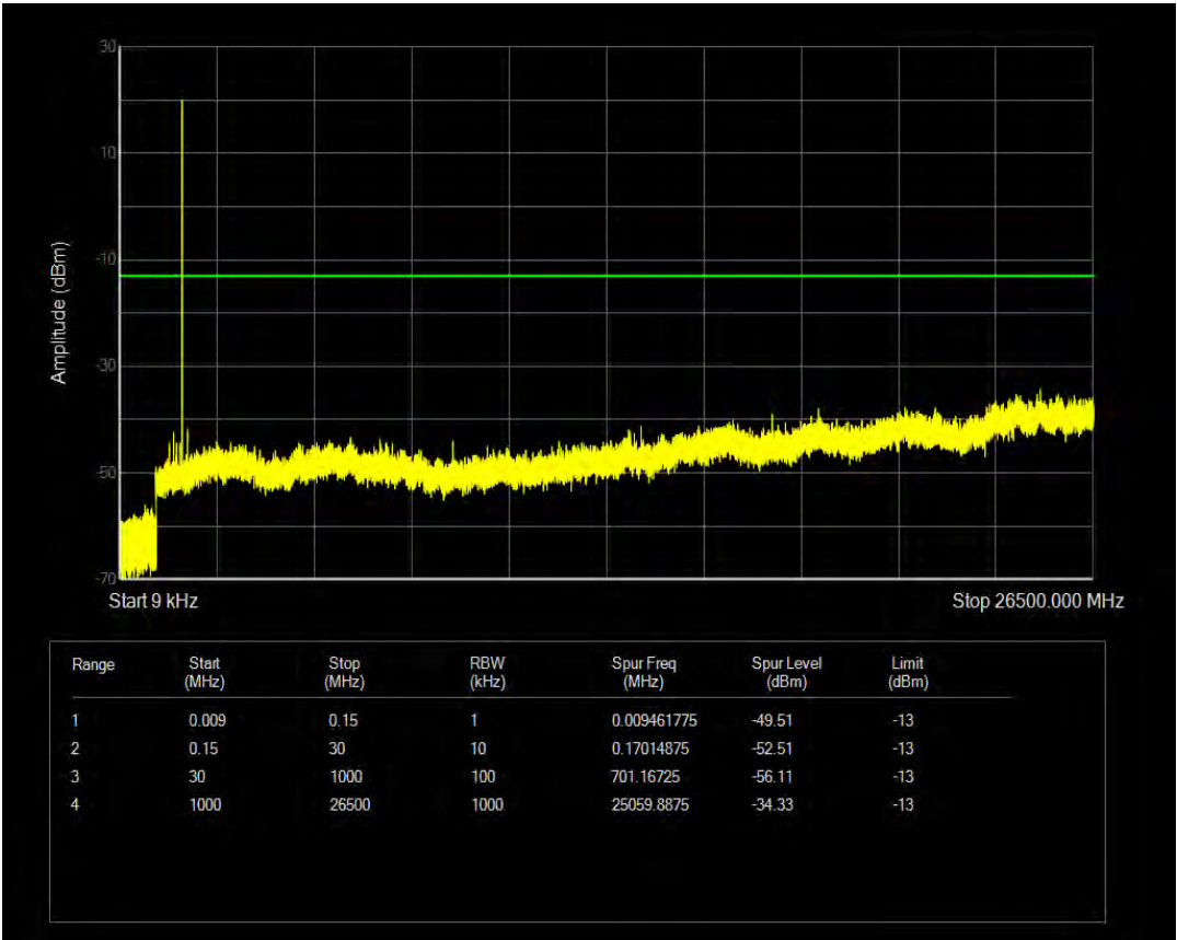
Band4 16QAM BW=1.4MHz Channel=19957 RB Size=6 Position=#0 NB Index=0
