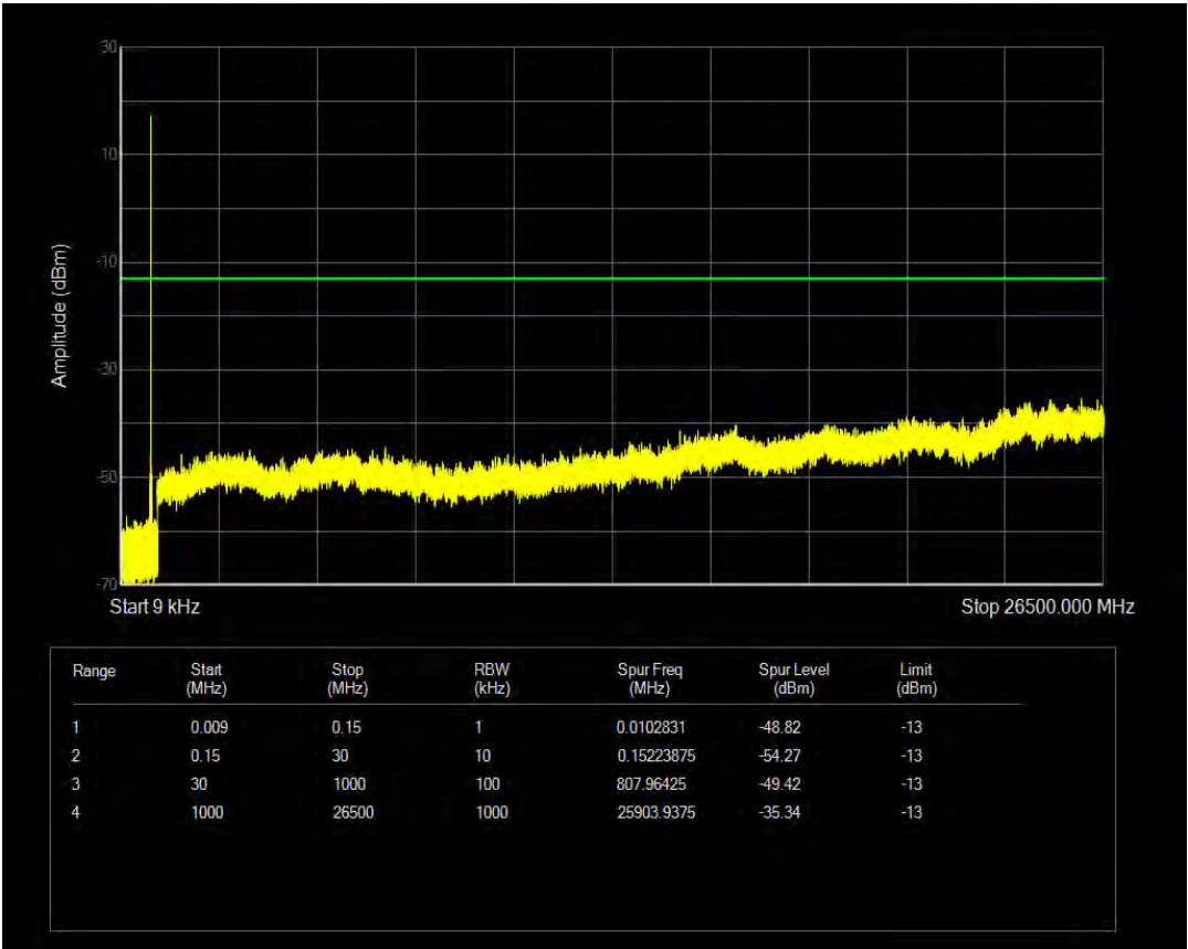
Band5 16QAM BW=3MHz Channel=20415 RB Size=6 Position=#0 NB Index=0
