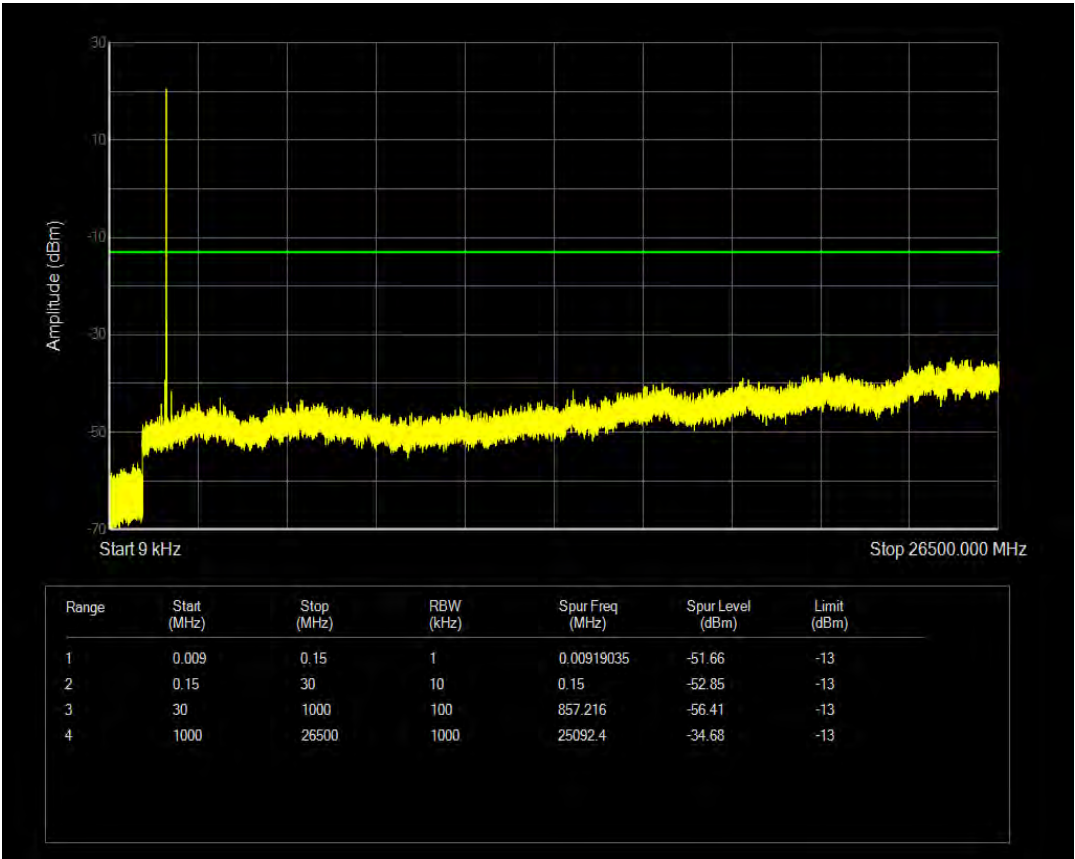
Band4 16QAM BW=3MHz Channel=19965 RB Size=6 Position=#0 NB Index=0
