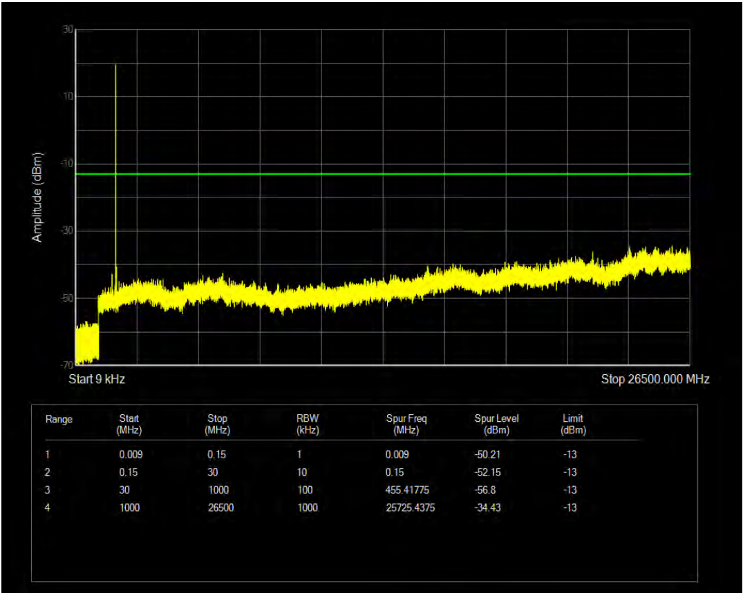
Band4 16QAM BW=20MHz Channel=20300 RB Size=6 Position=#0 NB Index=0
