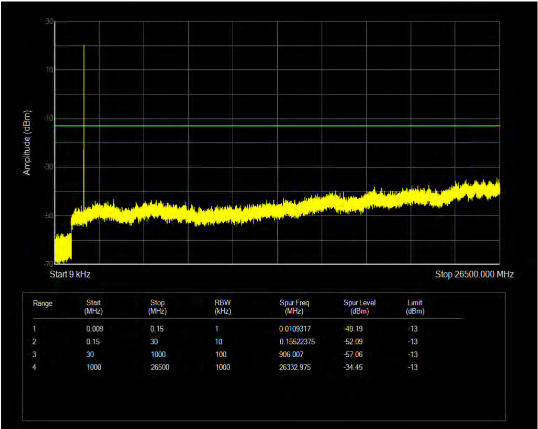
Band4 16QAM BW=3MHz Channel=20385 RB Size=6 Position=#0 NB Index=0
