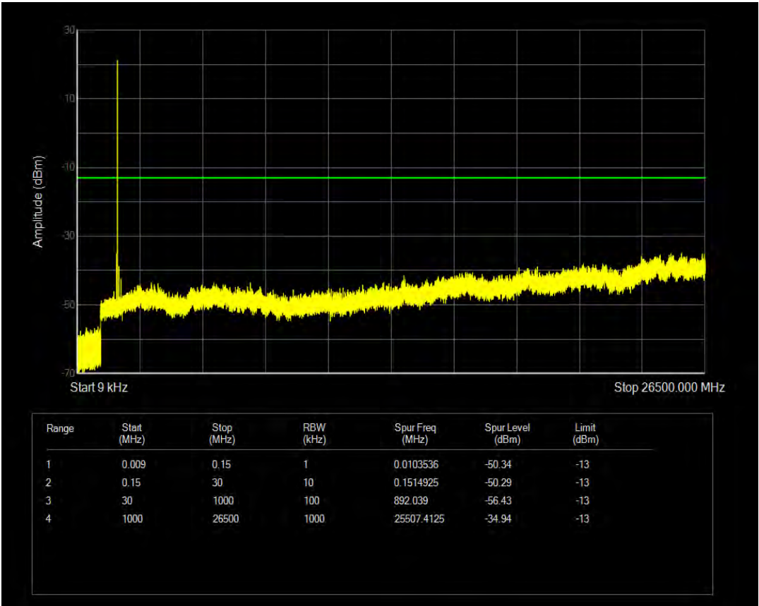
Band66 16QAM BW=10MHz Channel=132022 RB Size=6 Position=#0 NB Index=0
