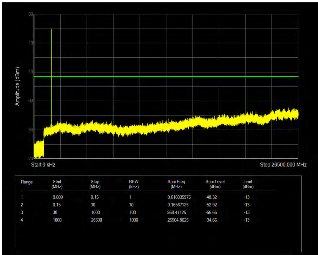
Band66 16QAM BW=1.4MHz Channel=132665 RB Size=6 Position=#0 NB Index=0
