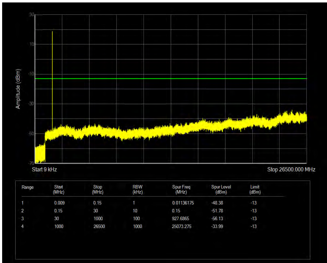
Band66 16QAM BW=1.4MHz Channel=131979 RB Size=6 Position=#0 NB Index=0
