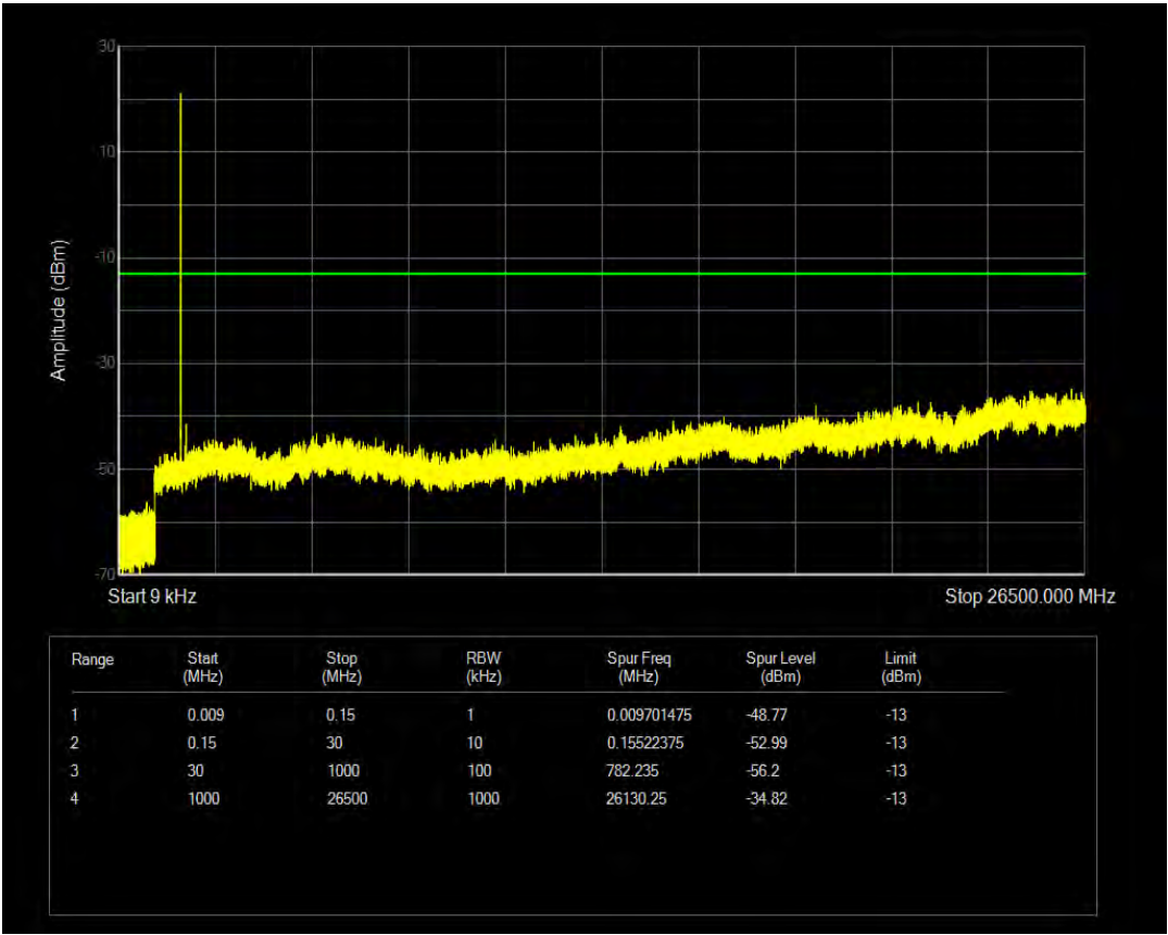
Band4 16QAM BW=10MHz Channel=20000 RB Size=6 Position=#0 NB Index=0
