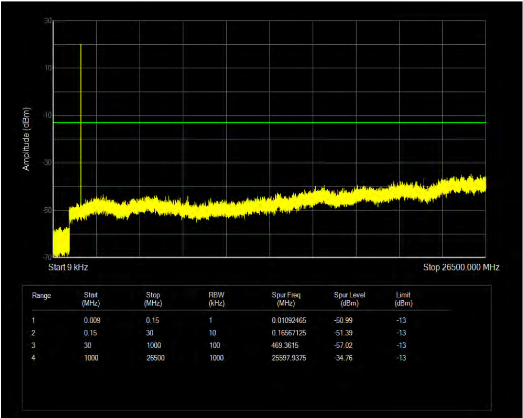
Band66 16QAM BW=5MHz Channel=131997 RB Size=6 Position=#0 NB Index=0
