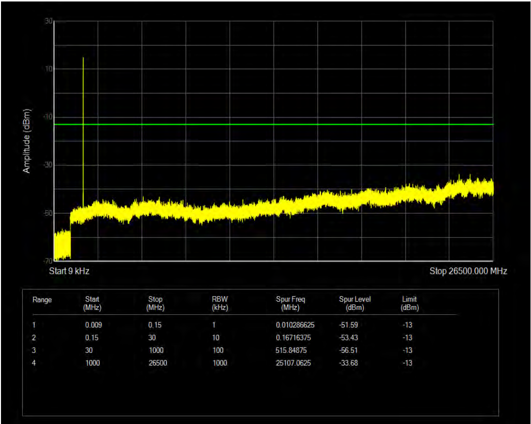
Band66 16QAM BW=3MHz Channel=132657 RB Size=6 Position=#0 NB Index=0
