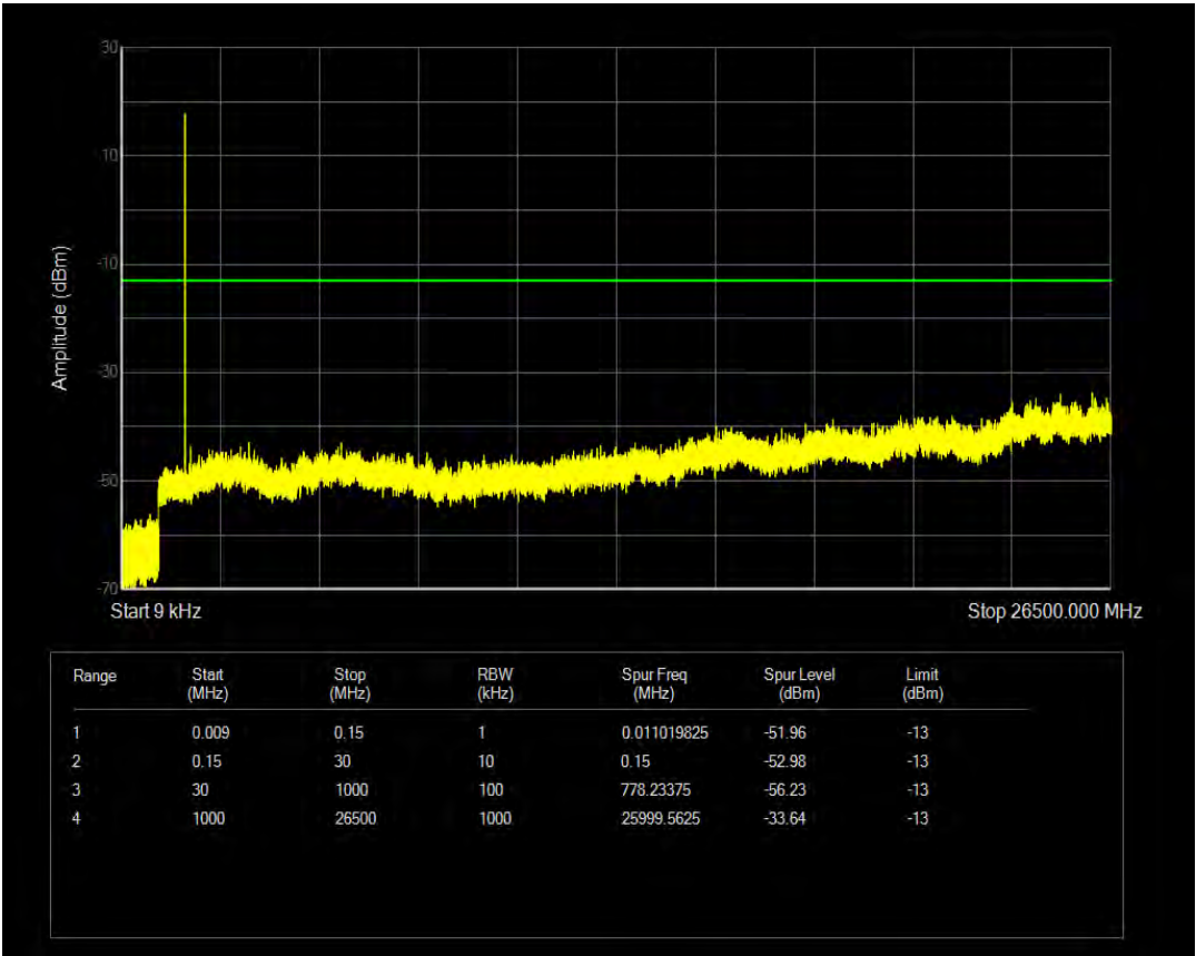
Band66 16QAM BW=15MHz Channel=132047 RB Size=6 Position=#0 NB Index=0
