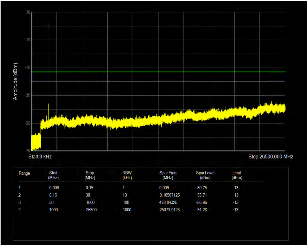
Band66 16QAM BW=20MHz Channel=132572 RB Size=6 Position=#0 NB Index=0
