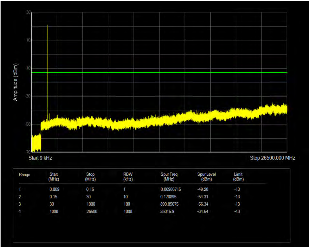
Band66 16QAM BW=20MHz Channel=132072 RB Size=6 Position=#0 NB Index=0
