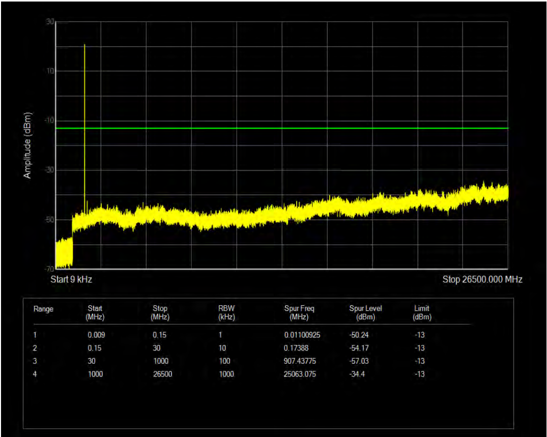
Band4 16QAM BW=5MHz Channel=19975 RB Size=6 Position=#0 NB Index=0
