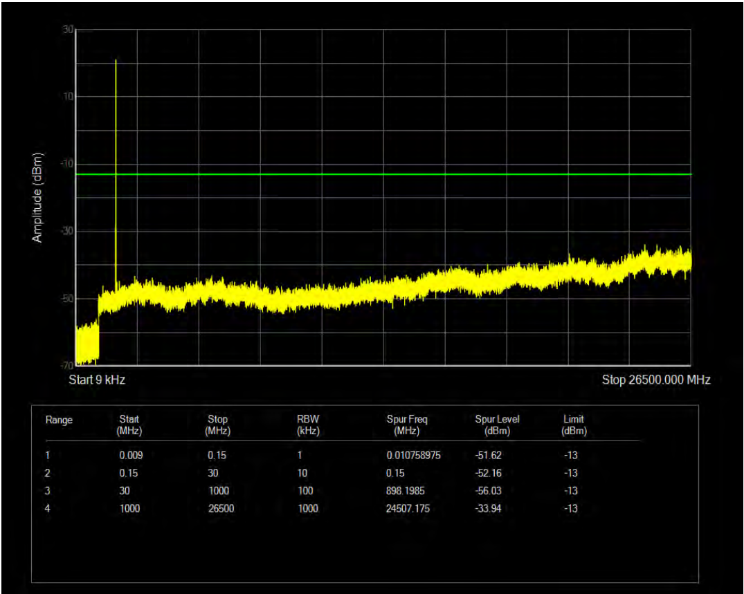
Band4 16QAM BW=15MHz Channel=20325 RB Size=6 Position=#0 NB Index=0
