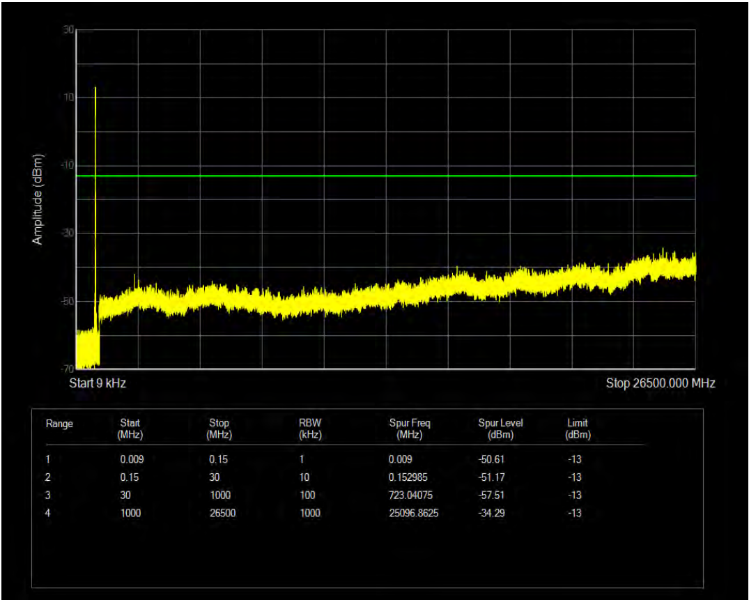
Band26(824-849) QPSK BW=3MHz Channel=26805 RB Size=1 Position=#0 NB Index=0
