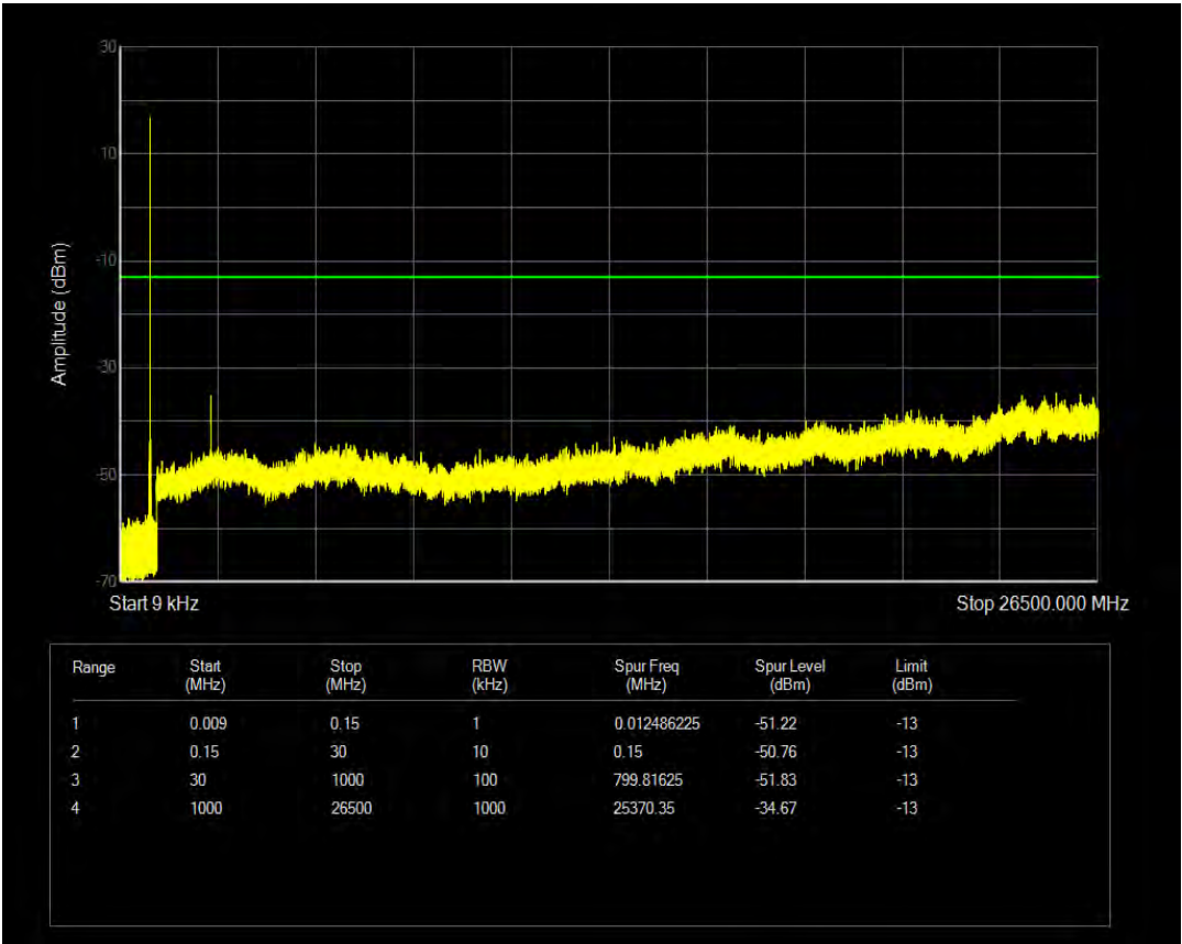
Band5 16QAM BW=5MHz Channel=20425 RB Size=6 Position=#0 NB Index=0
