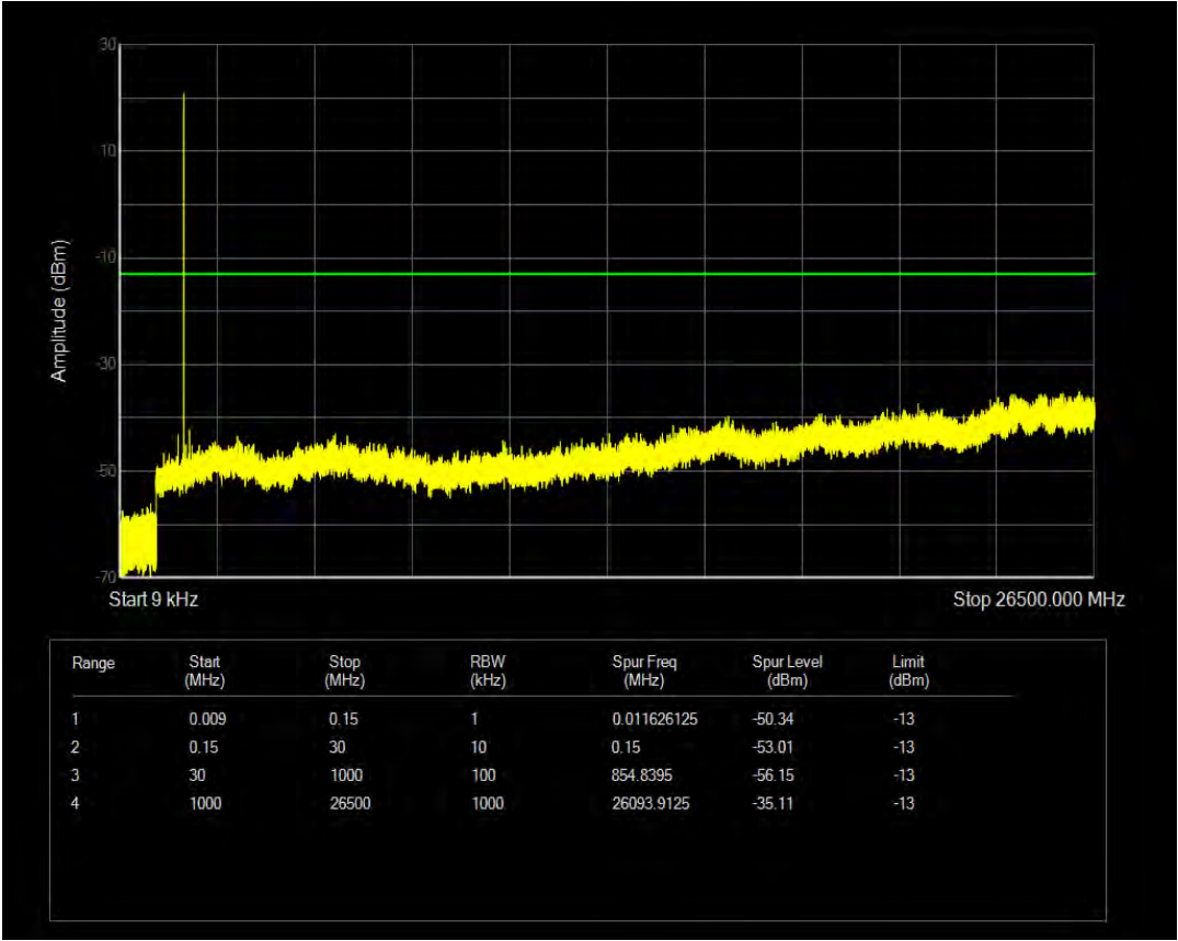
Band4 16QAM BW=1.4MHz Channel=20393 RB Size=6 Position=#0 NB Index=0
