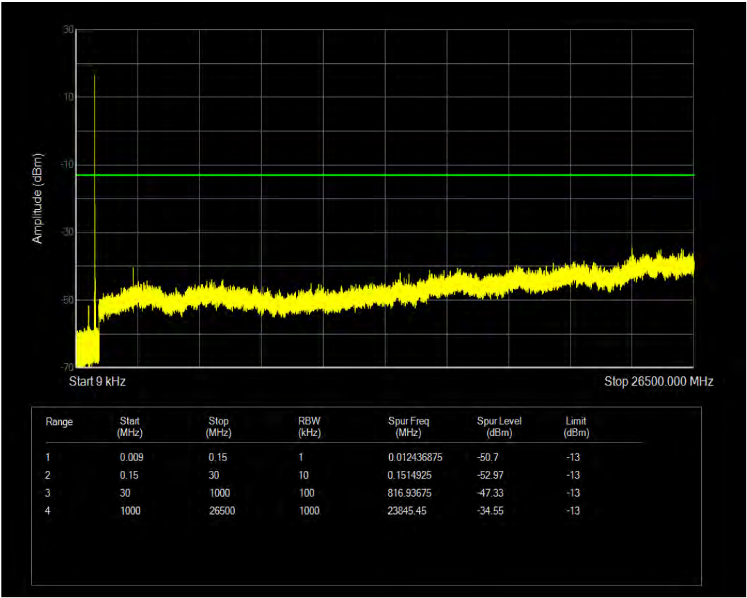
Band5 16QAM BW=1.4MHz Channel=20407 RB Size=6 Position=#0 NB Index=0
