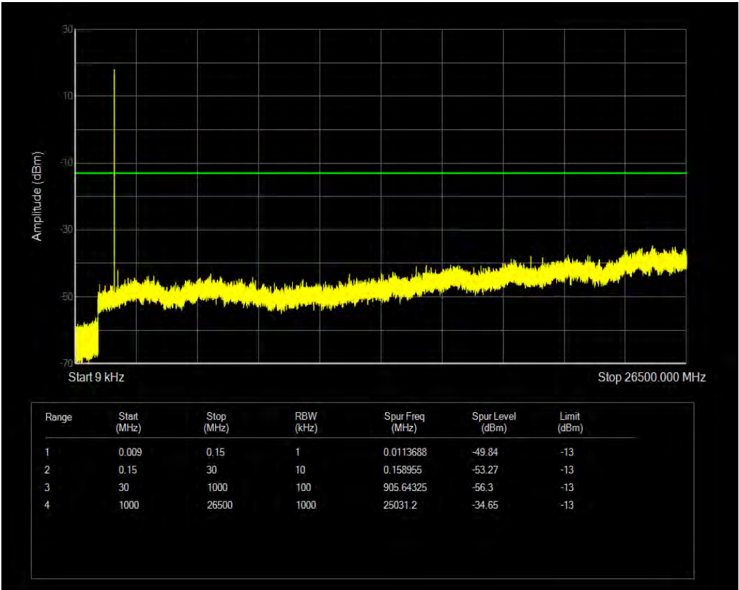
Band66 16QAM BW=3MHz Channel=131987 RB Size=6 Position=#0 NB Index=0
