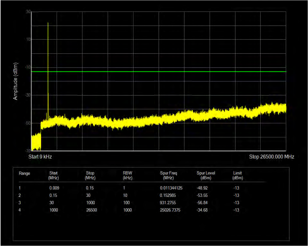
Band4 16QAM BW=10MHz Channel=20350 RB Size=6 Position=#0 NB Index=0
