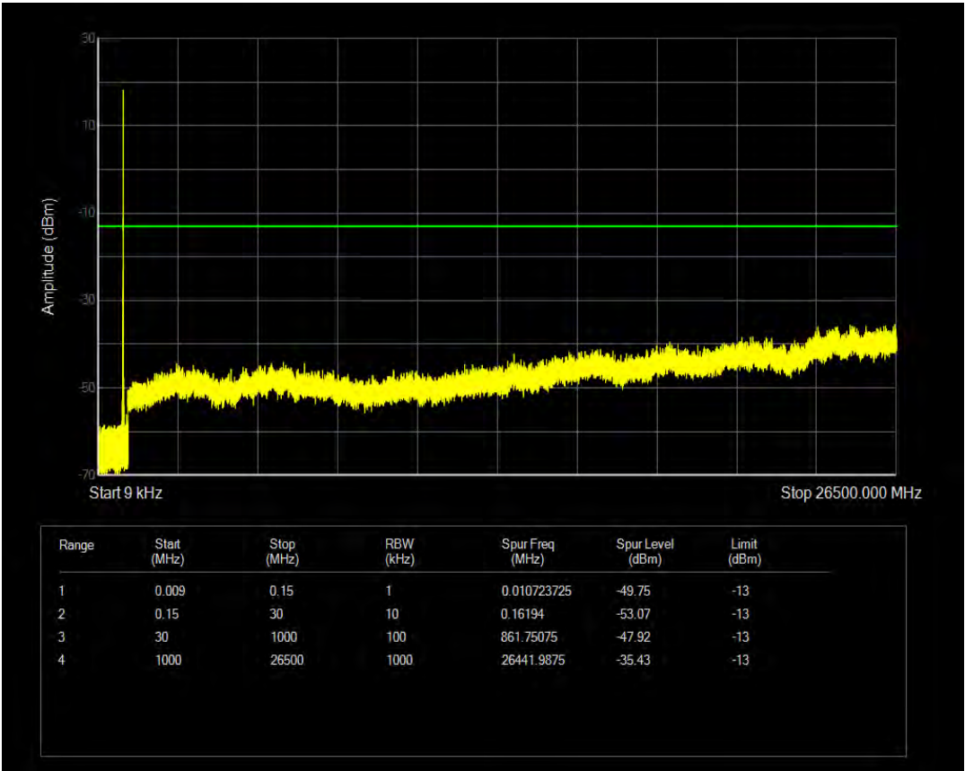
Band5 16QAM BW=3MHz Channel=20635 RB Size=6 Position=#0 NB Index=0
