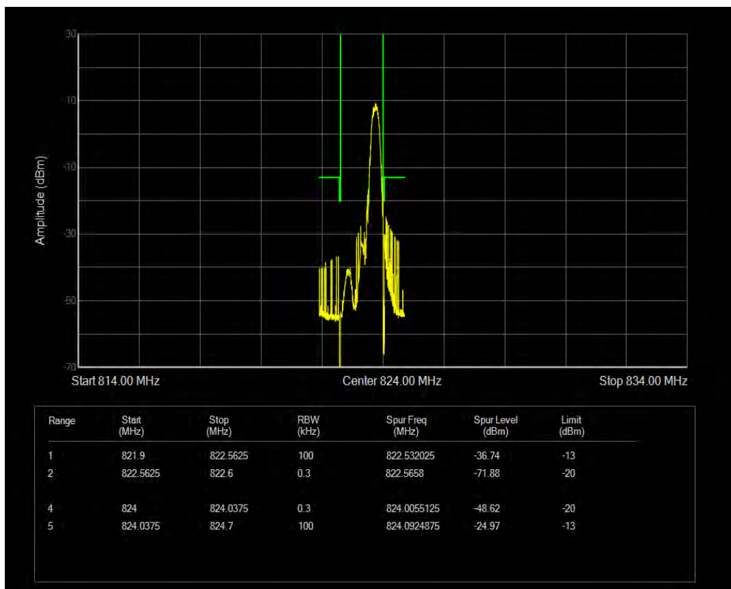
Band26(814-824) 16QAM BW=1.4MHz Channel=26783 RB Size=6 Position=#Max NB Index=0
