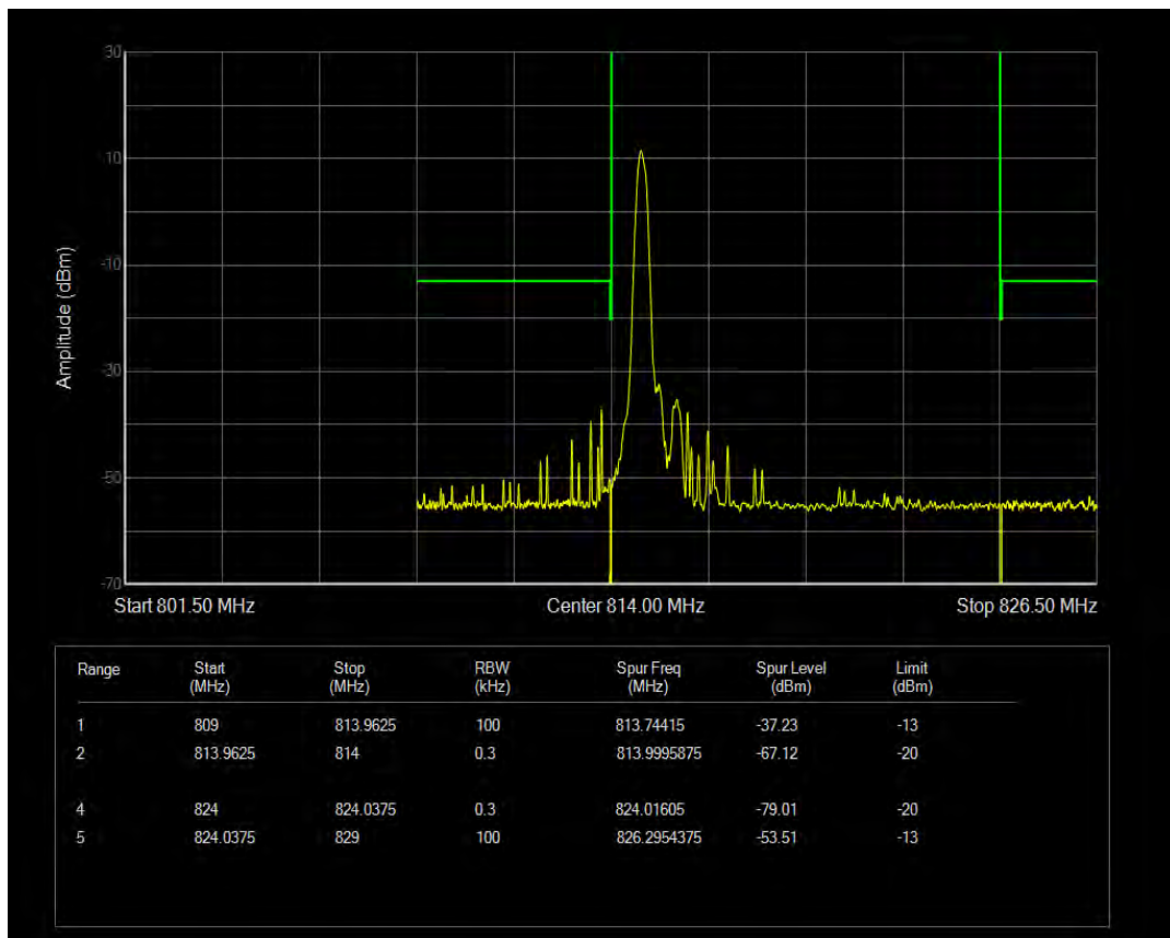
Band26(814-824) QPSK BW=10MHz Channel=26740 RB Size=4 Position=#0 NB Index=0
