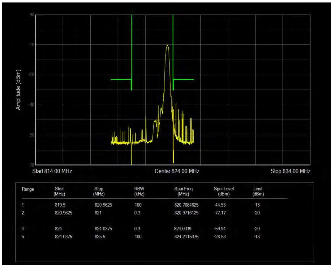
Band26(814-824) QPSK BW=3MHz Channel=26775 RB Size=6 Position=#Max NB Index=1
