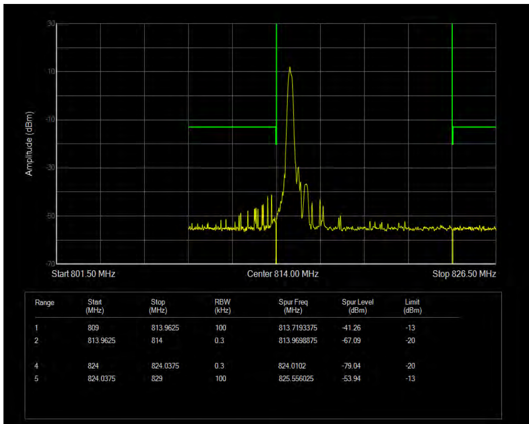
Band26(814-824) 16QAM BW=10MHz Channel=26740 RB Size=4 Position=#0 NB Index=0
