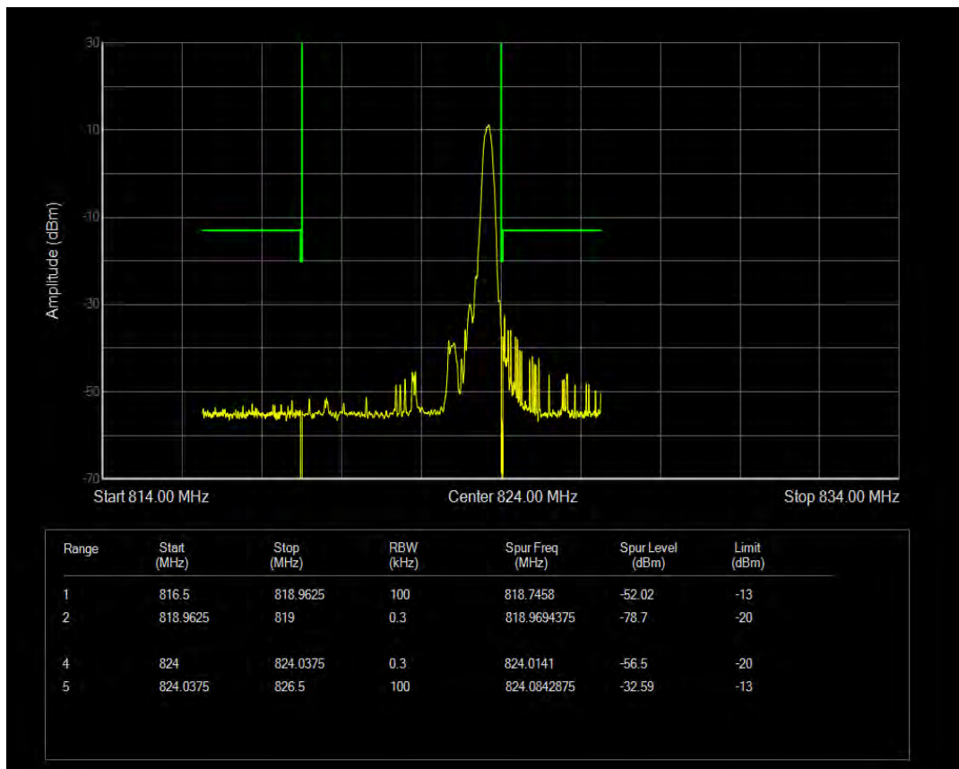
Band26(814-824) 16QAM BW=5MHz Channel=26765 RB Size=6 Position=#Max NB Index=3
