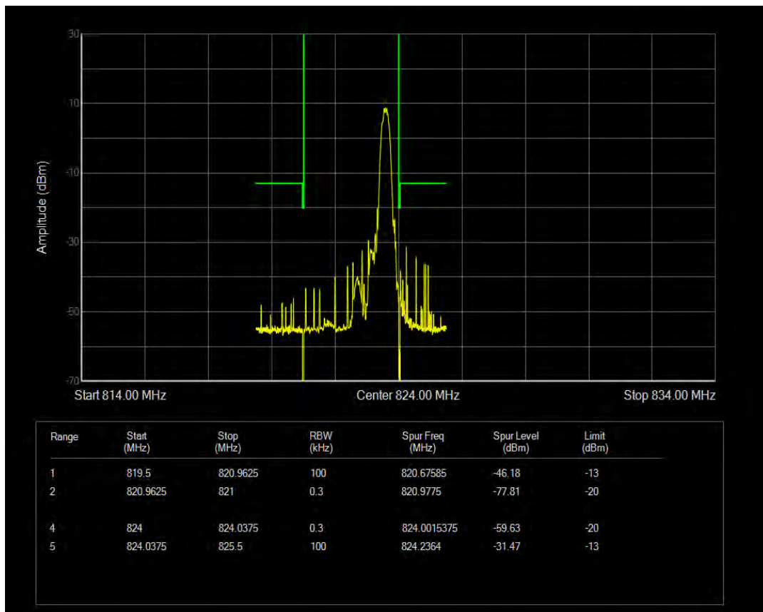
Band26(814-824) 16QAM BW=3MHz Channel=26775 RB Size=6 Position=#Max NB Index=1
