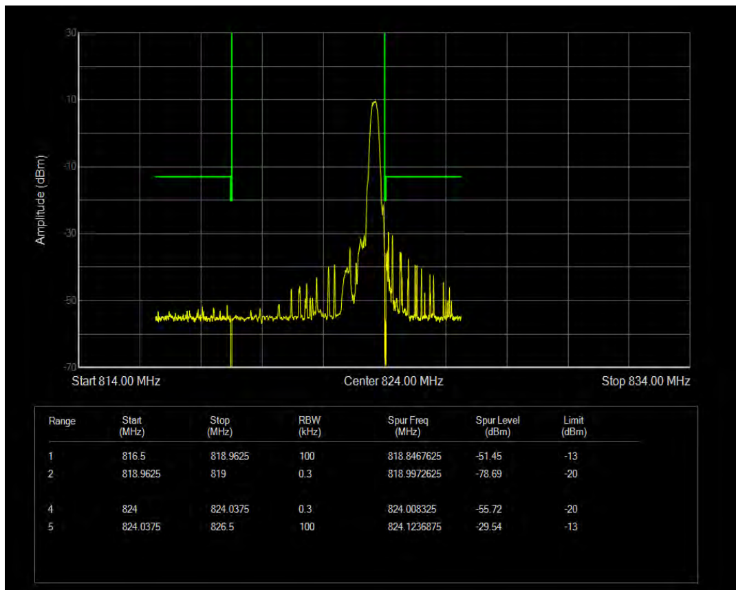
Band26(814-824) QPSK BW=5MHz Channel=26765 RB Size=6 Position=#Max NB Index=3
