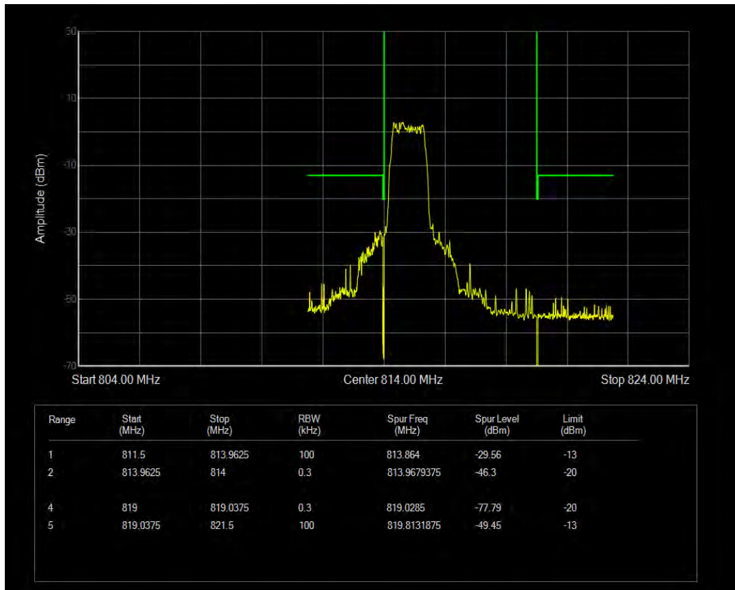
Band26(814-824) 16QAM BW=5MHz Channel=26765 RB Size=1 Position=#Max NB Index=3
