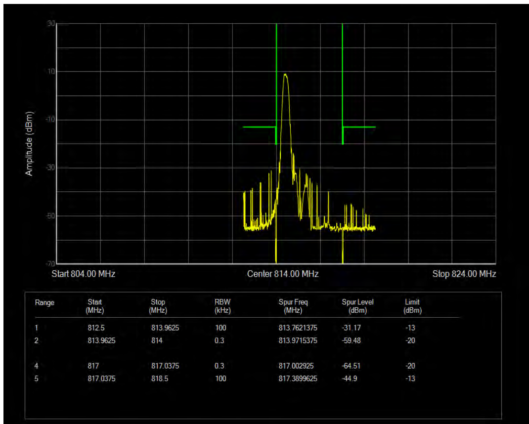
Band26(814-824) 16QAM BW=3MHz Channel=26705 RB Size=6 Position=#0 NB Index=0
