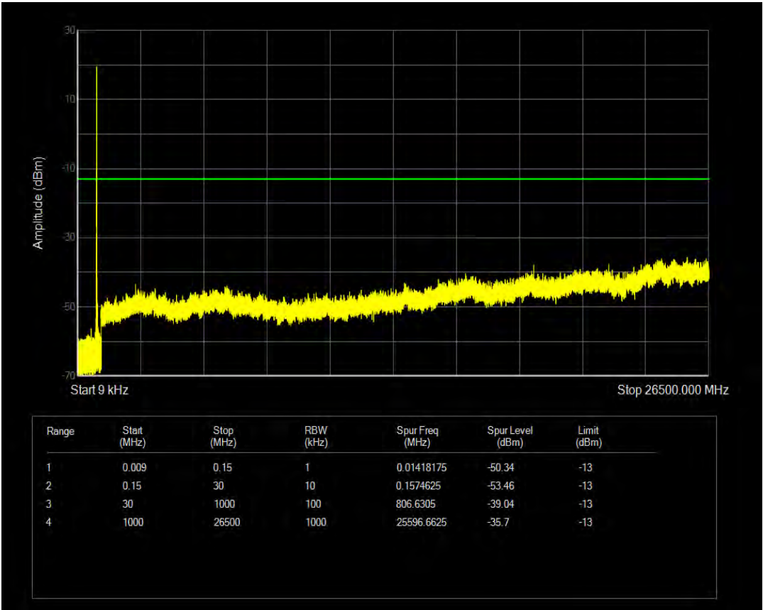
Band26(814-824) 16QAM BW=1.4MHz Channel=26697 RB Size=6 Position=#0 NB Index=0
