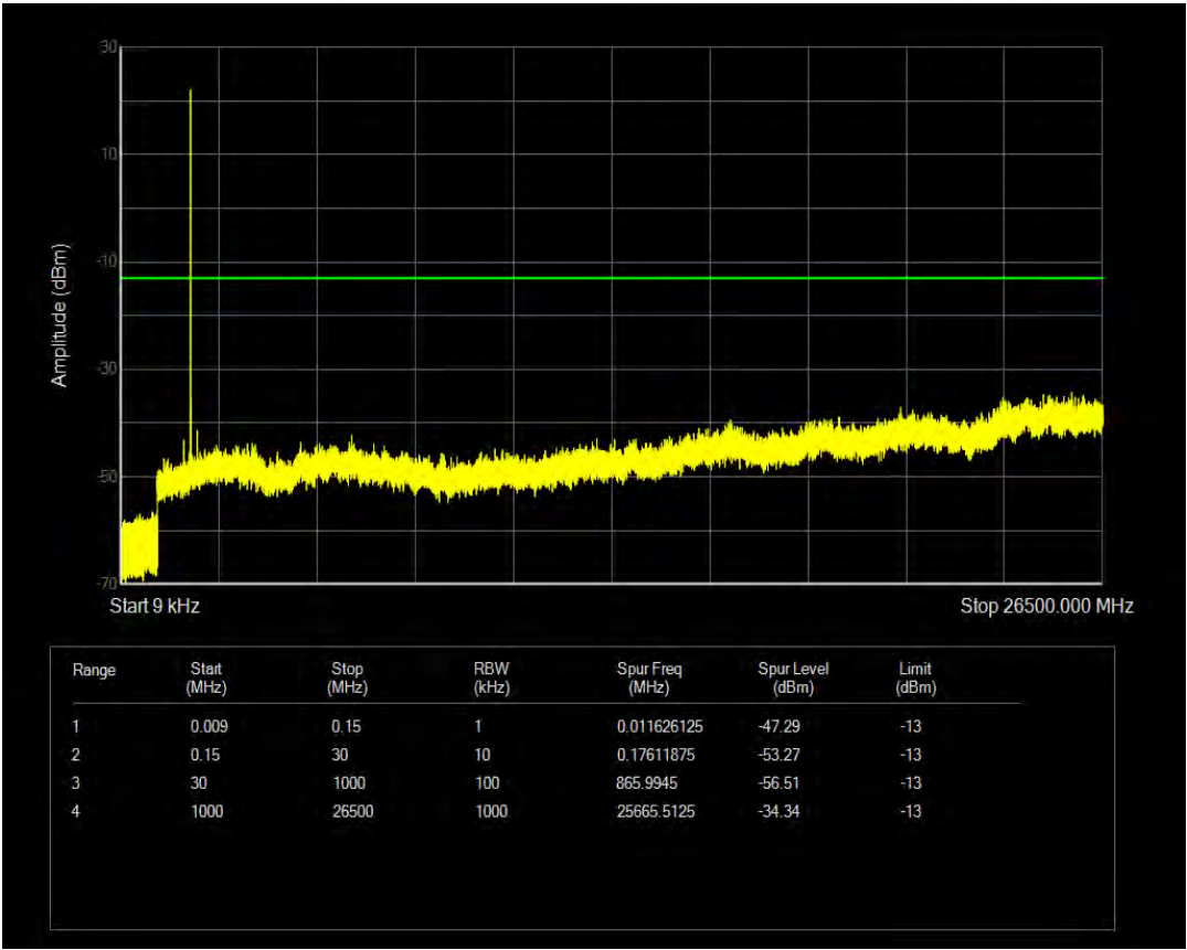
Band25 16QAM BW=20MHz Channel=26590 RB Size=6 Position=#0 NB Index=0
