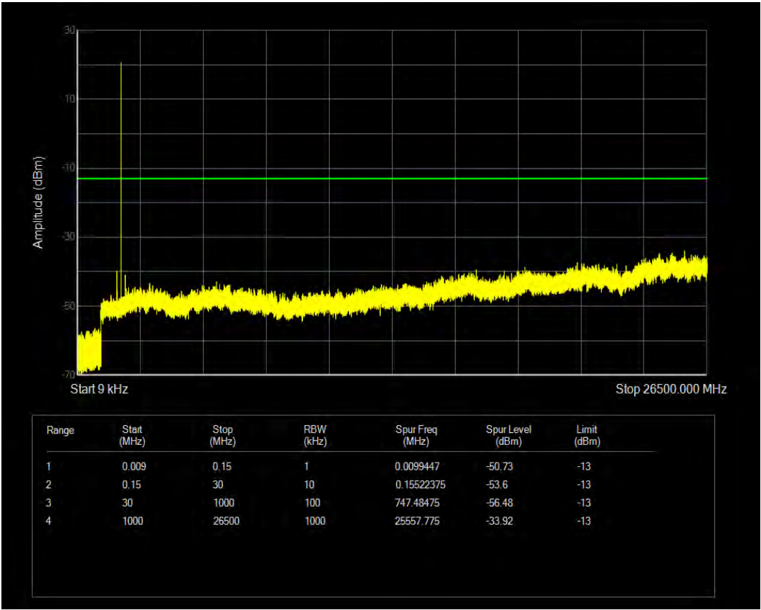
Band25 16QAM BW=10MHz Channel=26090 RB Size=6 Position=#0 NB Index=0
