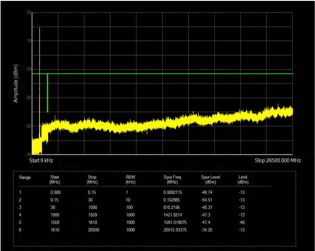
Band13 16QAM BW=5MHz Channel=23255 RB Size=6 Position=#0 NB Index=0
