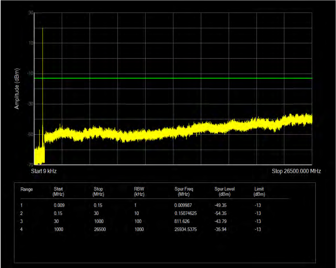
Band26(824-849) QPSK BW=1.4MHz Channel=26797 RB Size=6 Position=#0 NB Index=0
