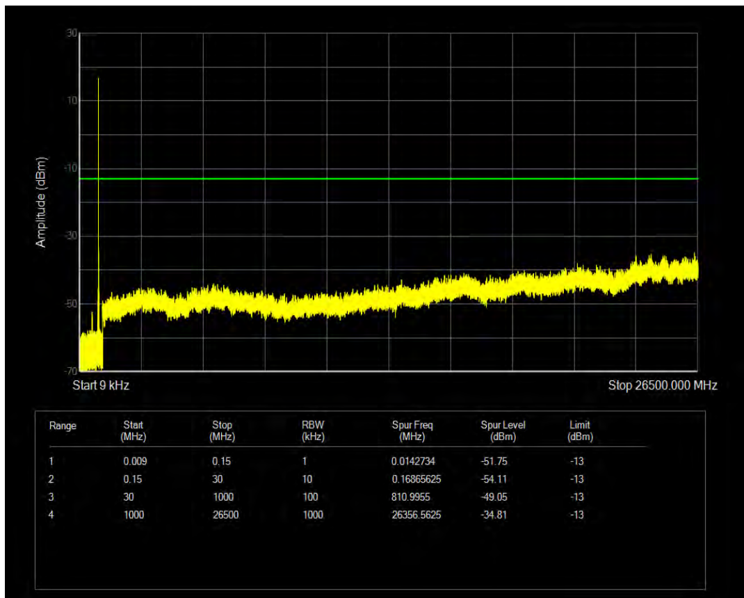
Band26(824-849) 16QAM BW=3MHz Channel=26805 RB Size=6 Position=#0 NB Index=0
