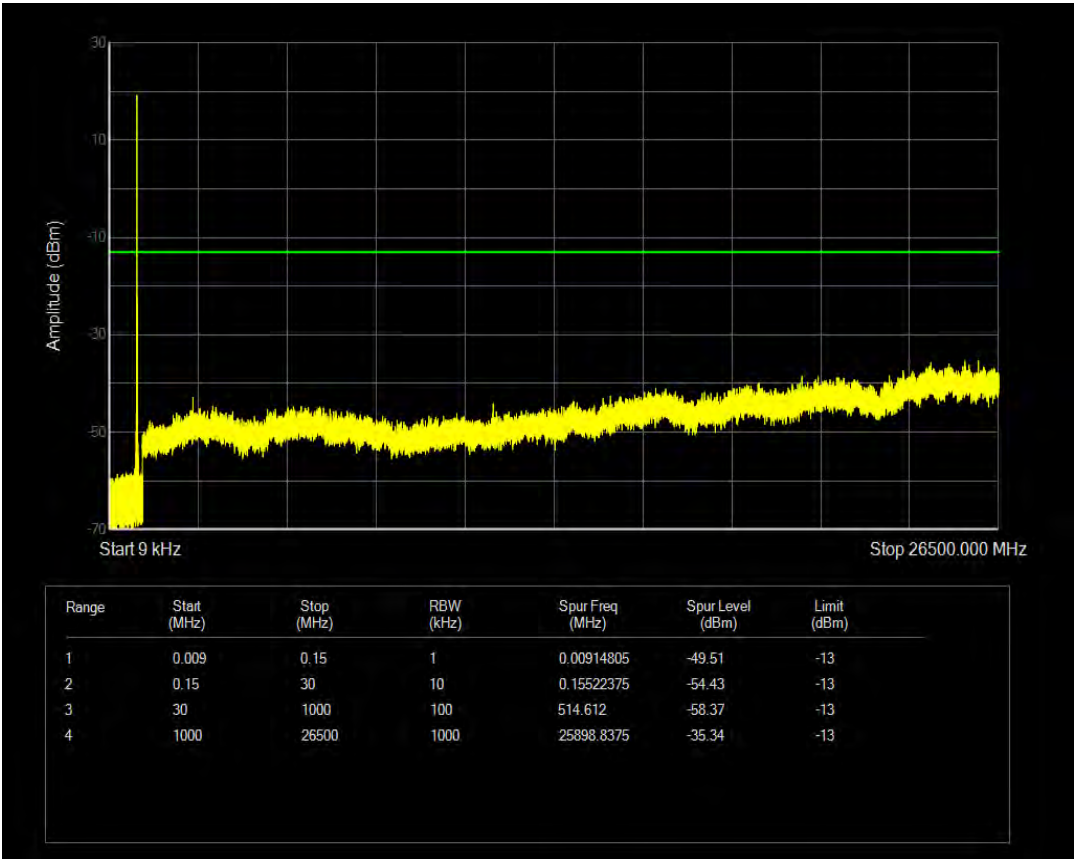
Band26(824-849) 16QAM BW=15MHz Channel=26965 RB Size=6 Position=#0 NB Index=0
