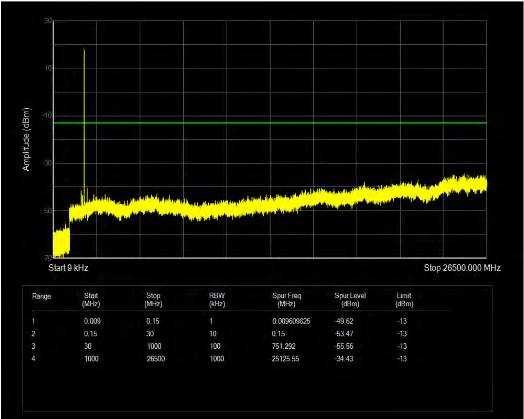
Band25 16QAM BW=15MHz Channel=26615 RB Size=6 Position=#0 NB Index=0
