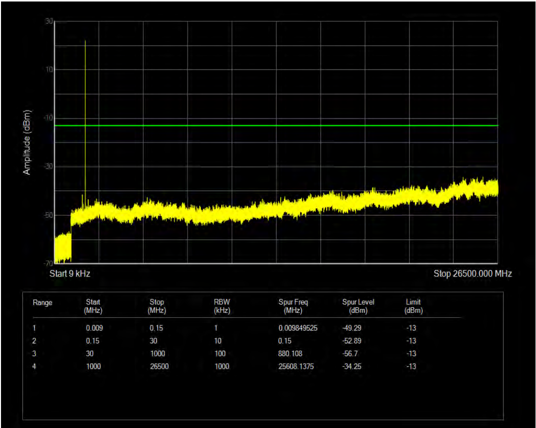
Band25 16QAM BW=20MHz Channel=26140 RB Size=6 Position=#0 NB Index=0
