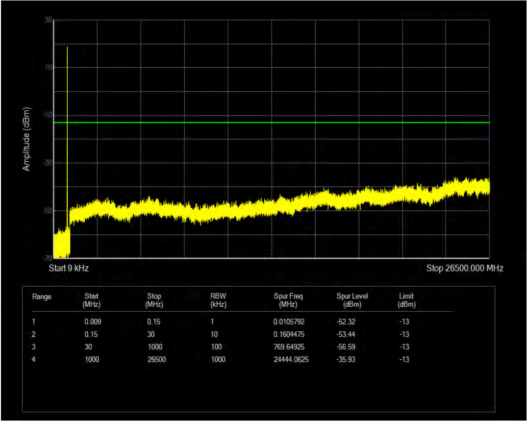
Band26(824-849) 16QAM BW=3MHz Channel=27025 RB Size=6 Position=#0 NB Index=0
