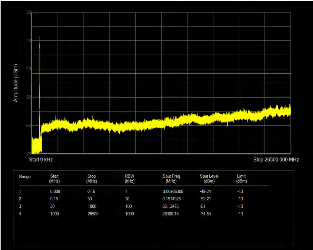
Band26(814-824) QPSK BW=5MHz Channel=26715 RB Size=1 Position=#0 NB Index=0
