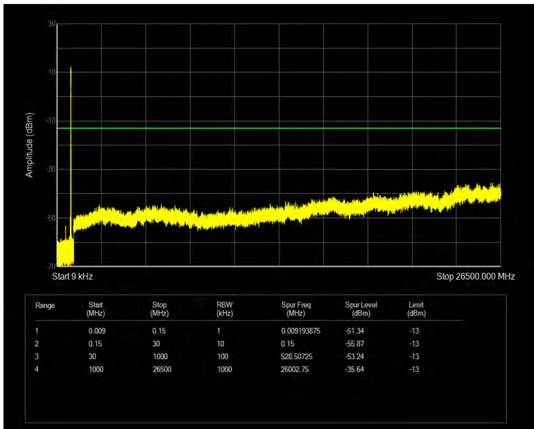
Band26(824-849) 16QAM BW=3MHz Channel=26805 RB Size=1 Position=#0 NB Index=0
