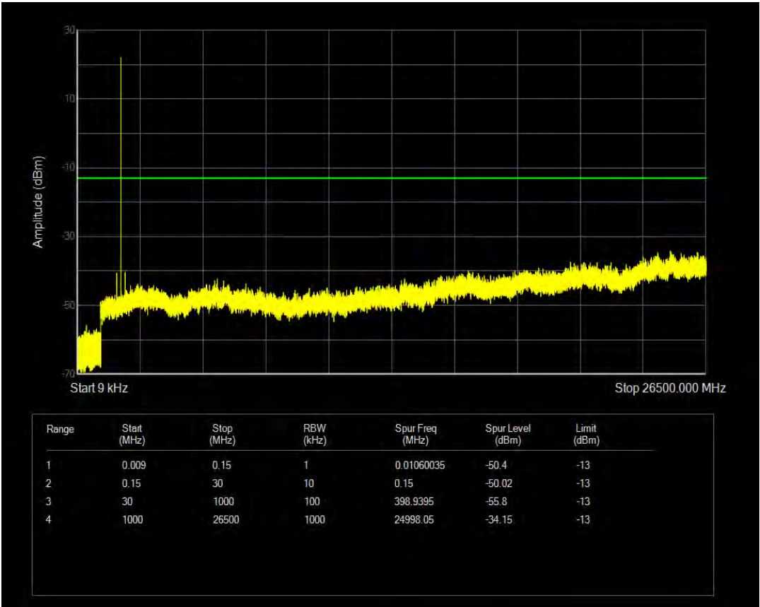
Band25 16QAM BW=5MHz Channel=26065 RB Size=6 Position=#0 NB Index=0
