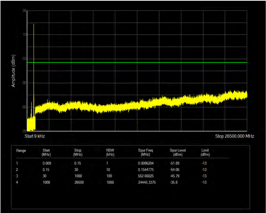
Band26(814-824) 16QAM BW=3MHz Channel=26775 RB Size=6 Position=#0 NB Index=0
