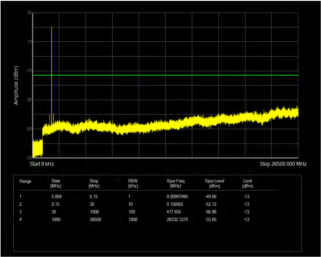
Band25 16QAM BW=10MHz Channel=26640 RB Size=6 Position=#0 NB Index=0
