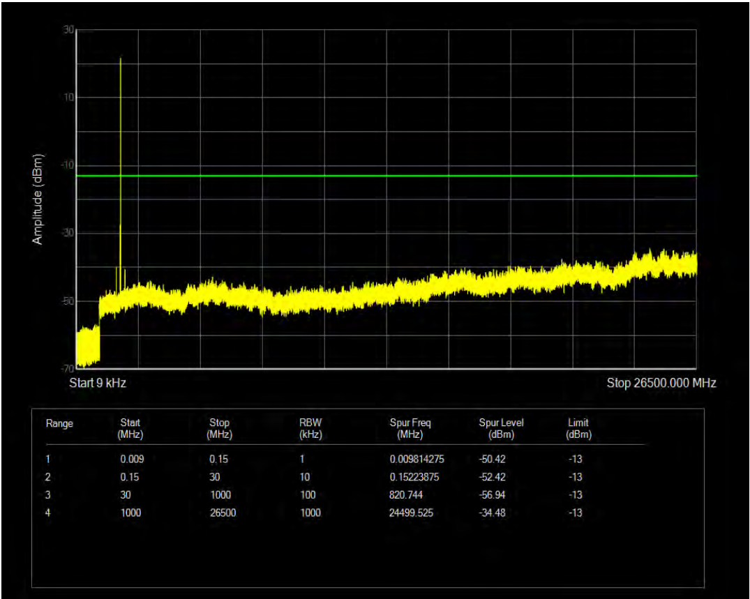
Band2 16QAM BW=3MHz Channel=19185 RB Size=6 Position=#0 NB Index=0
