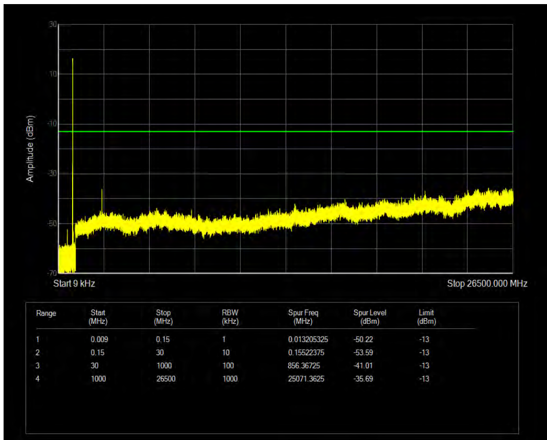
Band26(824-849) 16QAM BW=1.4MHz Channel=27033 RB Size=6 Position=#0 NB Index=0
