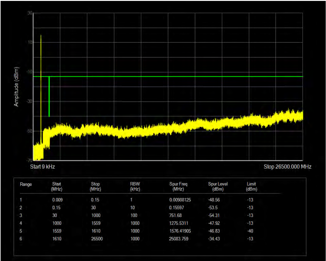
Band13 16QAM BW=5MHz Channel=23255 RB Size=1 Position=#0 NB Index=0
