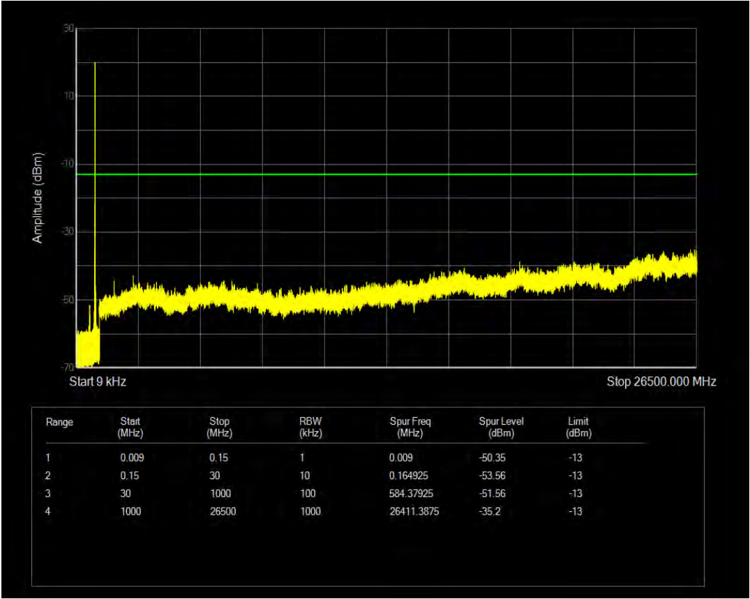
Band26(814-824) 16QAM BW=10MHz Channel=26740 RB Size=6 Position=#0 NB Index=0
