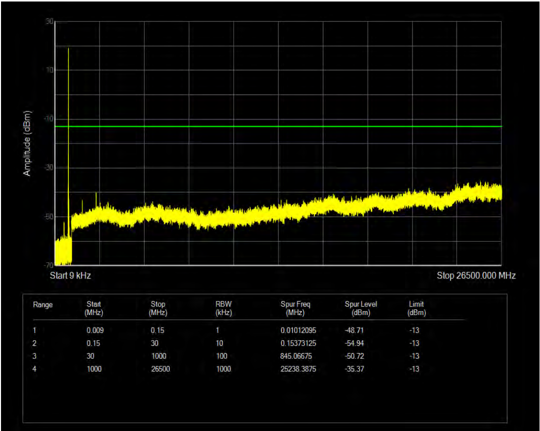
Band26(814-824) 16QAM BW=5MHz Channel=26765 RB Size=6 Position=#0 NB Index=0
