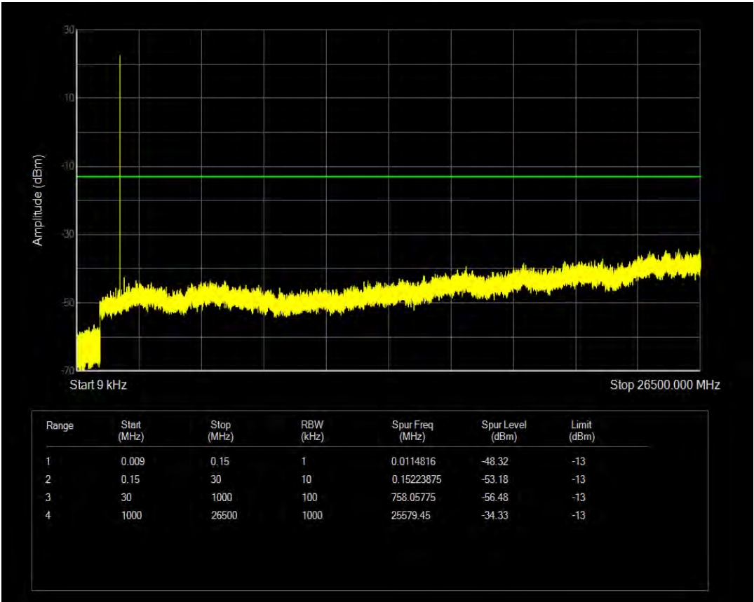
Band25 16QAM BW=3MHz Channel=26055 RB Size=6 Position=#0 NB Index=0
