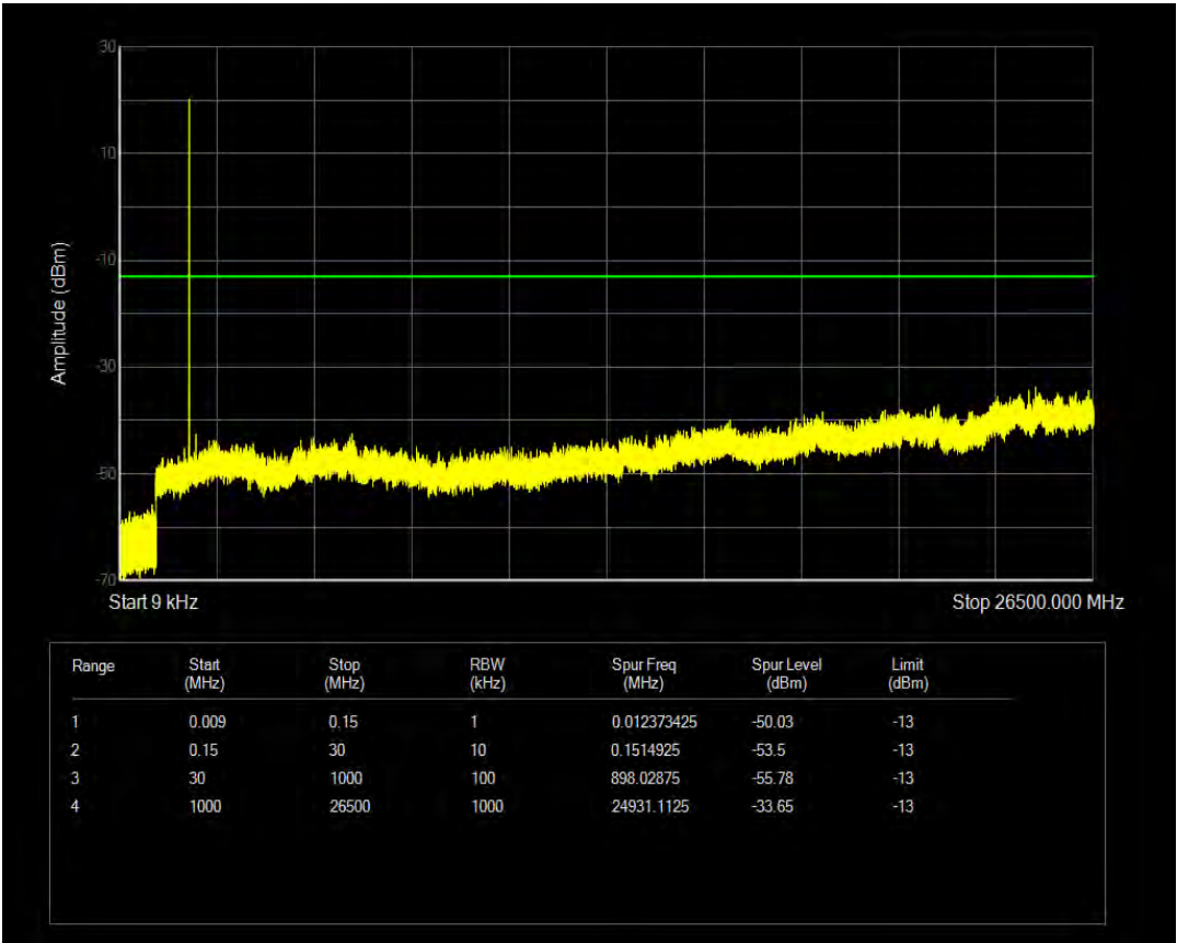
Band25 16QAM BW=15MHz Channel=26115 RB Size=1 Position=#0 NB Index=0
