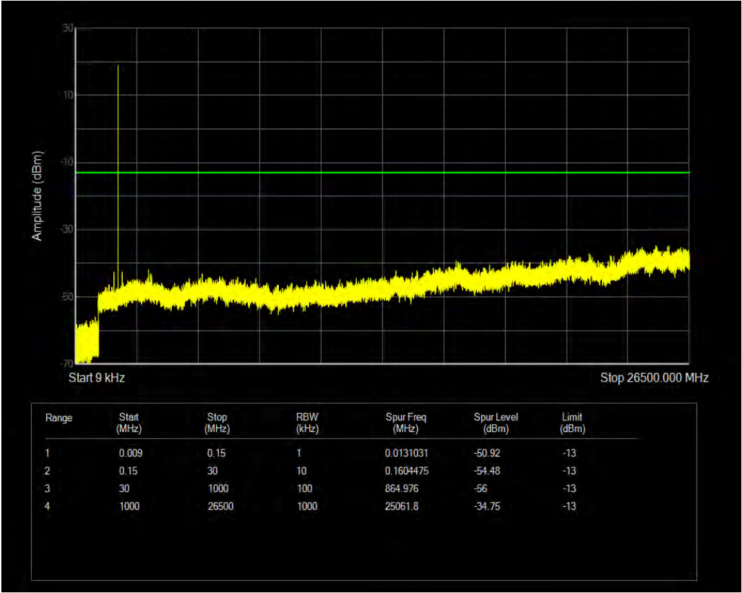
Band2 16QAM BW=10MHz Channel=18650 RB Size=6 Position=#0 NB Index=0
