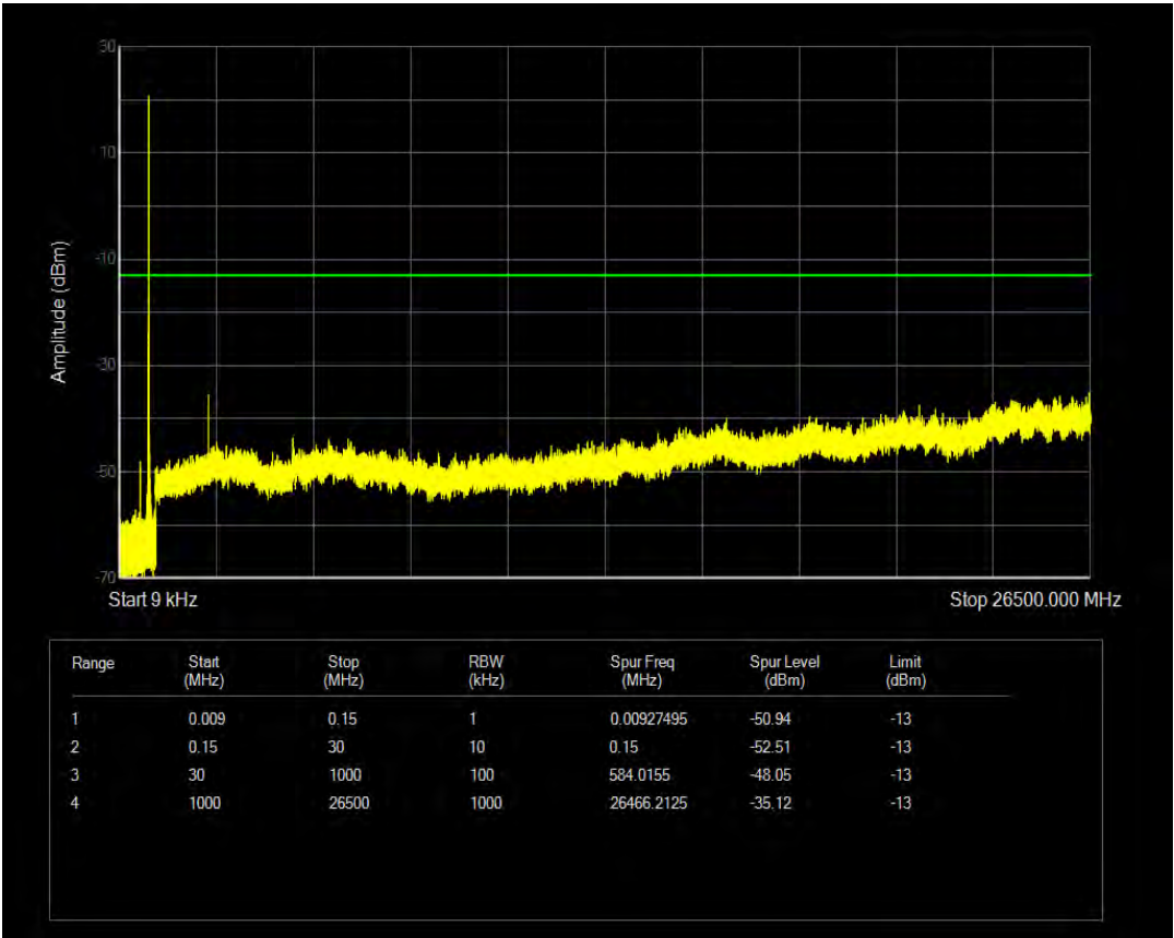
Band26(814-824) 16QAM BW=5MHz Channel=26715 RB Size=6 Position=#0 NB Index=0
