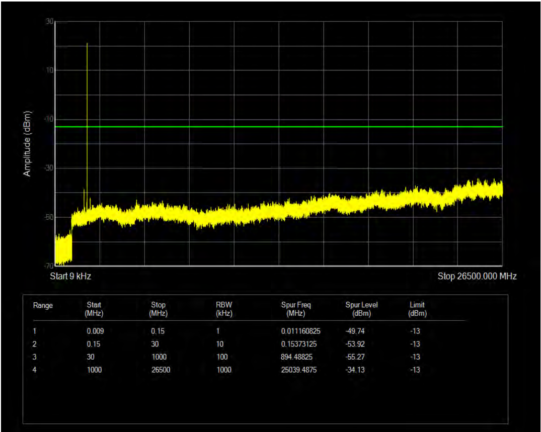
Band25 16QAM BW=3MHz Channel=26675 RB Size=6 Position=#0 NB Index=0
