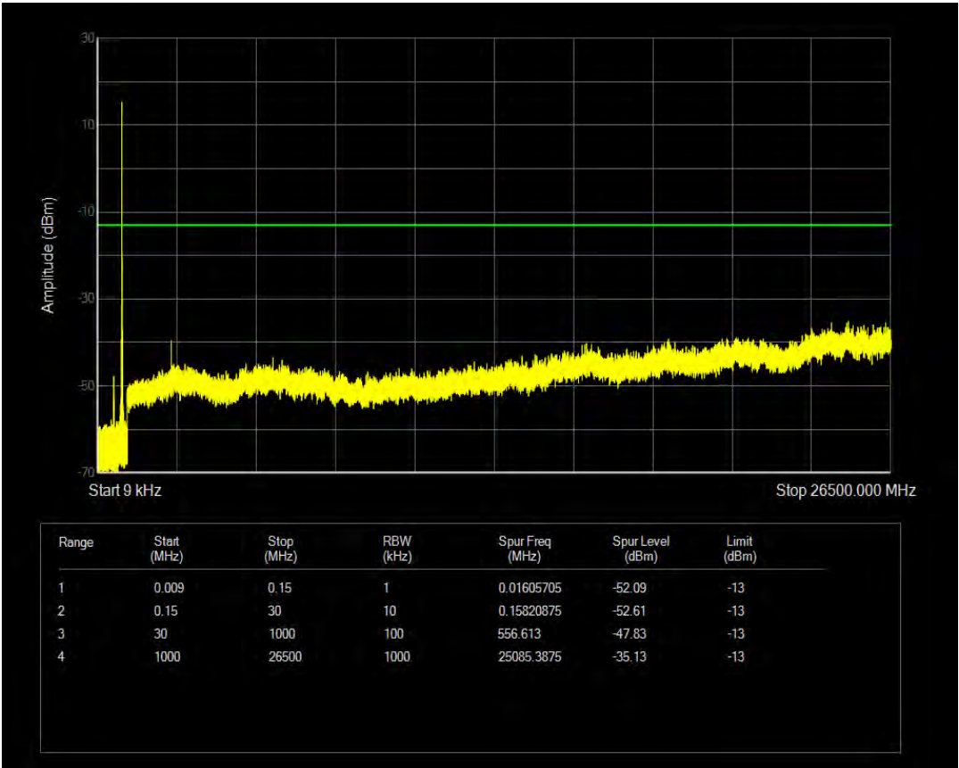
Band26(824-849) 16QAM BW=15MHz Channel=26965 RB Size=1 Position=#0 NB Index=0
