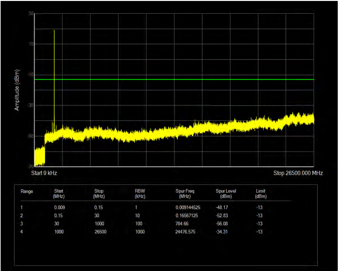
Band25 16QAM BW=3MHz Channel=26055 RB Size=1 Position=#0 NB Index=0
