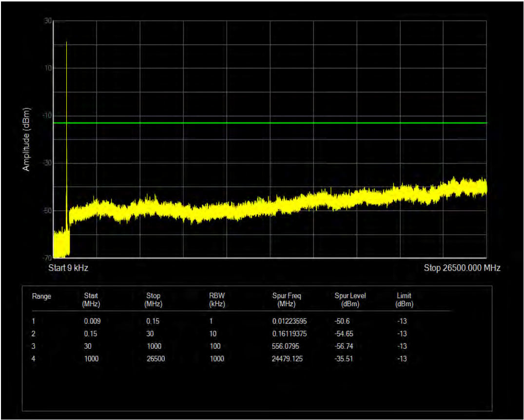
Band26(824-849) 16QAM BW=15MHz Channel=26865 RB Size=6 Position=#0 NB Index=0
