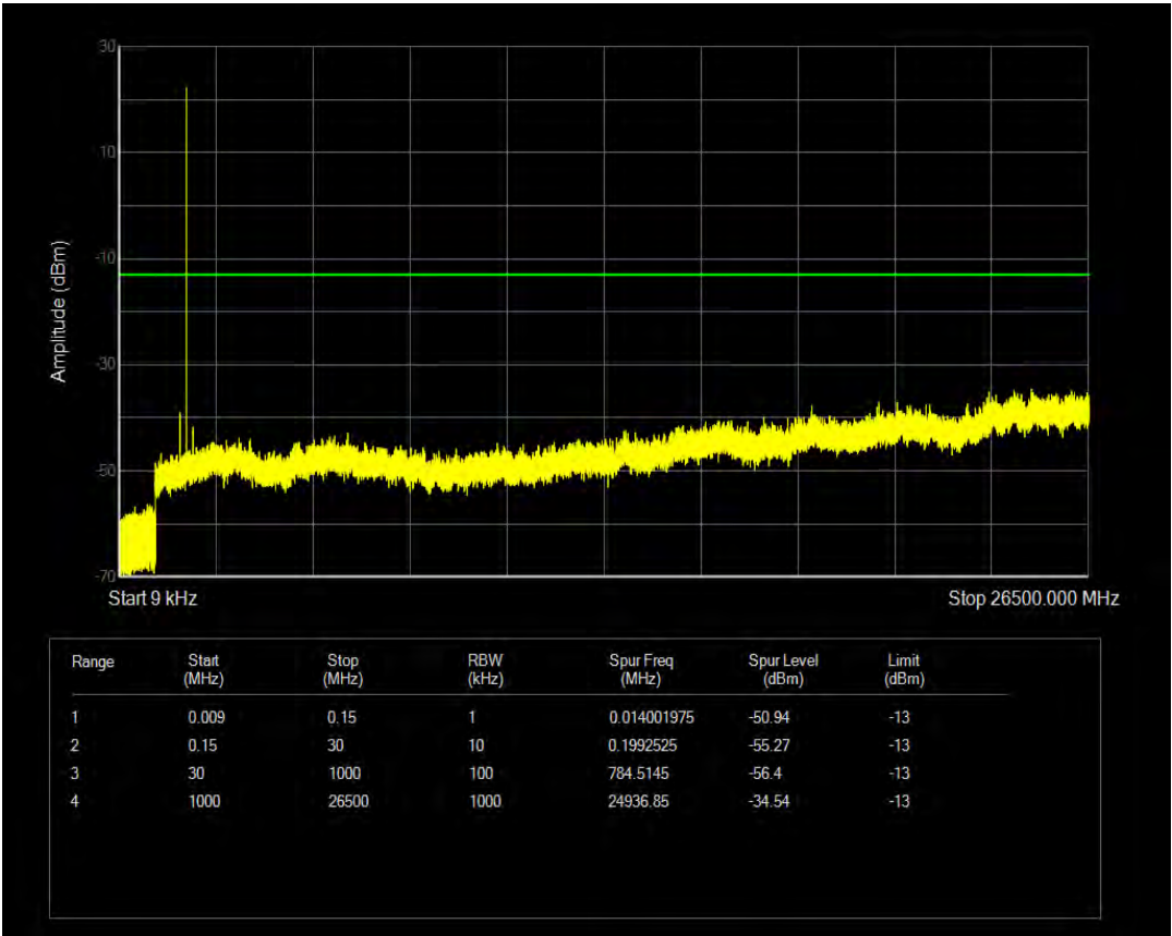
Band25 16QAM BW=15MHz Channel=26115 RB Size=6 Position=#0 NB Index=0
