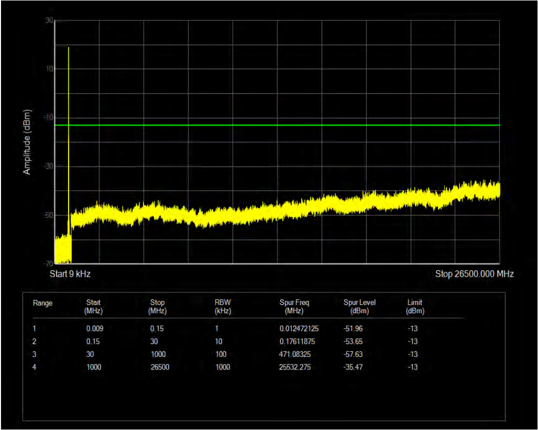
Band26(824-849) 16QAM BW=10MHz Channel=26990 RB Size=6 Position=#0 NB Index=0
