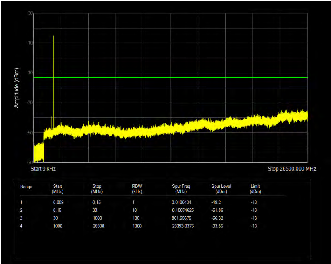
Band25 16QAM BW=5MHz Channel=26665 RB Size=6 Position=#0 NB Index=0
