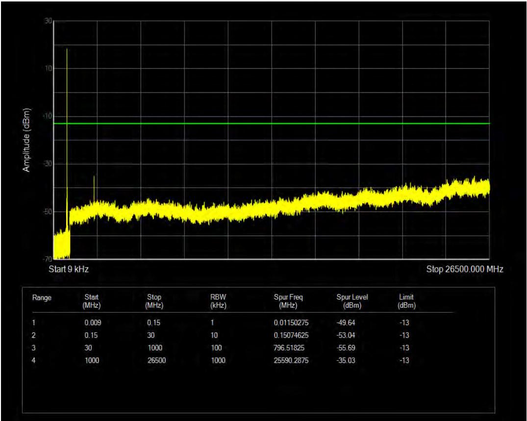
Band26(824-849) 16QAM BW=5MHz Channel=26815 RB Size=6 Position=#0 NB Index=0
