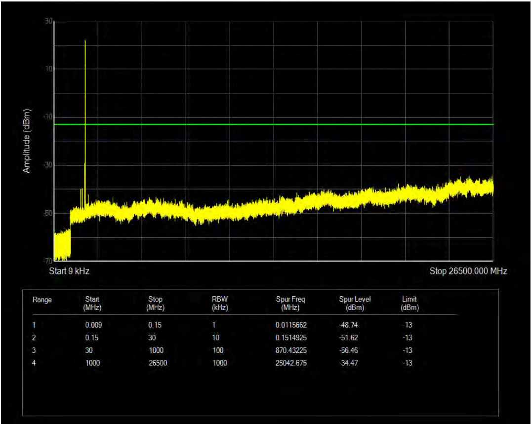
Band2 16QAM BW=15MHz Channel=19125 RB Size=6 Position=#0 NB Index=0
