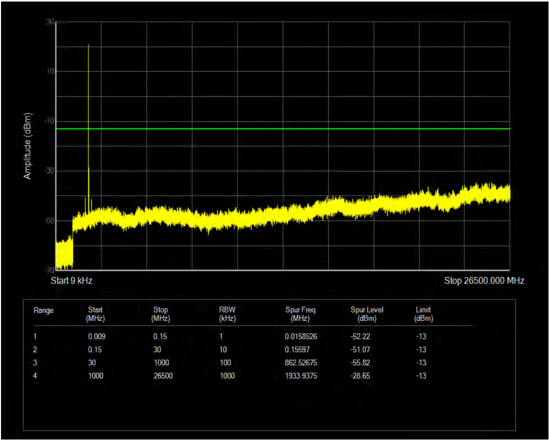
Band25 16QAM BW=1.4MHz Channel=26683 RB Size=6 Position=#0 NB Index=0
