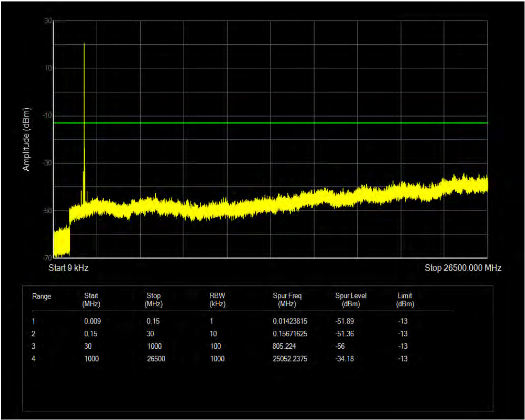
Band2 16QAM BW=20MHz Channel=19100 RB Size=6 Position=#0 NB Index=0
