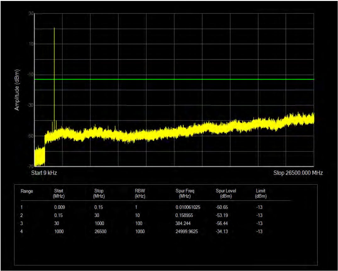
Band2 16QAM BW=10MHz Channel=19150 RB Size=6 Position=#0 NB Index=0
