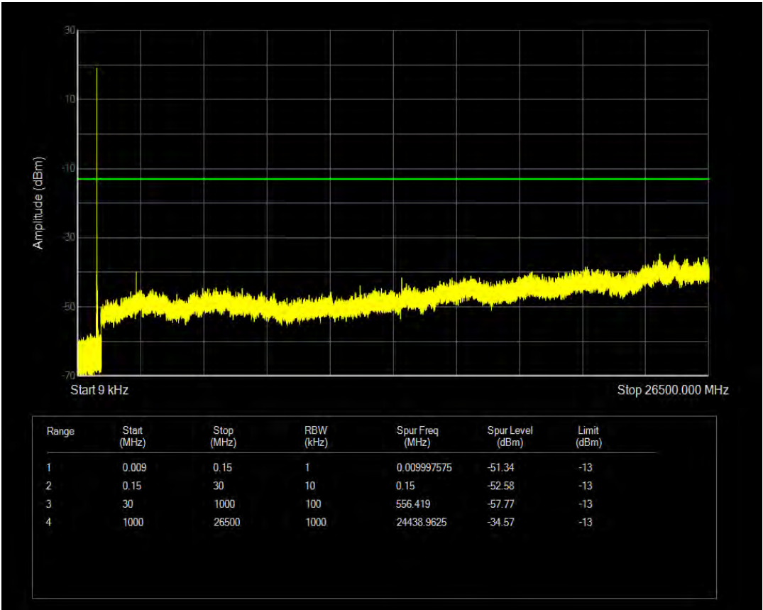
Band26(824-849) 16QAM BW=10MHz Channel=26840 RB Size=6 Position=#0 NB Index=0
