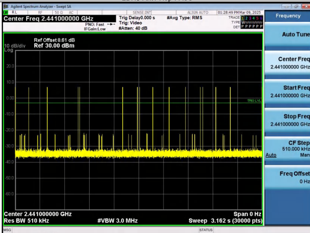
2DH3-Ant1-Hop-PASS
