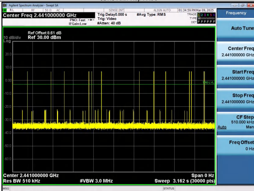
3DH3-Ant1-Hop-PASS
