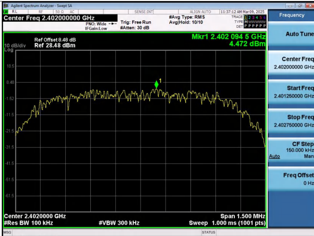
3DH5-Ant1-2402-0~Reference-PASS
