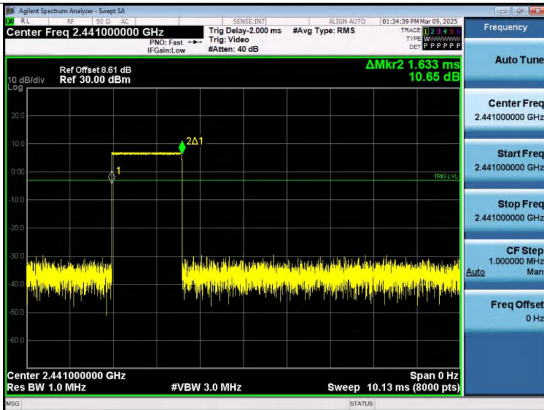
3DH3-Ant1-Hop-PASS
