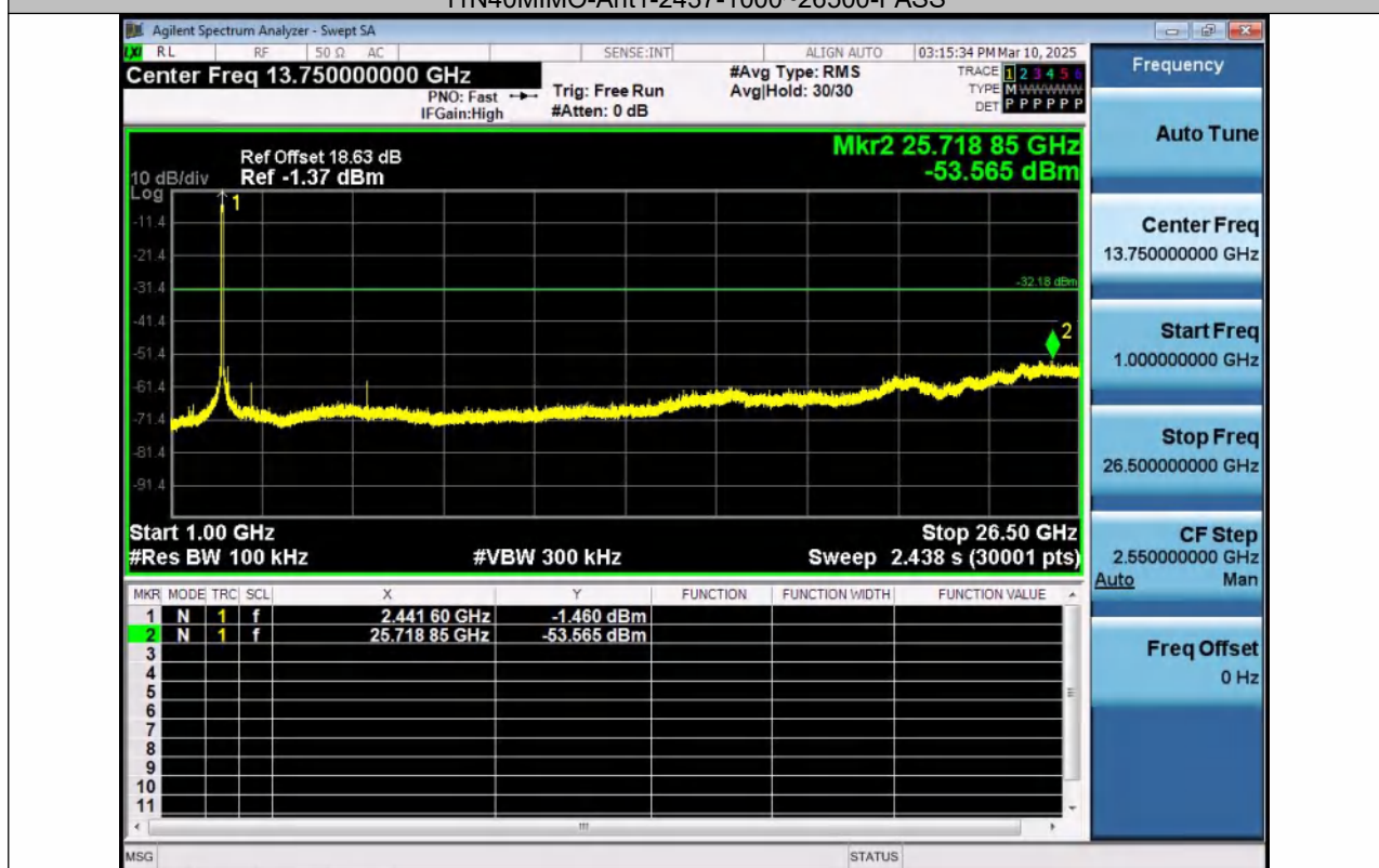
11N40MIMO-Ant2-2437-1000~26500-PASS
