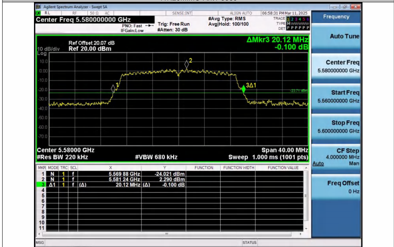
11N20MIMO-Ant2-5580
