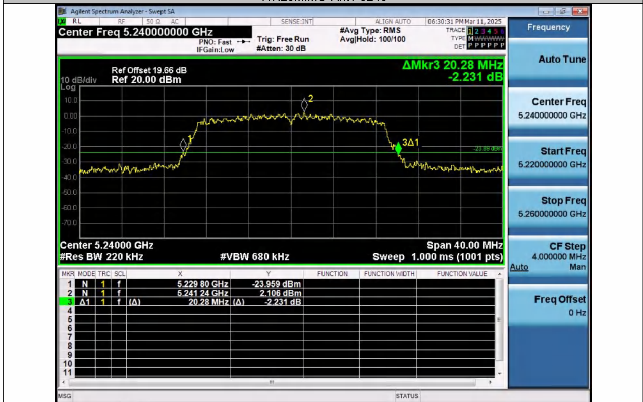
11N20MIMO-Ant2-5240
