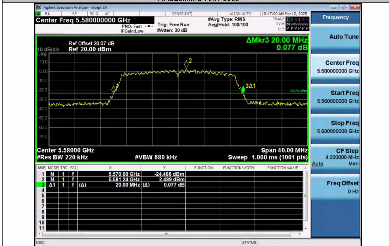
11AC20MIMO-Ant2-5580
