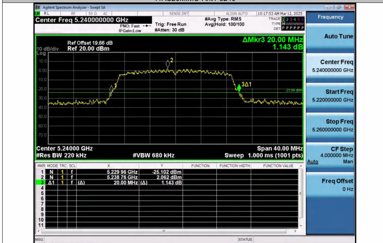
11AC20MIMO-Ant2-5240
