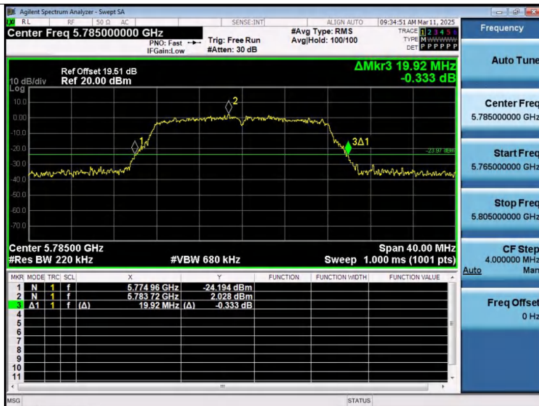
11A-Ant1-5785
