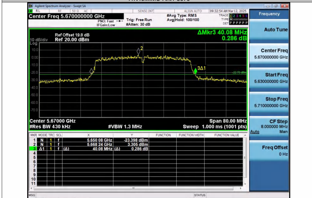
11N40MIMO-Ant2-5670
