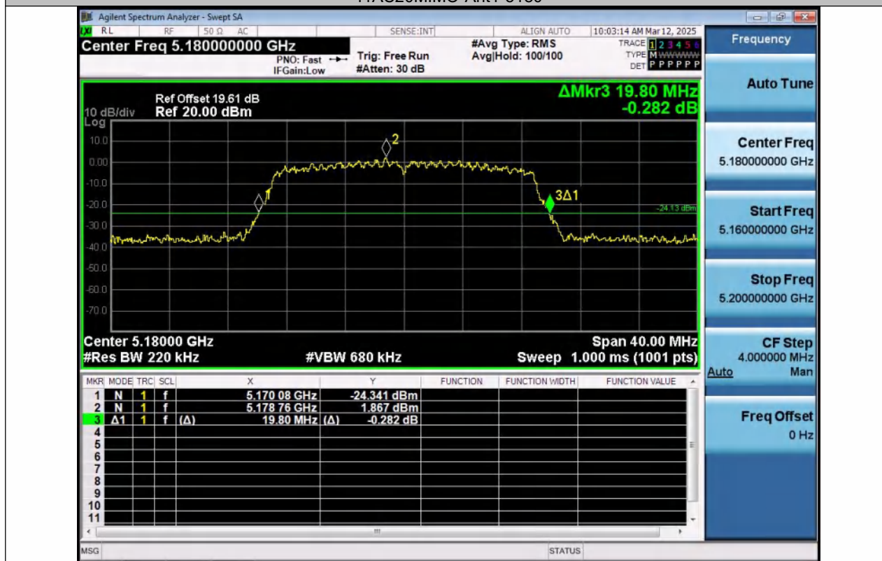
11AC20MIMO-Ant2-5180
