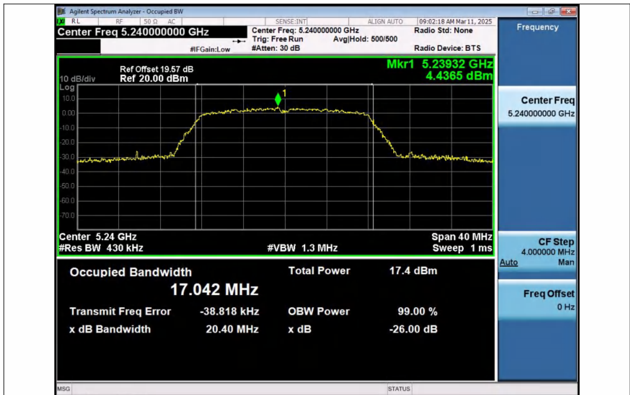
11A-Ant1-5240
