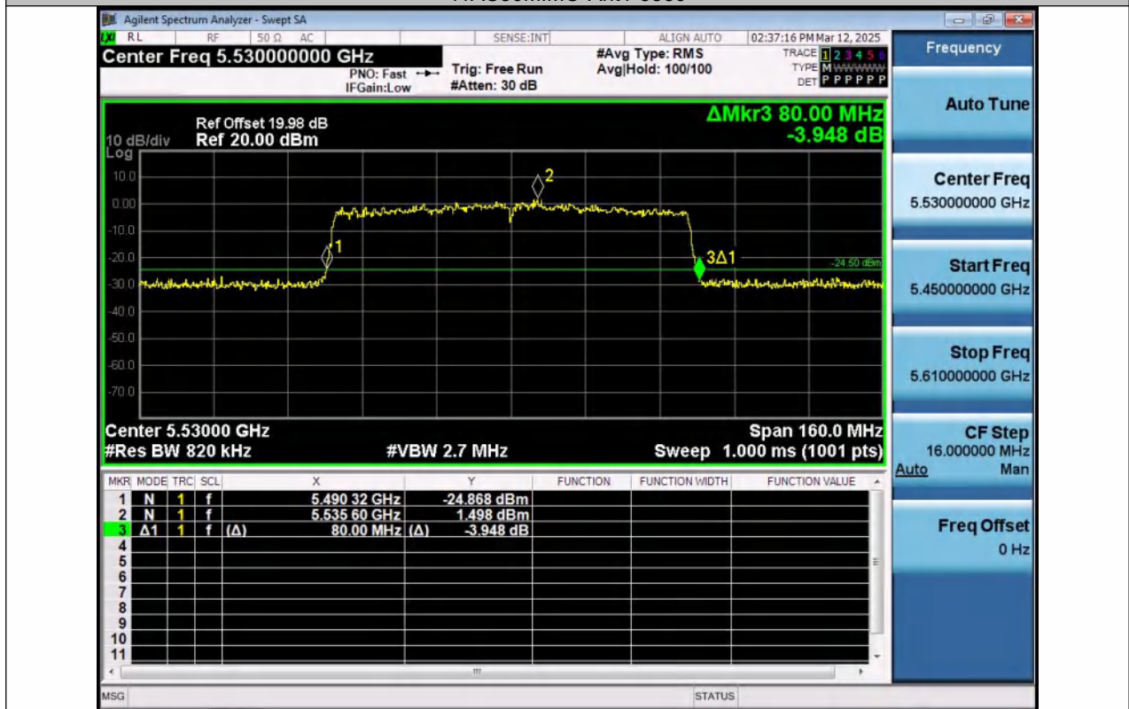
11AC80MIMO-Ant2-5530
