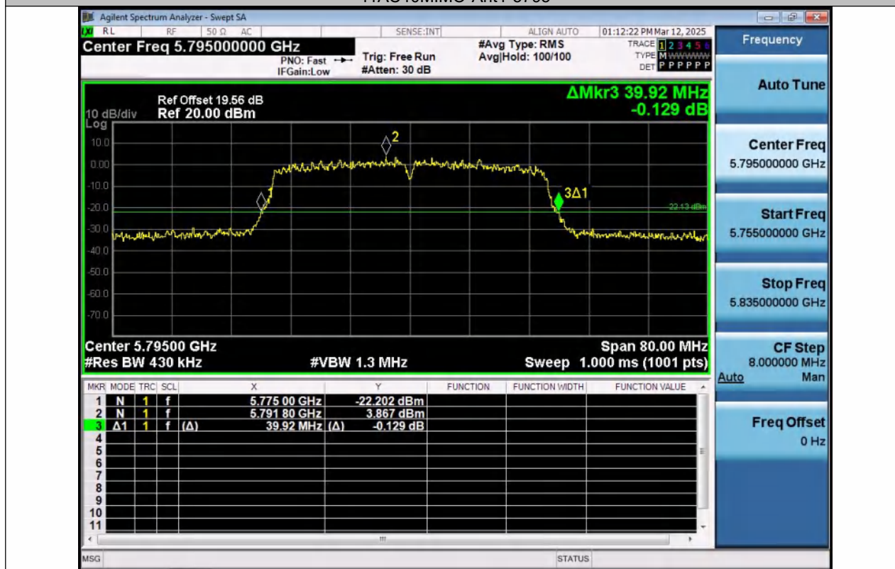
11AC40MIMO-Ant2-5795
