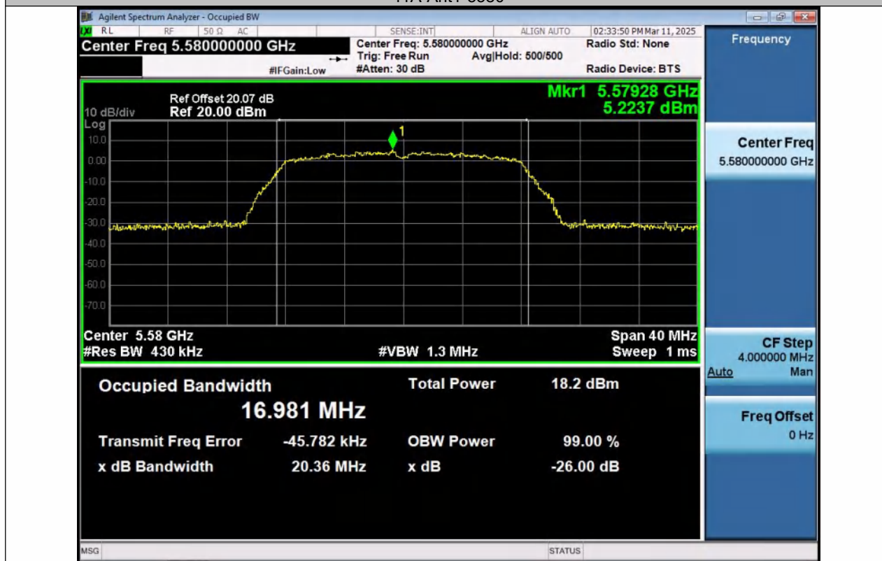
11A-Ant2-5580
