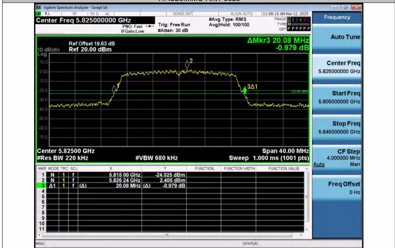
11AC20MIMO-Ant2-5825
