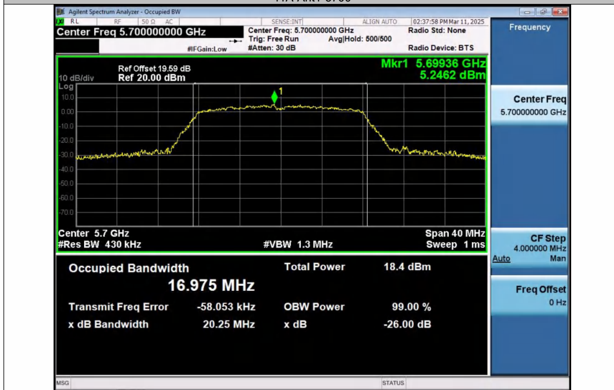
11A-Ant2-5700
