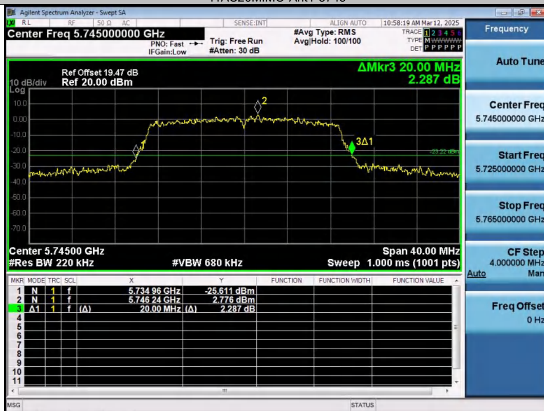
11AC20MIMO-Ant2-5745
