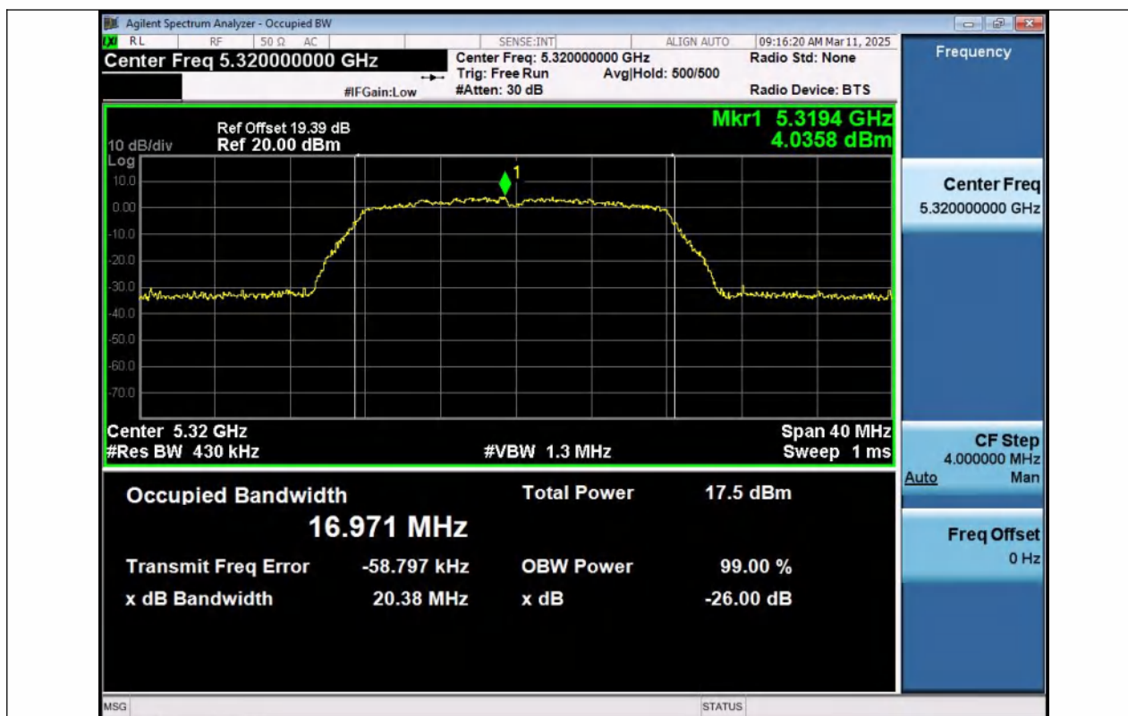
11A-Ant1-5320
