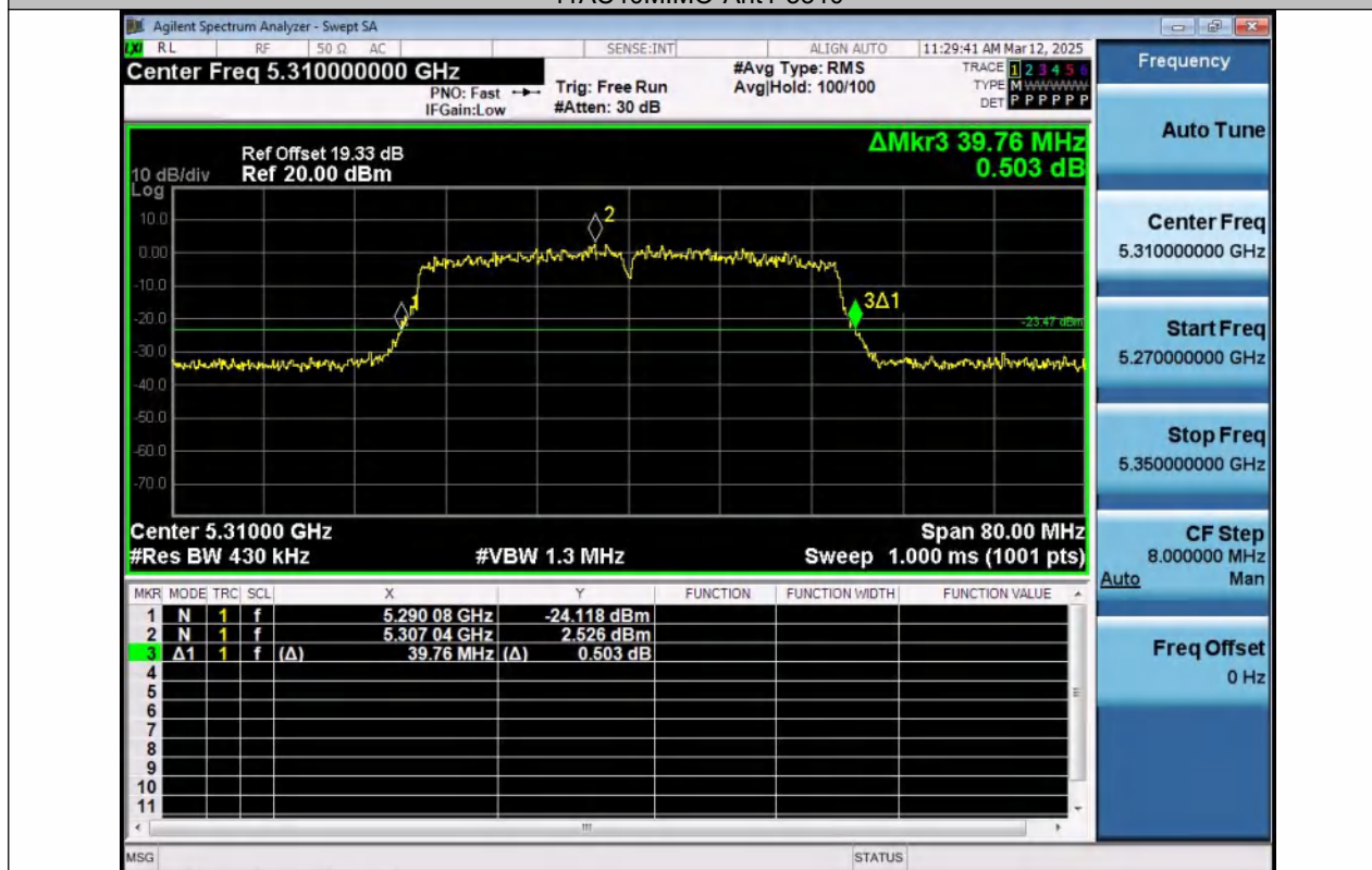
11AC40MIMO-Ant2-5310
