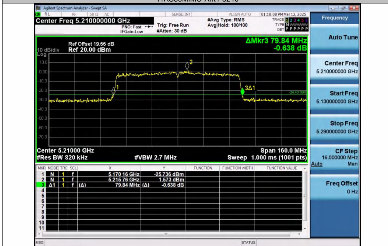
11AC80MIMO-Ant2-5210
