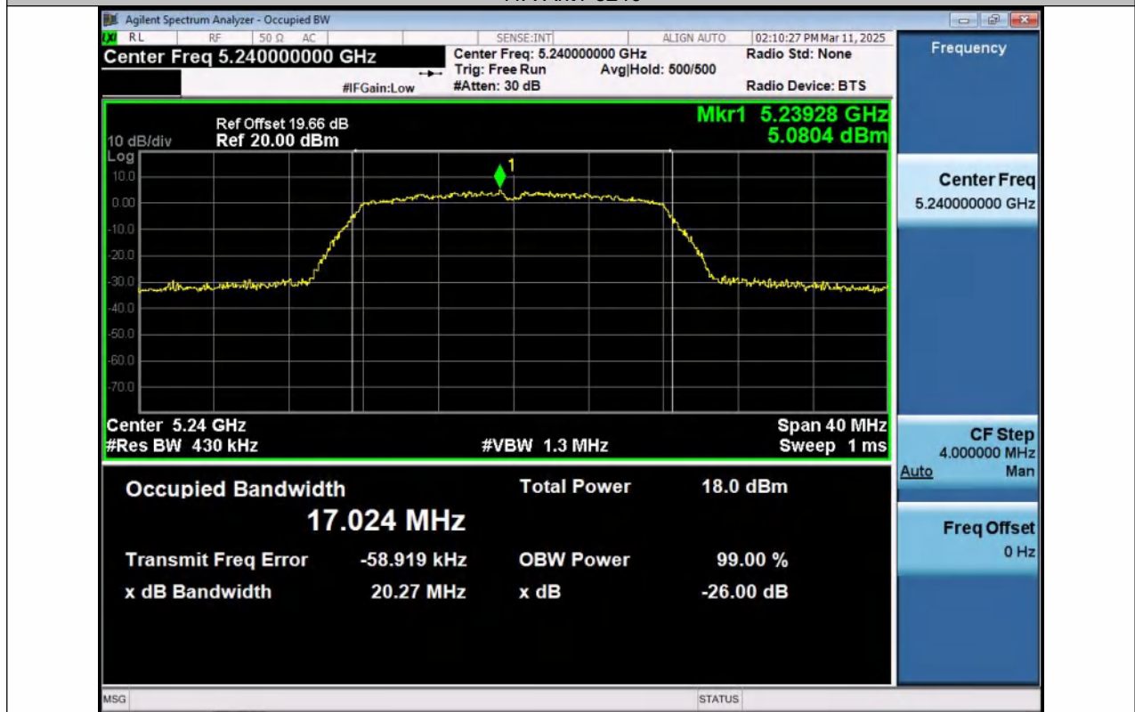
11A-Ant2-5240
