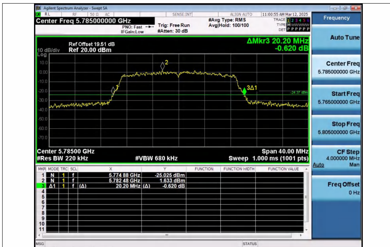
11AC20MIMO-Ant1-5785
