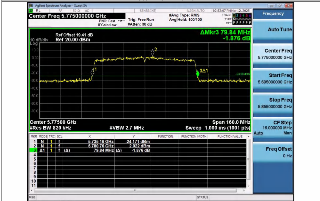
11AC80MIMO-Ant2-5775
