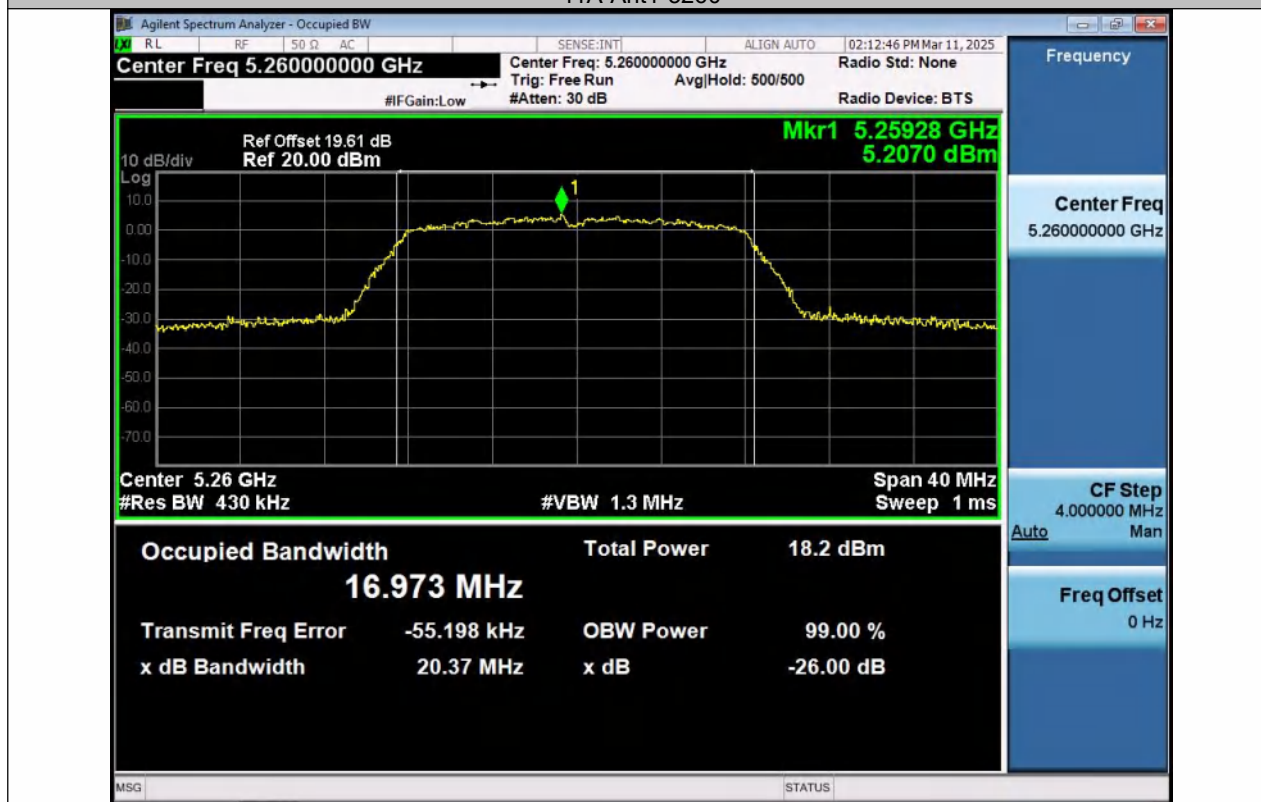
11A-Ant2-5260
