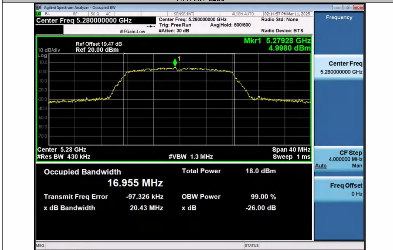
11A-Ant2-5280
