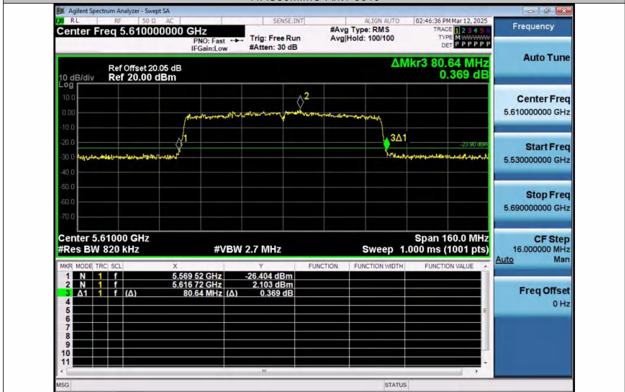
11AC80MIMO-Ant2-5610
