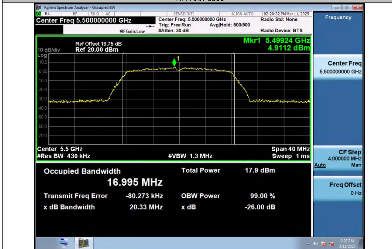
11A-Ant2-5500
