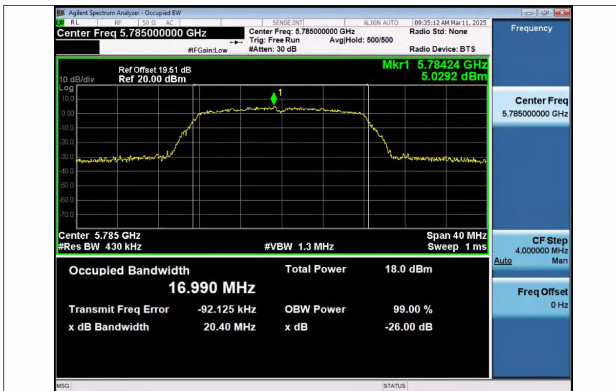
11A-Ant1-5785
