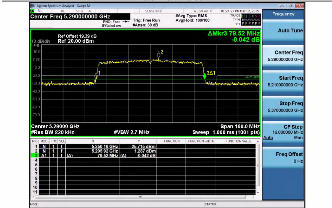
11AC80MIMO-Ant2-5290
