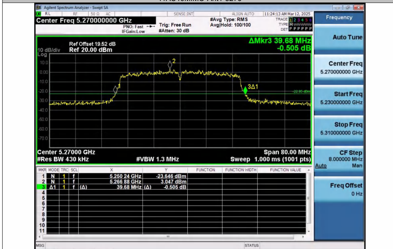
11AC40MIMO-Ant2-5270
