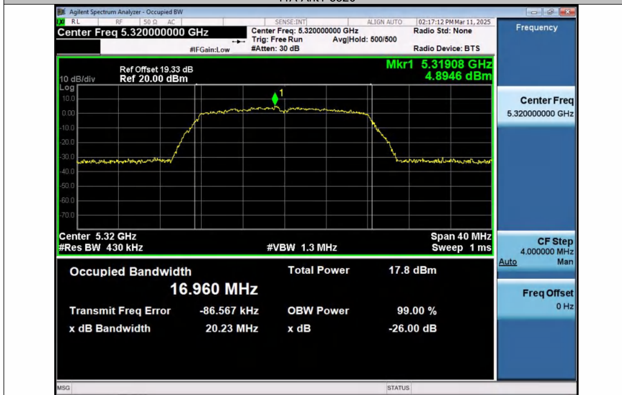
11A-Ant2-5320
