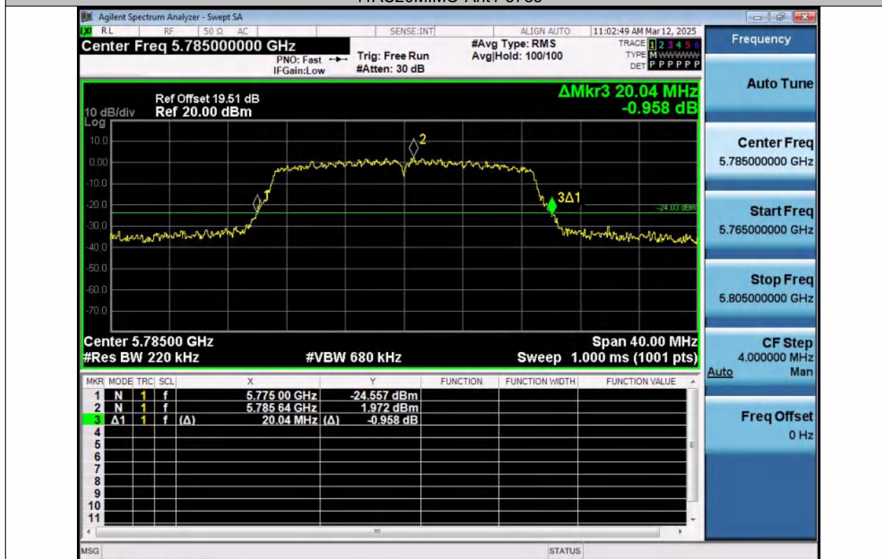
11AC20MIMO-Ant2-5785
