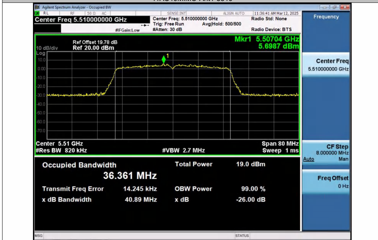
11AC40MIMO-Ant2-5510
