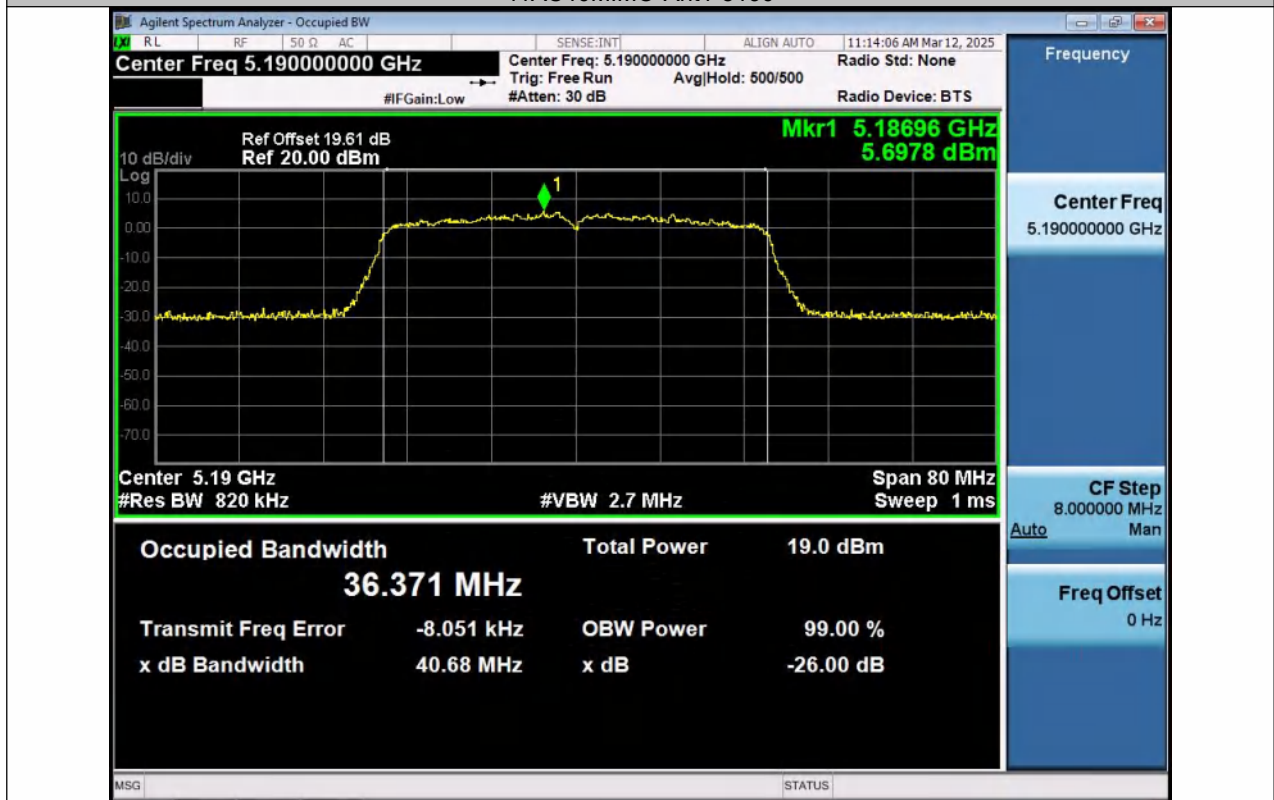
11AC40MIMO-Ant2-5190
