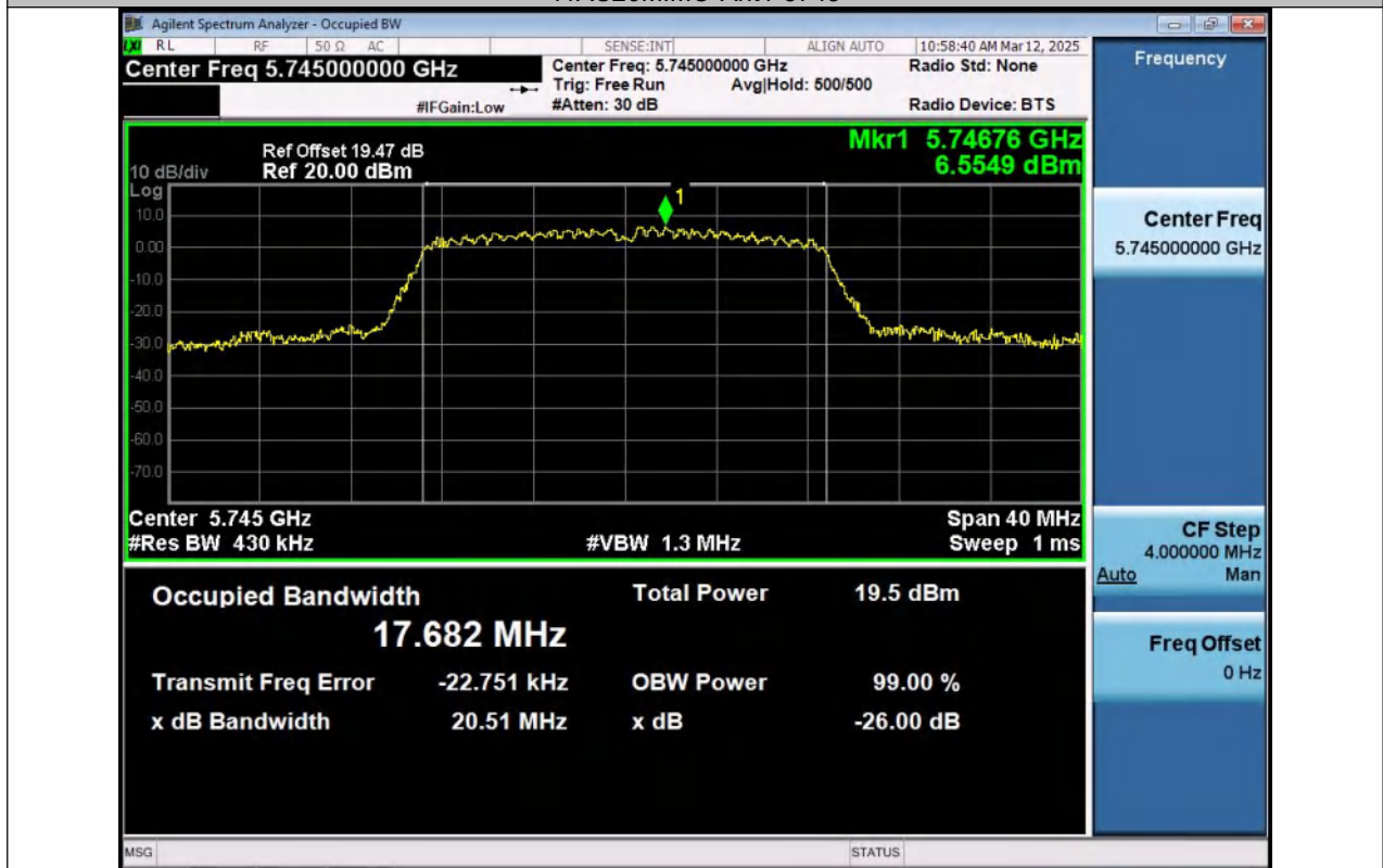
11AC20MIMO-Ant2-5745
