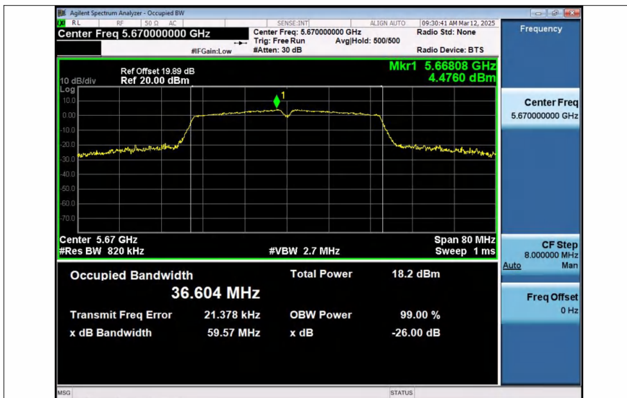
11N40MIMO-Ant1-5670
