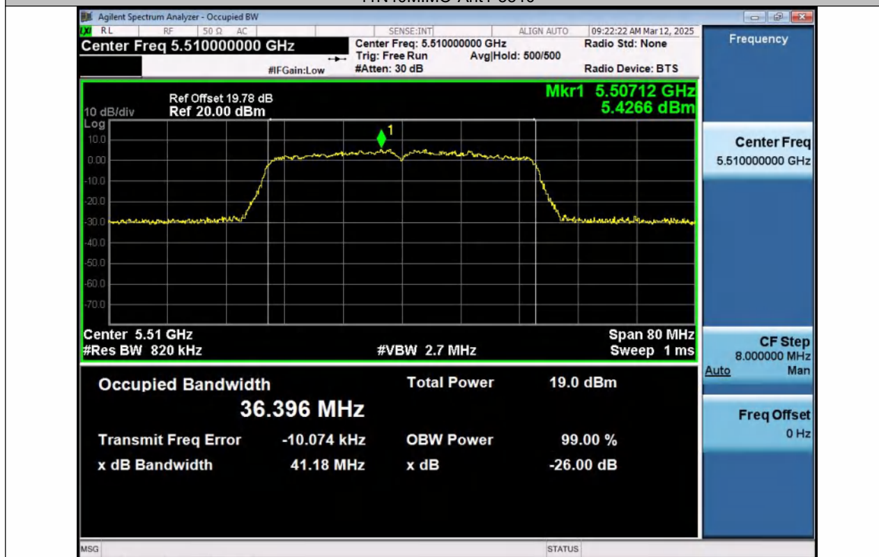
11N40MIMO-Ant2-5510
