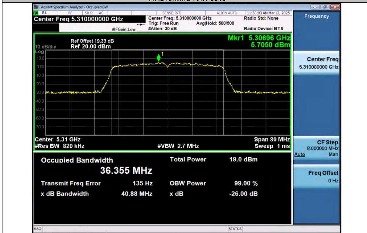
11AC40MIMO-Ant2-5310
