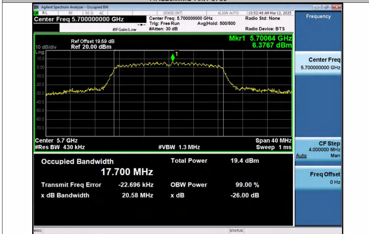
11AC20MIMO-Ant2-5700
