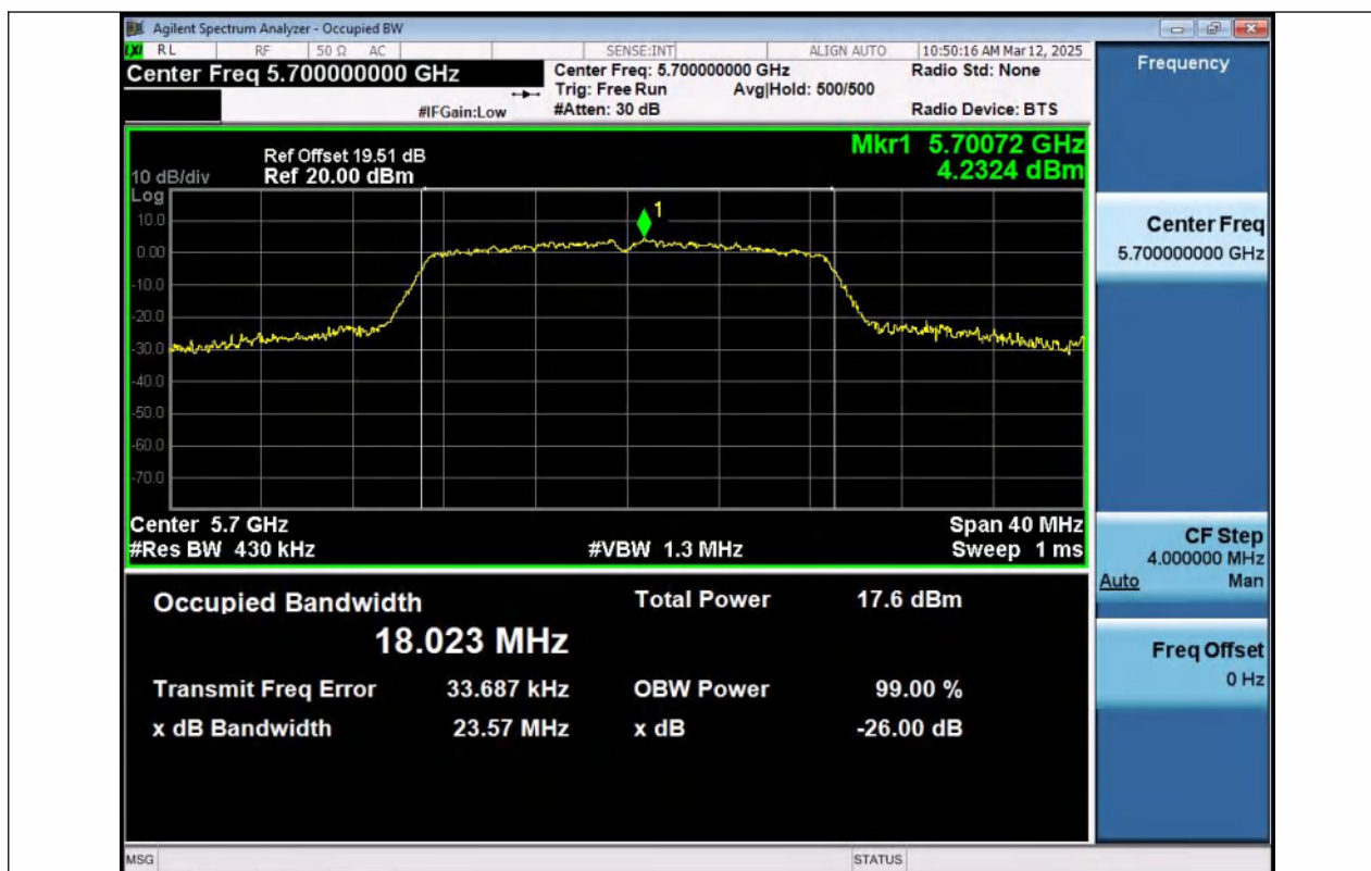
11AC20MIMO-Ant1-5700
