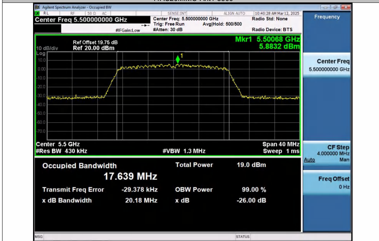
11AC20MIMO-Ant2-5500
