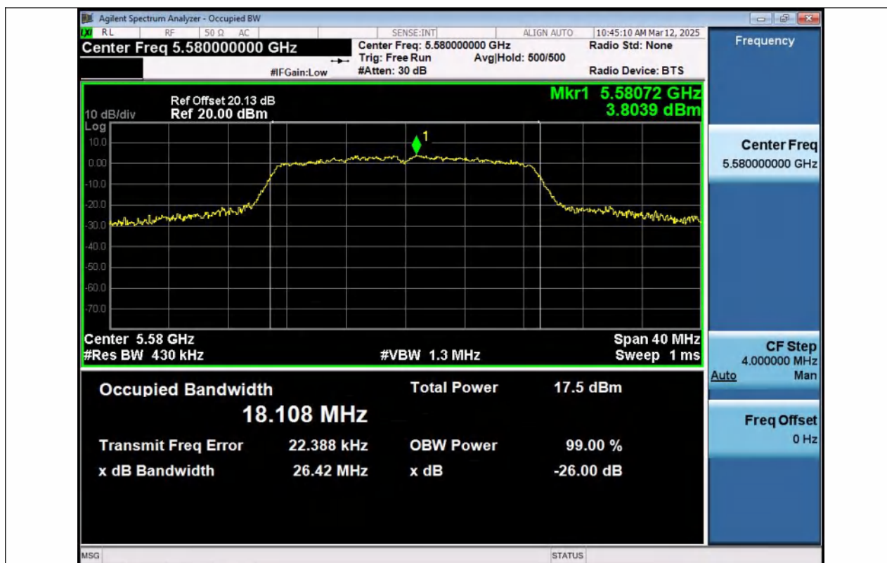
11AC20MIMO-Ant1-5580
