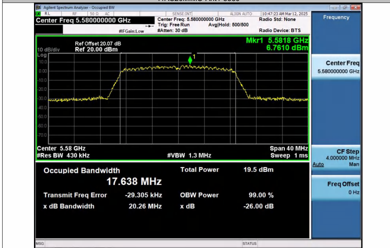
11AC20MIMO-Ant2-5580
