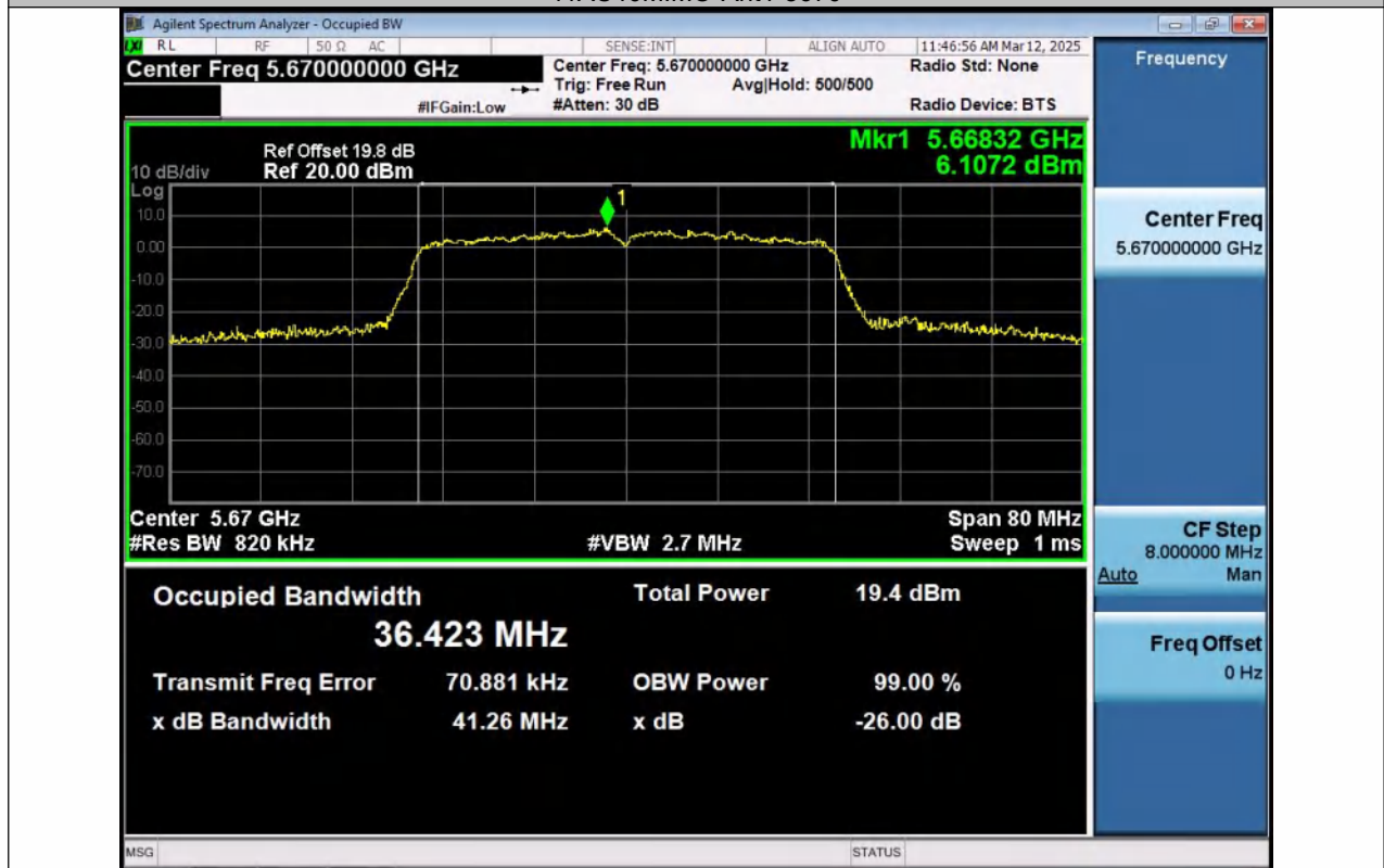
11AC40MIMO-Ant2-5670
