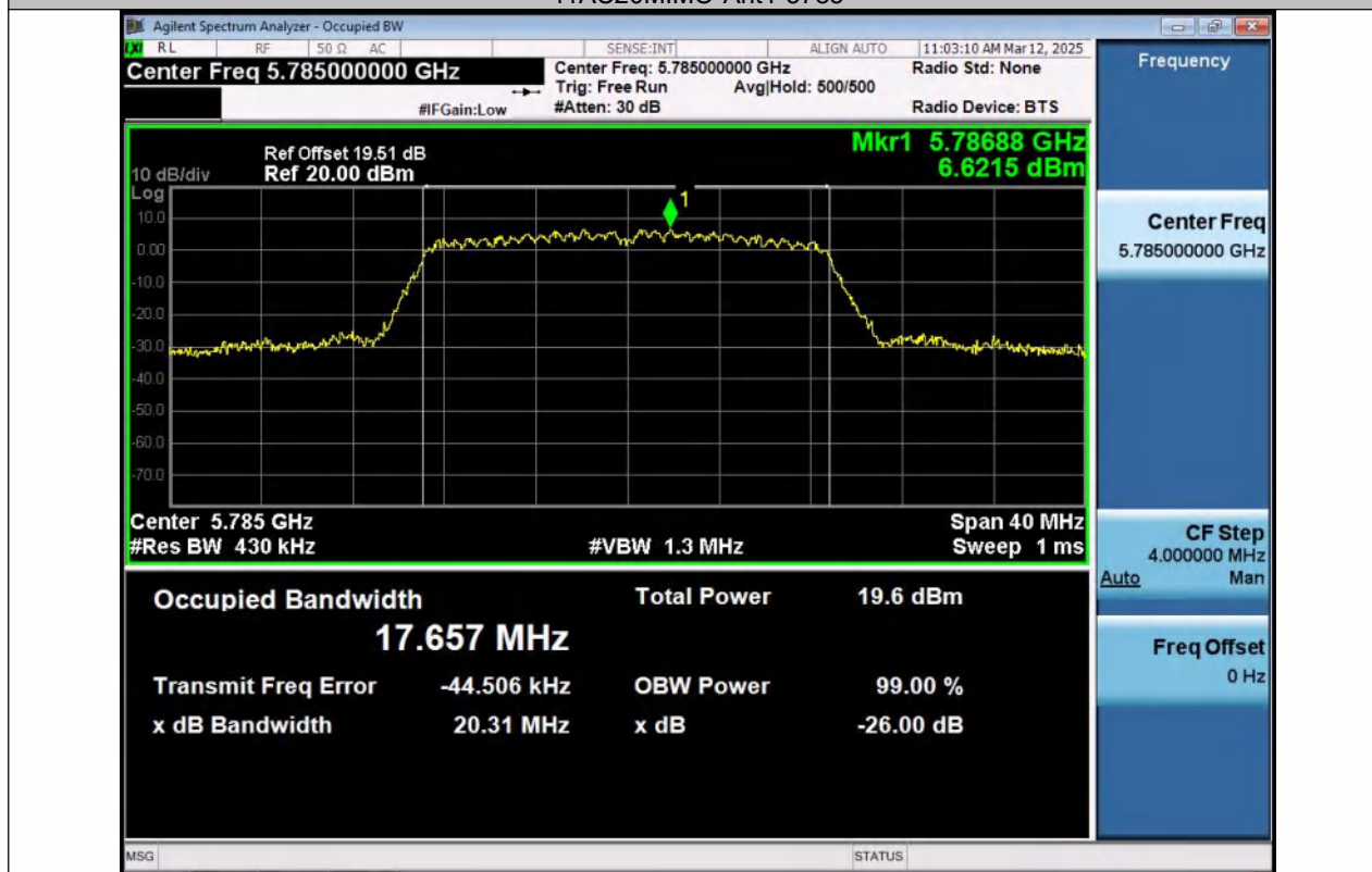
11AC20MIMO-Ant2-5785
