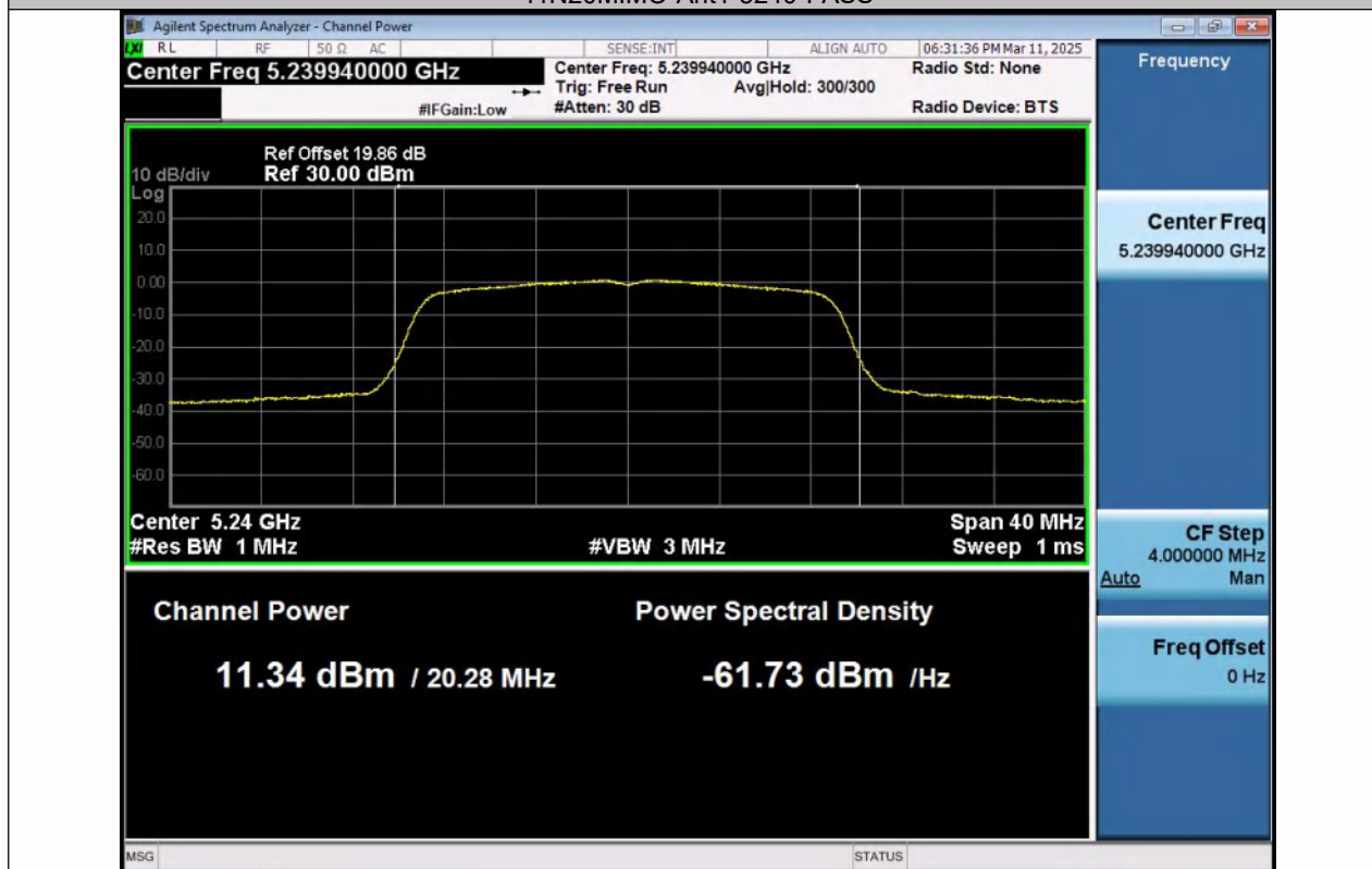
11N20MIMO-Ant2-5240-PASS
