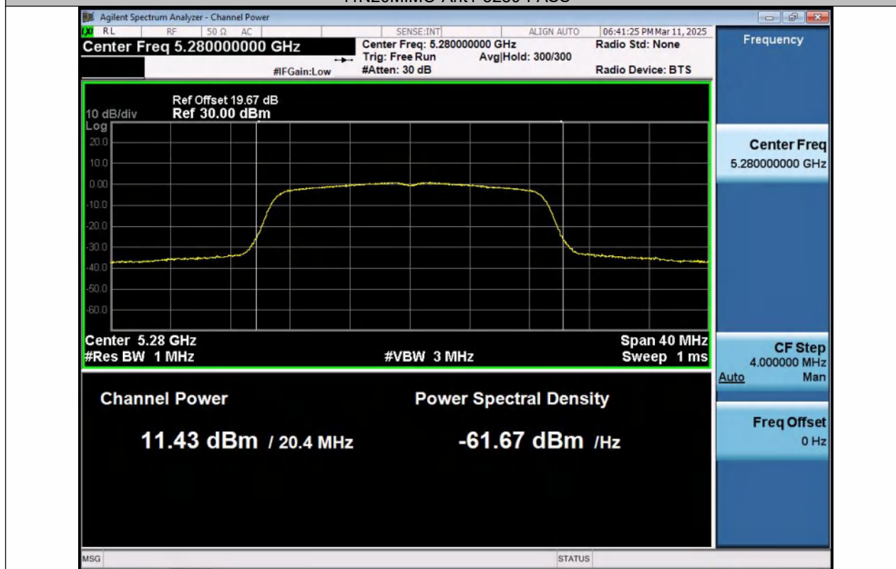
11N20MIMO-Ant2-5280-PASS
