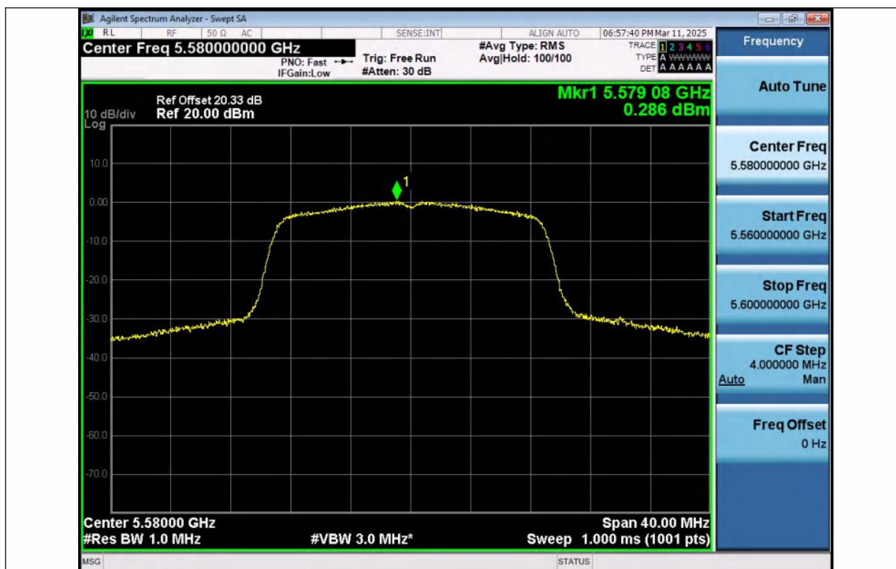
11N20MIMO-Ant1-5580-PASS
