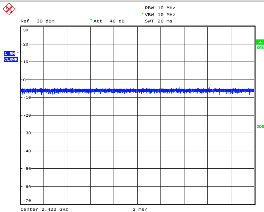
Test Graph_IEEE802.11 n (HT40) Duty Cycle:
