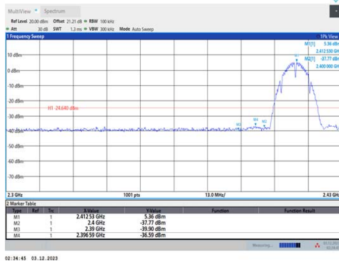
11B_Ant2_Low_2412
