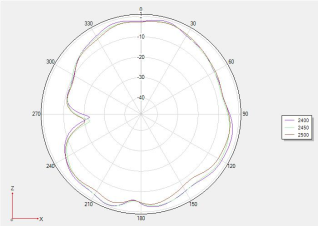
Phi 0 2D graph
