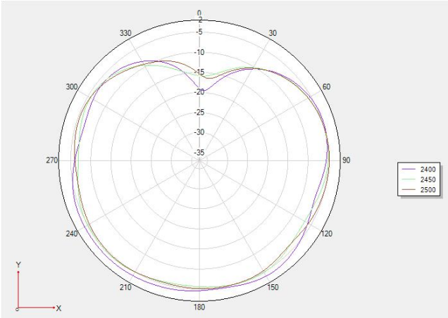
The Theta 90 2D chart
