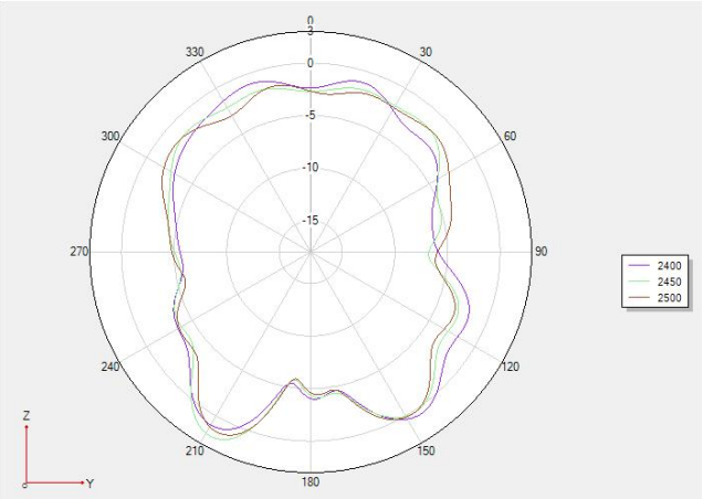
Phi 90 2D chart
