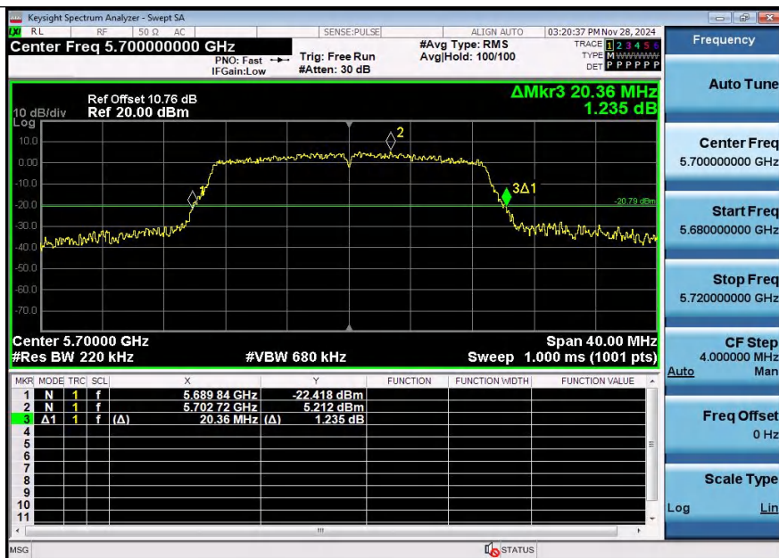
11N20SISO-Ant2-5700
