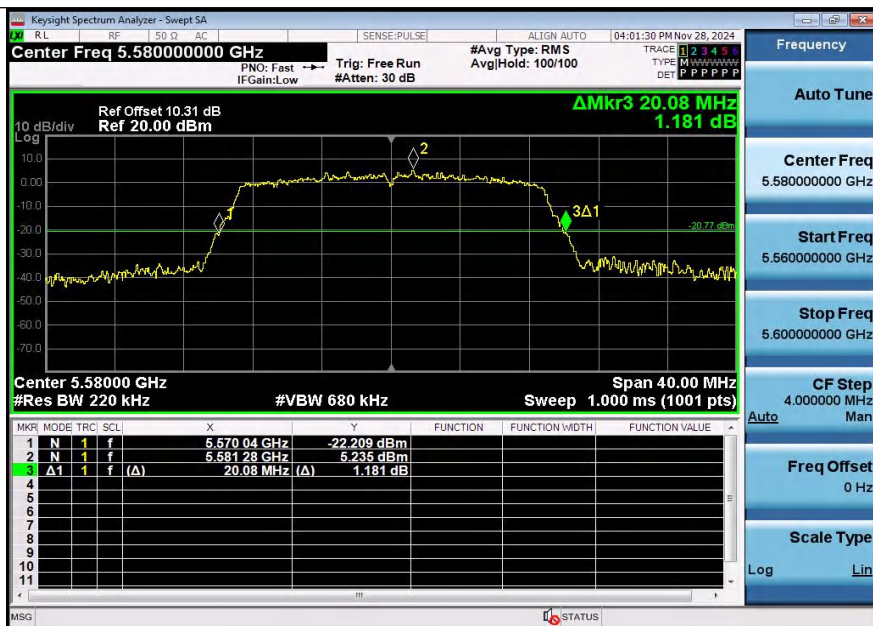
11AC20SISO-Ant2-5580
