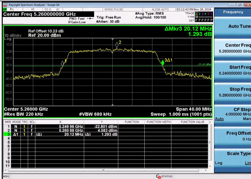
11N20SISO-Ant2-5260
