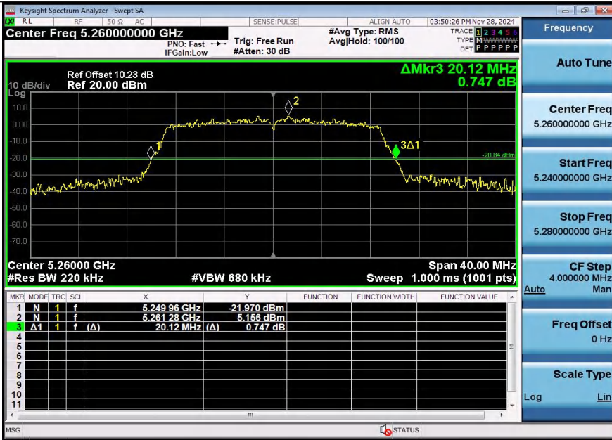
11AC20SISO-Ant2-5260
