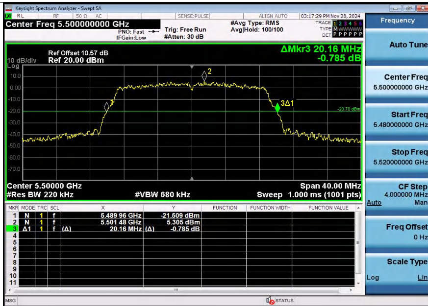
11N20SISO-Ant2-5500
