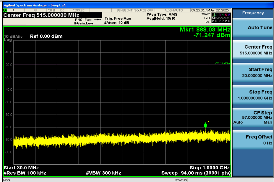
3DH5-Ant1-2480-30~1000-PASS
