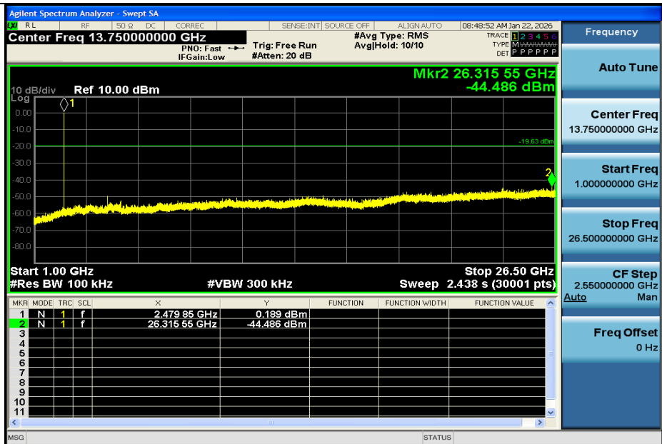
DH5-Ant1-2480-1000~26500-PASS
