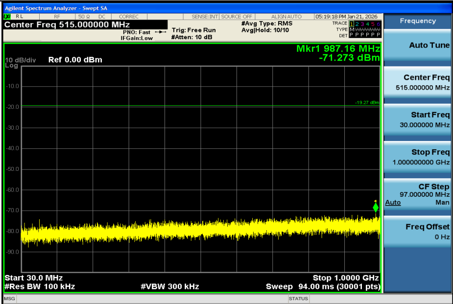
DH5-Ant1-2402-30~1000-PASS
