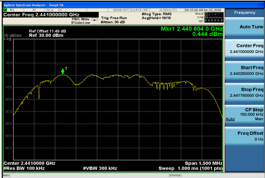
3DH5-Ant1-2441-0~Reference-PASS
