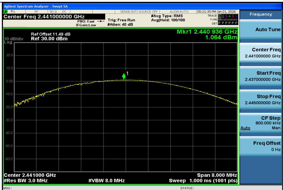
DH5-Ant1-2441-PASS
