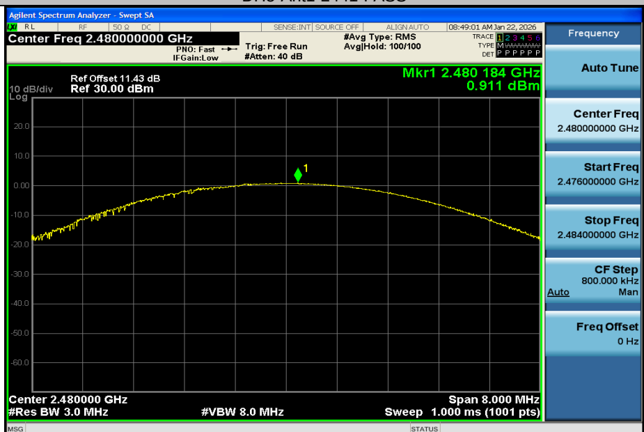
DH5-Ant1-2480-PASS
