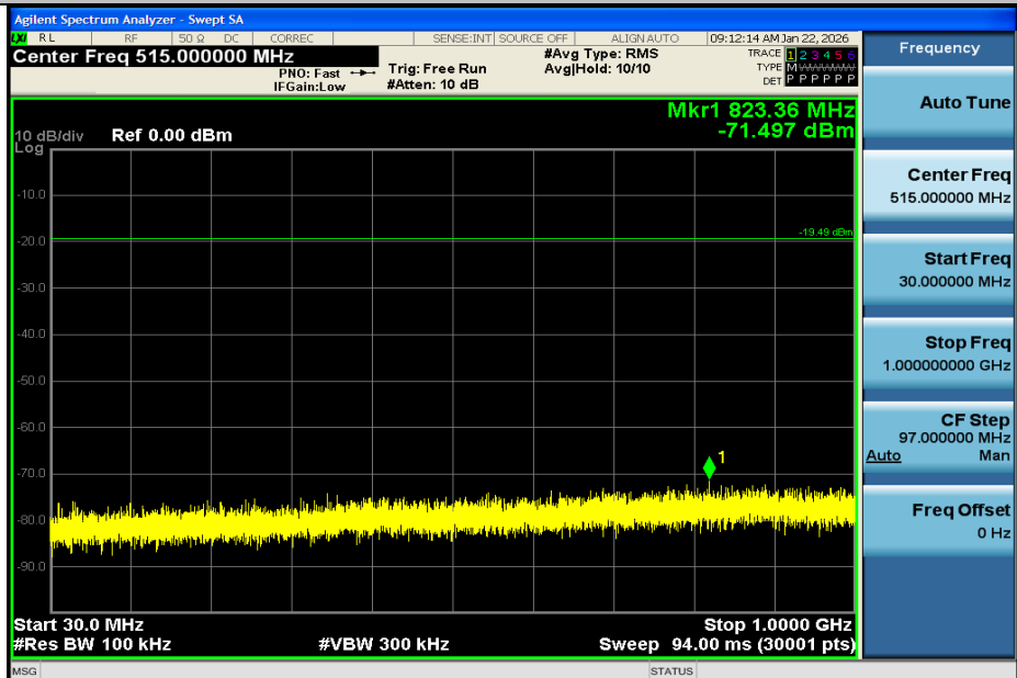
3DH5-Ant1-2402-30~1000-PASS
