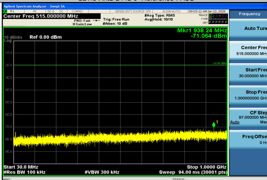
2DH5-Ant1-2441-30~1000-PASS
