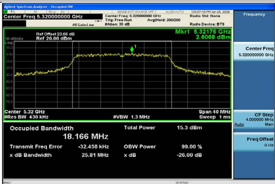
11N20MIMO-Ant2-5320
