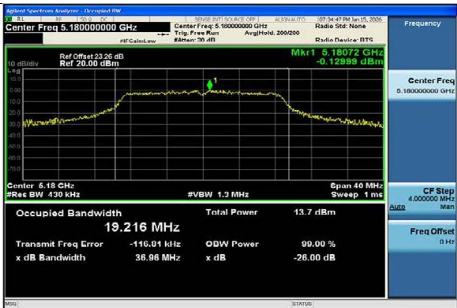
11AC20MIMO-Ant1-5180
