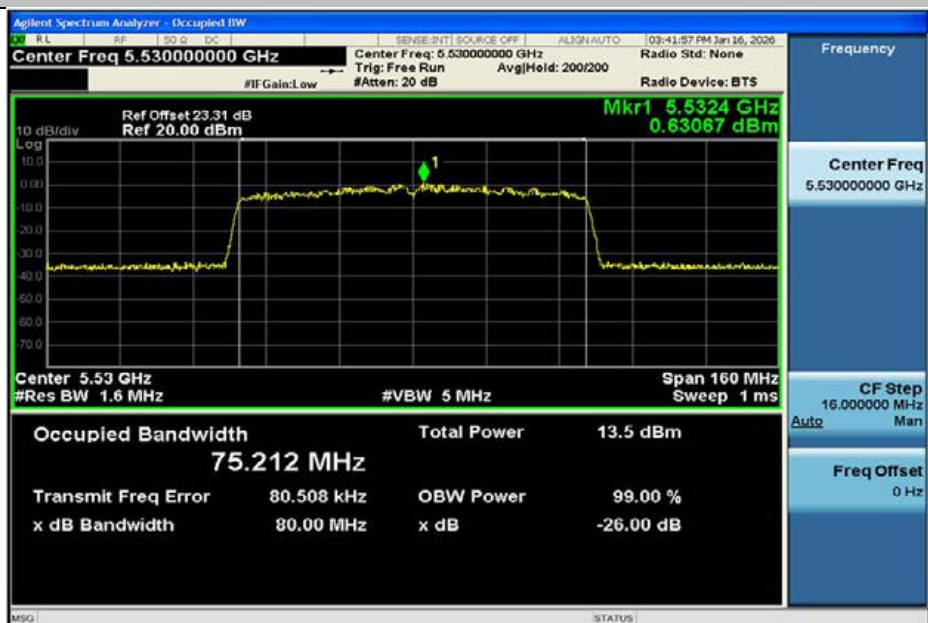
11AC80MIMO-Ant2-5530
