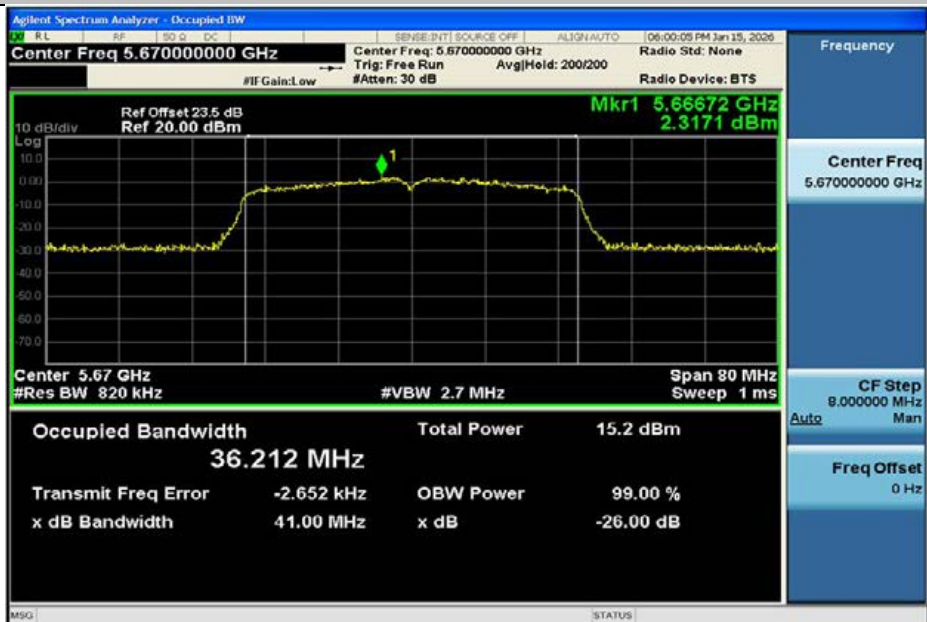
11N40MIMO-Ant2-5670
