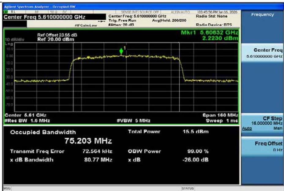
11AC80MIMO-Ant1-5610
