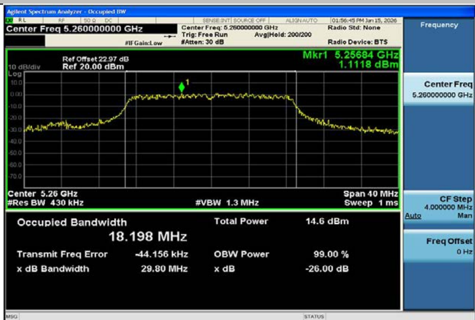
11N20MIMO-Ant2-5260
