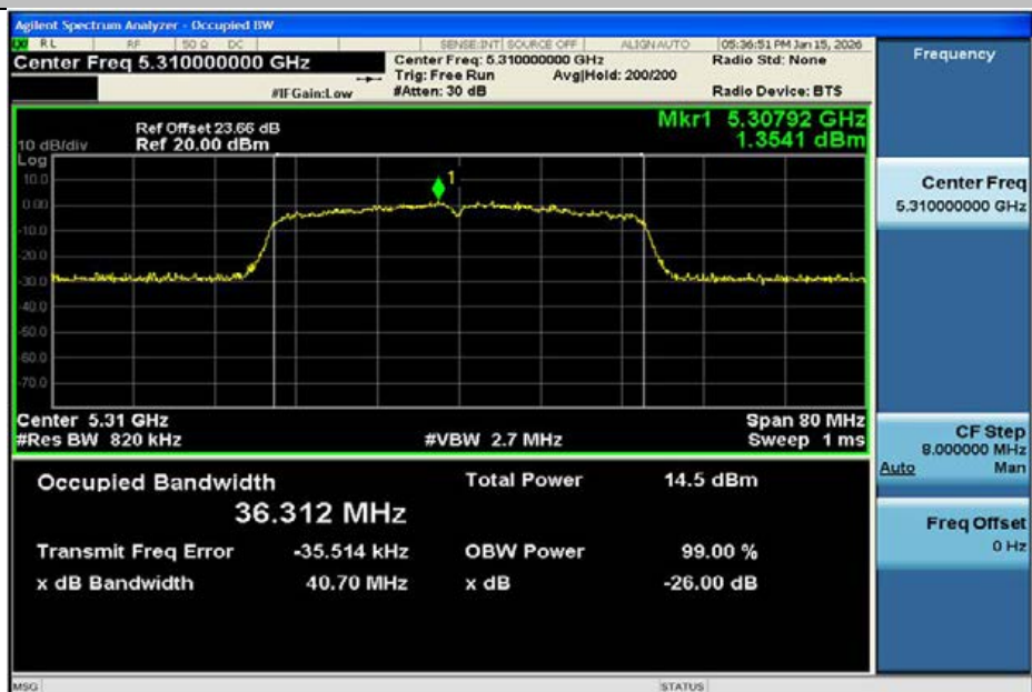
11N40MIMO-Ant2-5310
