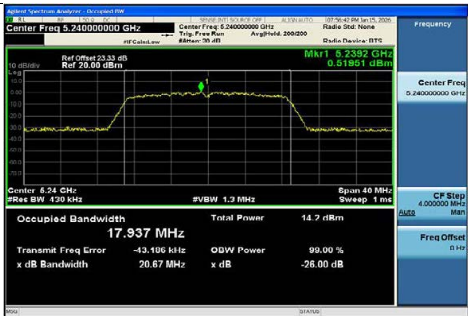
11AC20MIMO-Ant1-5240
