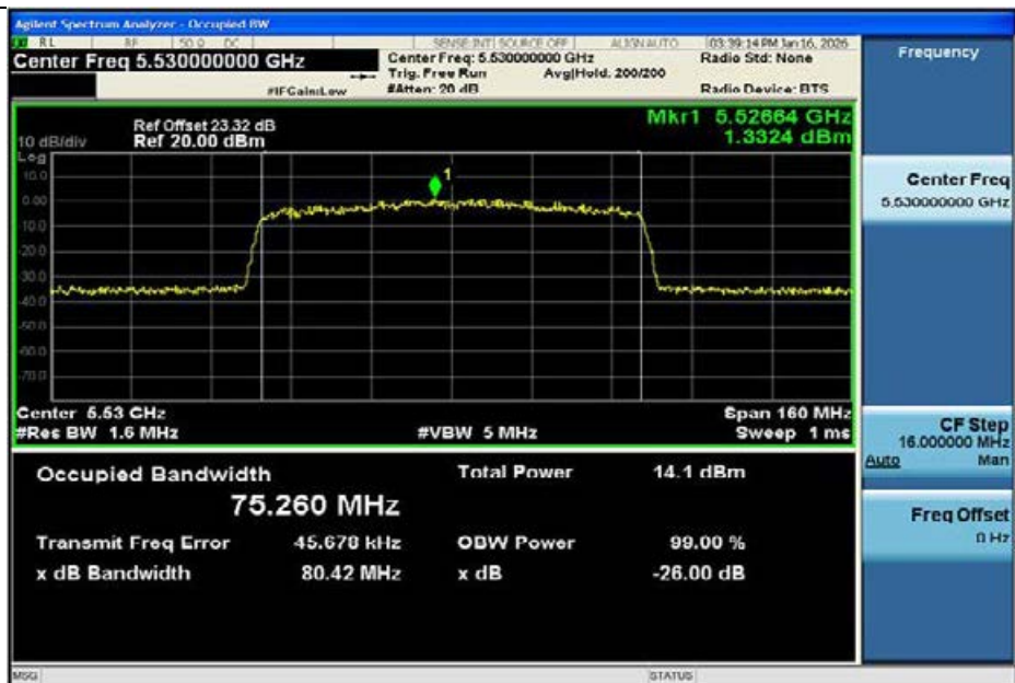
11AC80MIMO-Ant1-5530
