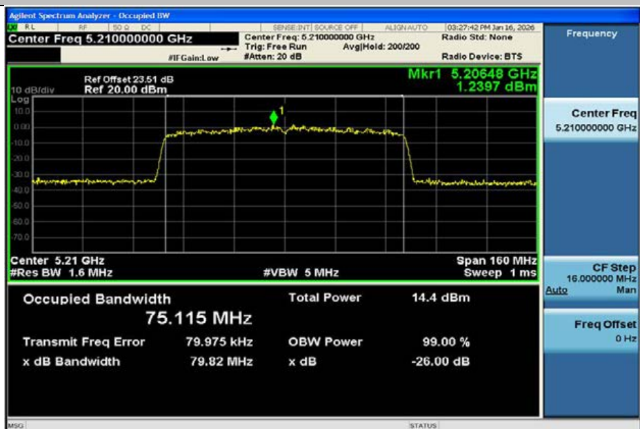
11AC80MIMO-Ant2-5210
