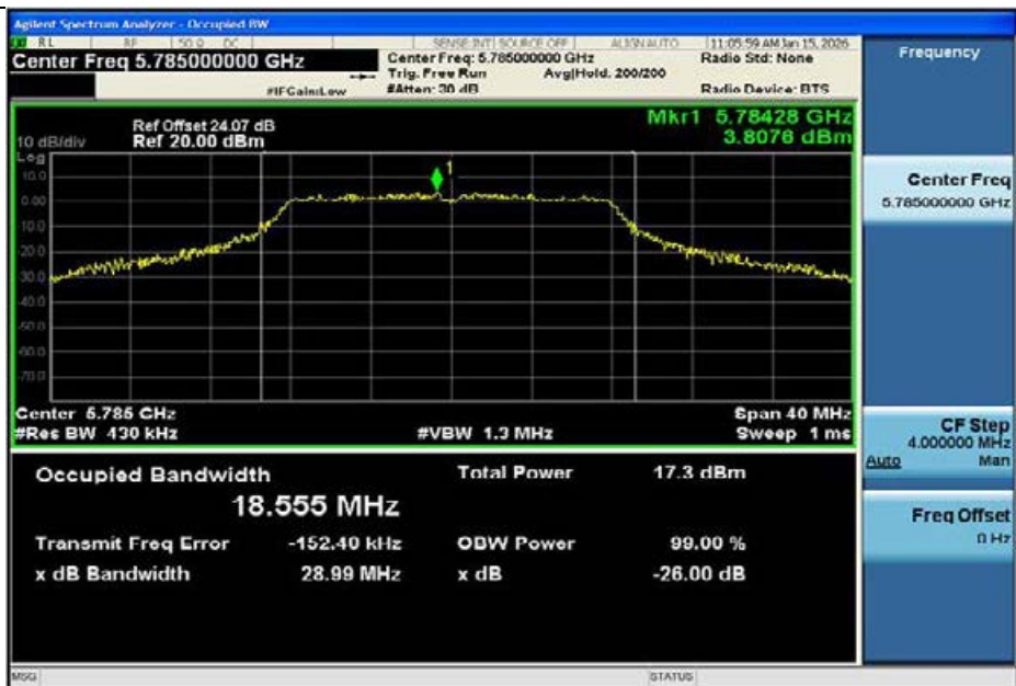
11A-CDD-Ant1-5785
