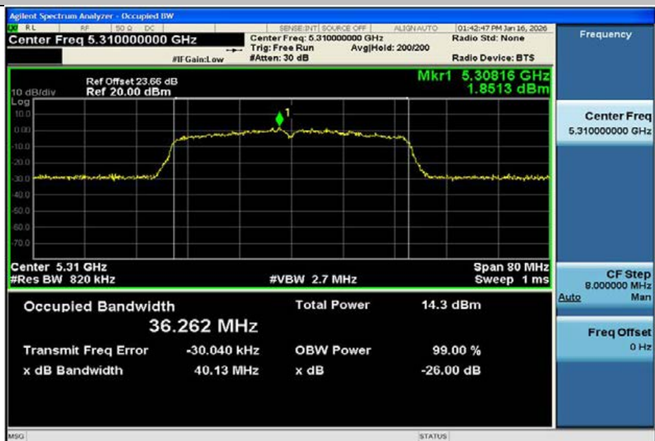
11AC40MIMO-Ant2-5310
