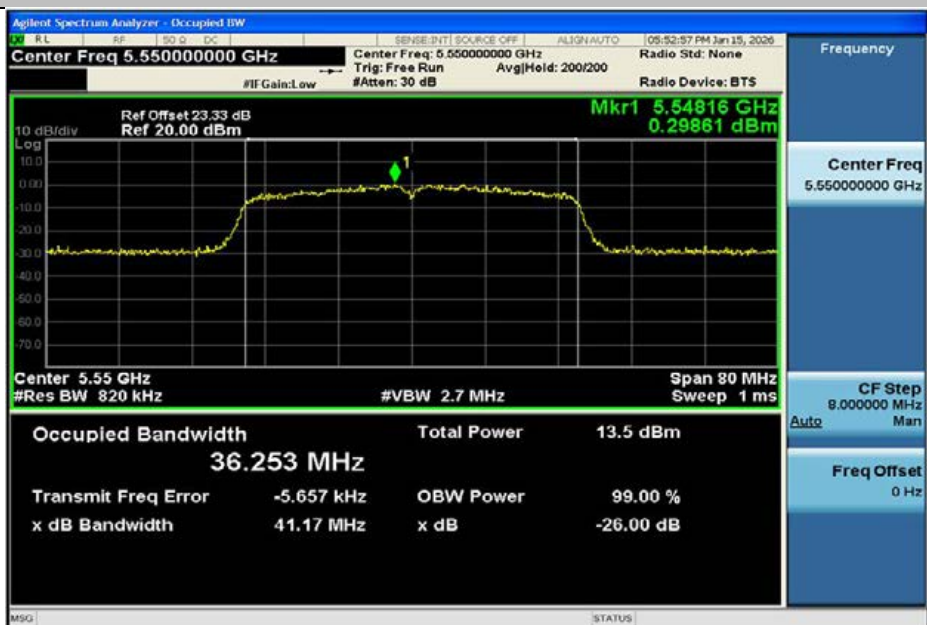
11N40MIMO-Ant2-5550
