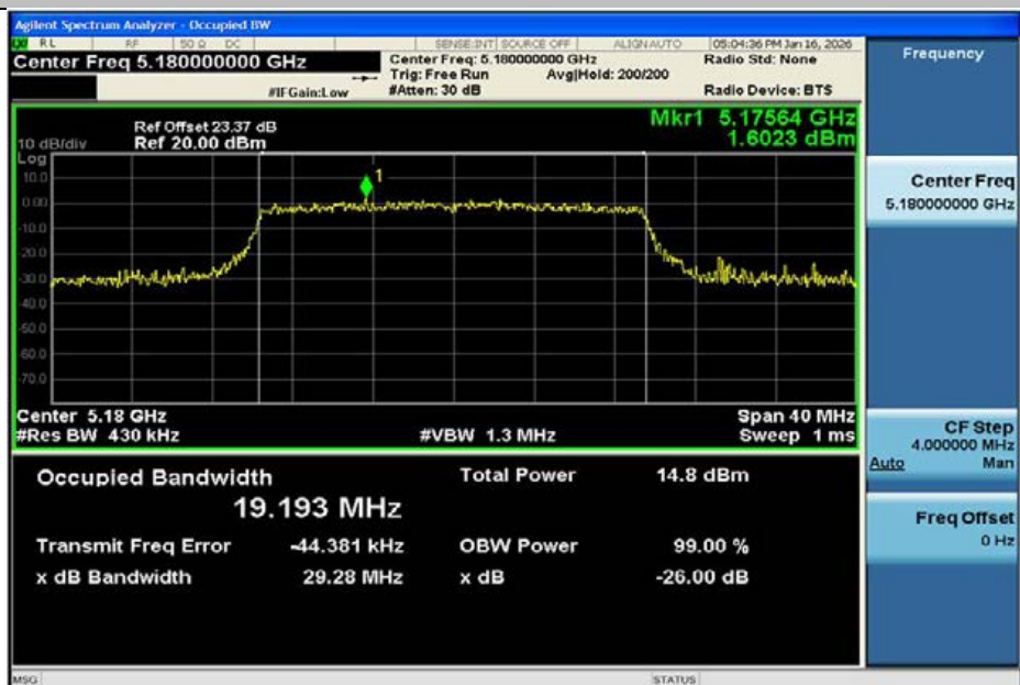
11AX20MIMO-Ant2-5180
