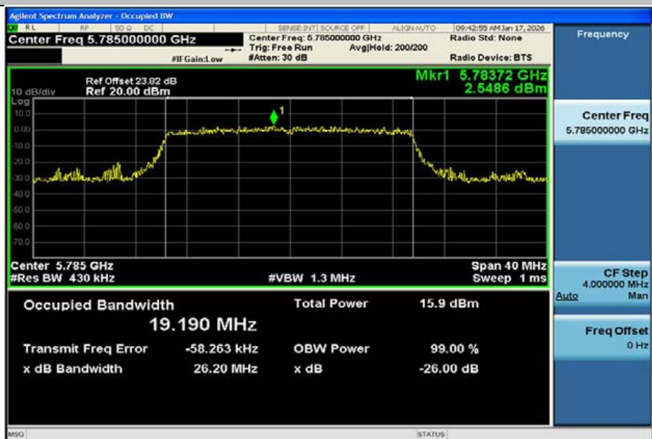
11AX20MIMO-Ant2-5785
