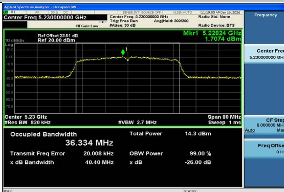
11AC40MIMO-Ant2-5230
