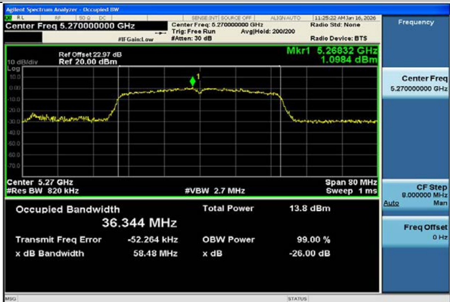
11AC40MIMO-Ant2-5270
