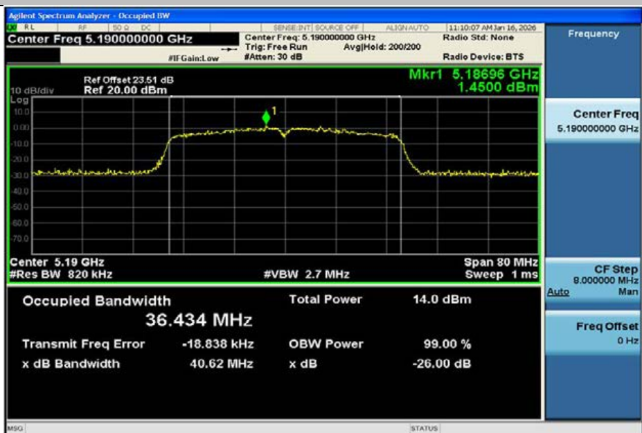
11AC40MIMO-Ant2-5190
