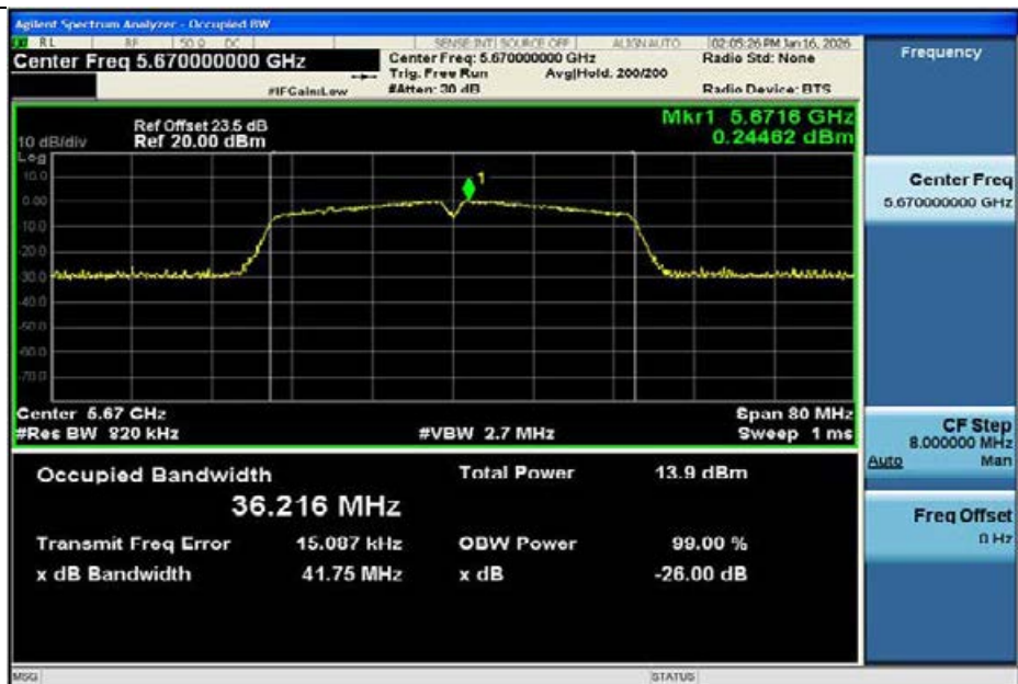
11AC40MIMO-Ant1-5670
