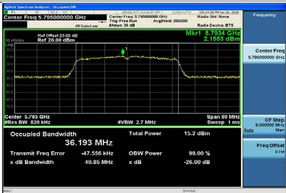
11AC40MIMO-Ant2-5795
