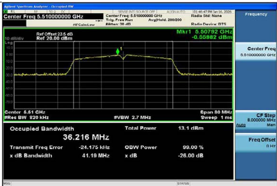
11AC40MIMO-Ant1-5510
