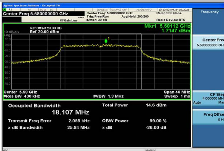
11AC20MIMO-Ant2-5580
