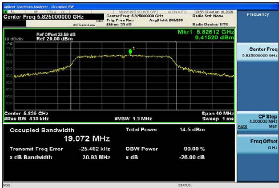
11AC20MIMO-Ant1-5825
