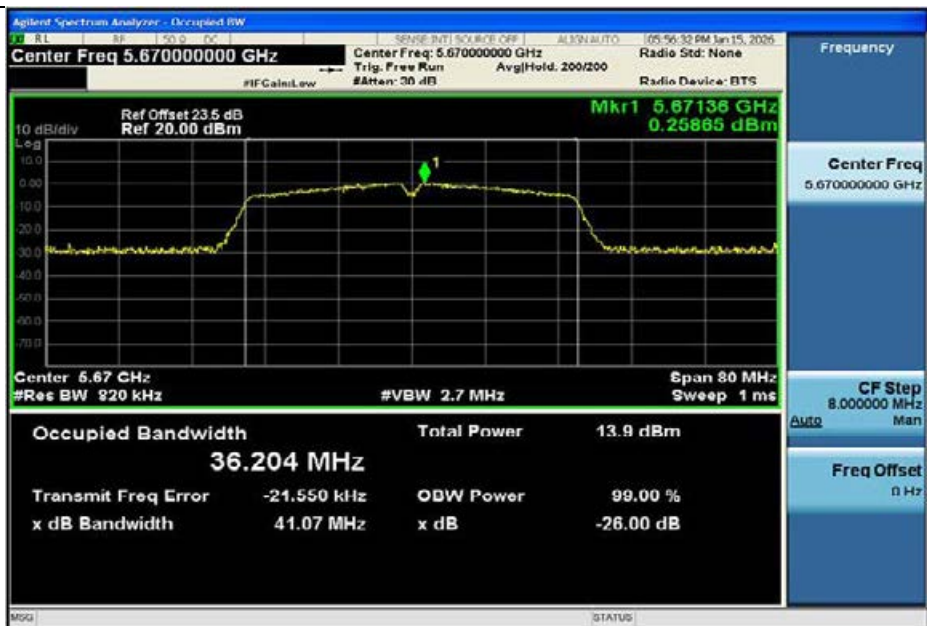
11N40MIMO-Ant1-5670
