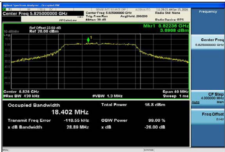
11A-CDD-Ant1-5825
