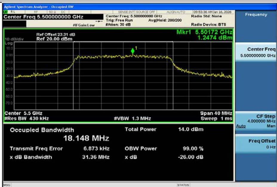
11AC20MIMO-Ant2-5500
