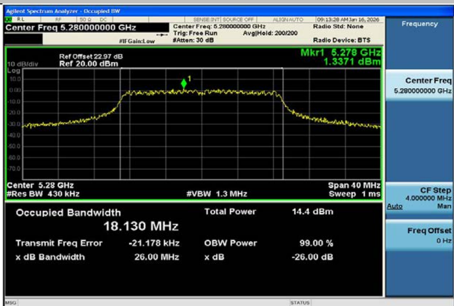
11AC20MIMO-Ant2-5280
