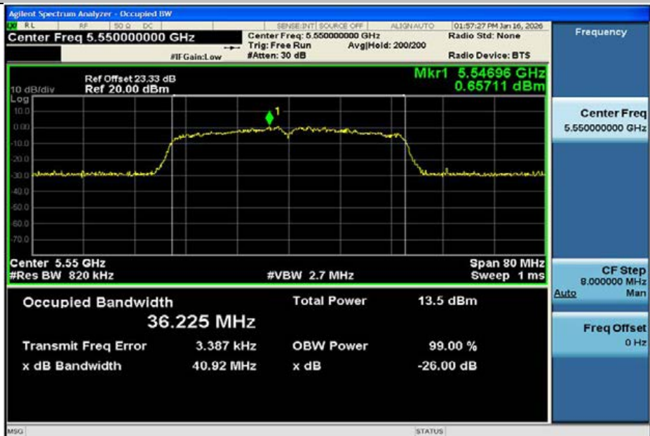
11AC40MIMO-Ant2-5550
