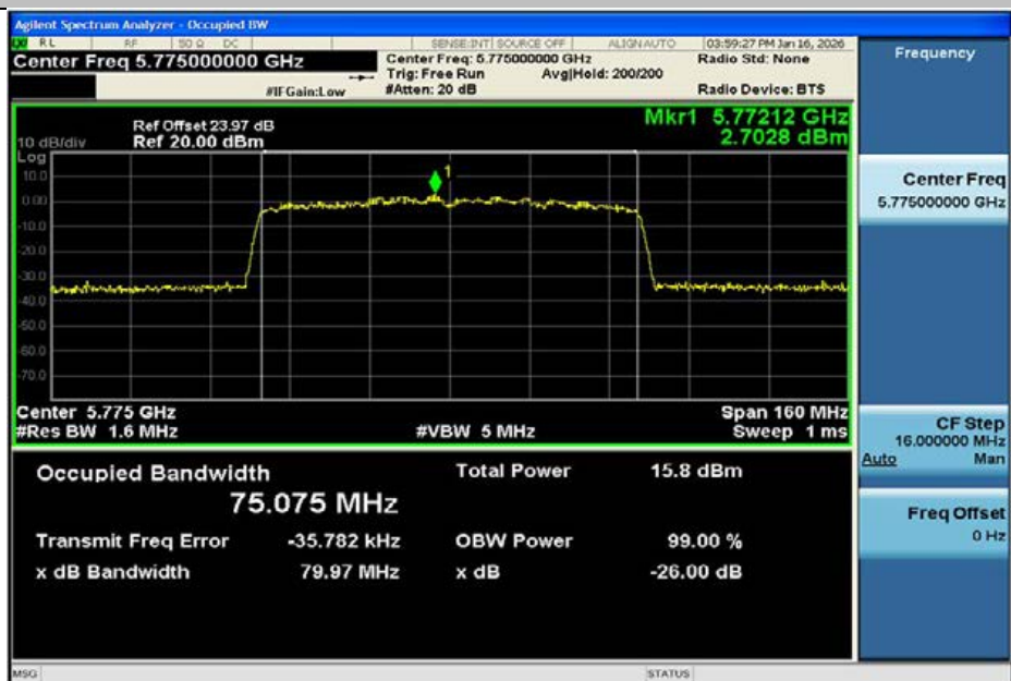
11AC80MIMO-Ant2-5775
