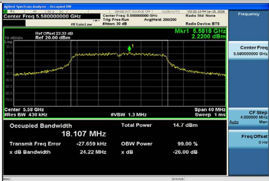
11N20MIMO-Ant2-5580
