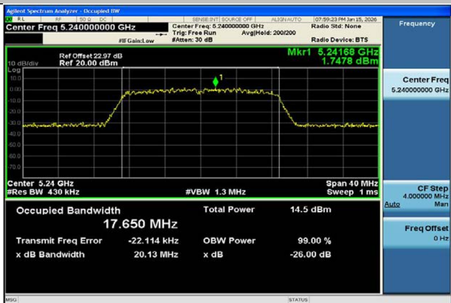
11AC20MIMO-Ant2-5240
