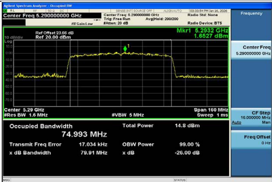
11AC80MIMO-Ant2-5290
