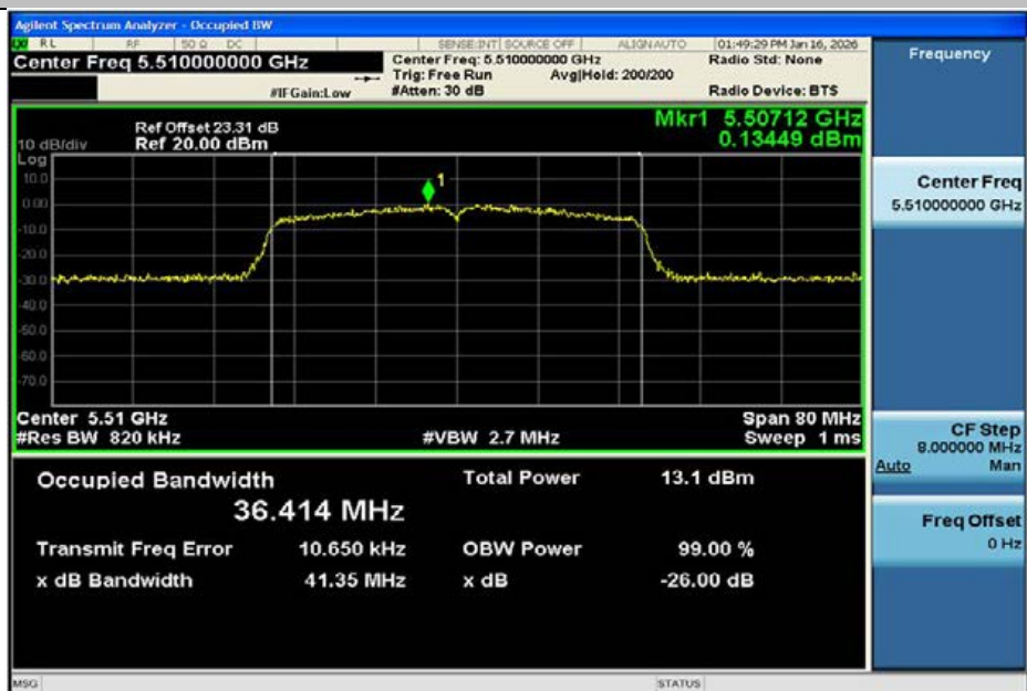
11AC40MIMO-Ant2-5510
