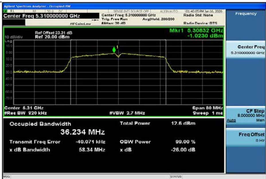
11AC40MIMO-Ant1-5310
