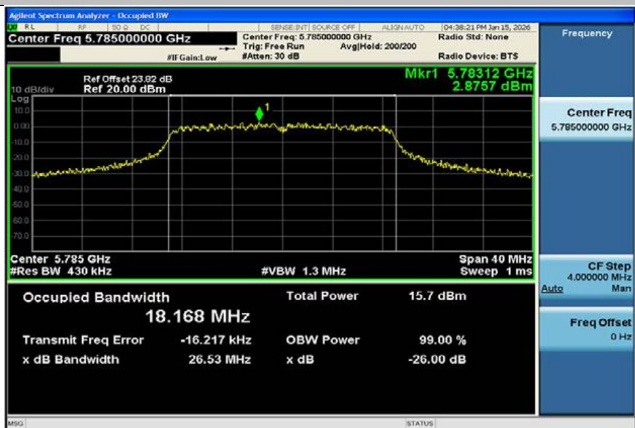
11N20MIMO-Ant2-5785
