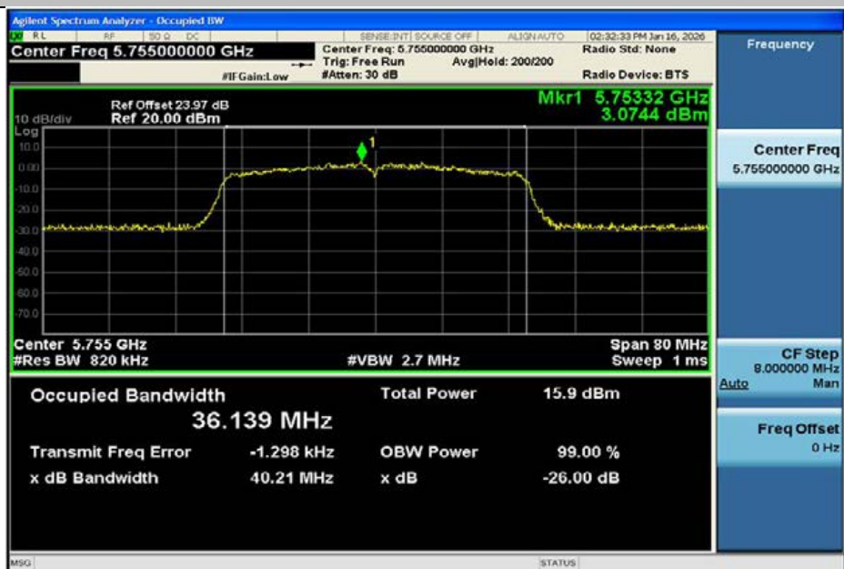
11AC40MIMO-Ant2-5755
