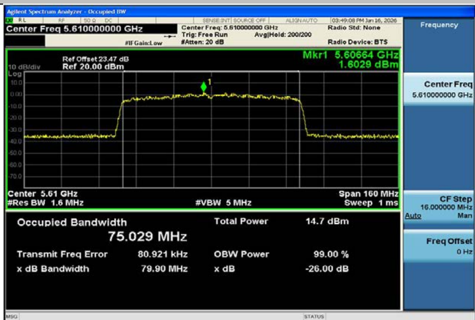
11AC80MIMO-Ant2-5610
