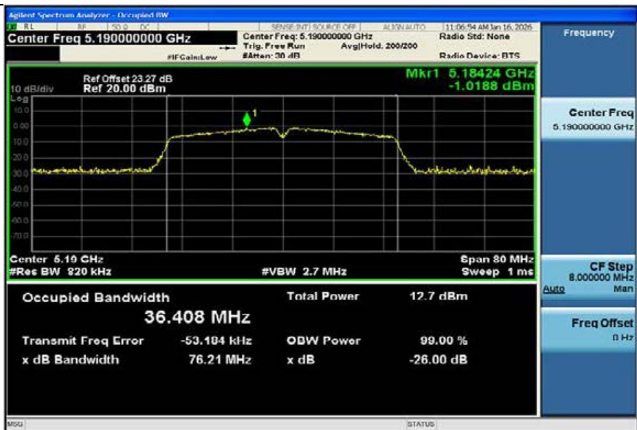
11AC40MIMO-Ant1-5190
