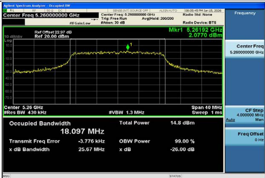
11AC20MIMO-Ant2-5260
