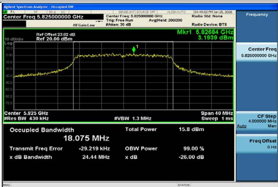
11N20MIMO-Ant2-5825
