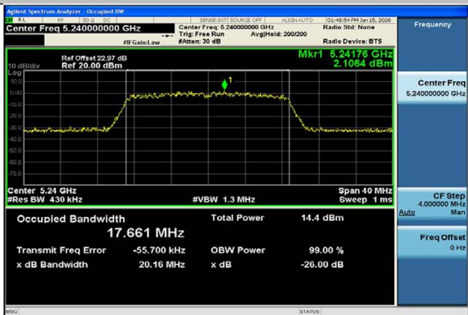
11N20MIMO-Ant2-5240
