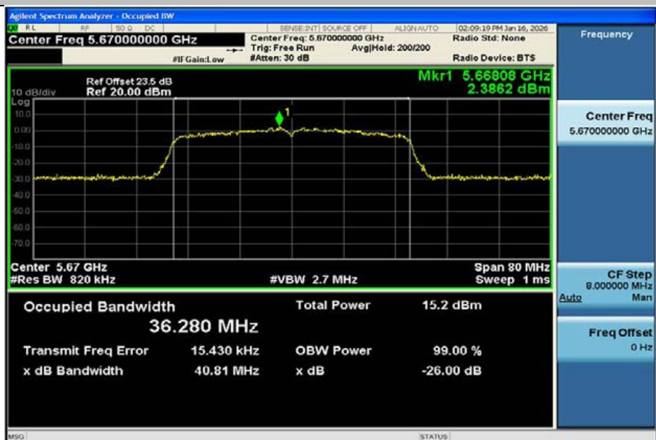
11AC40MIMO-Ant2-5670
